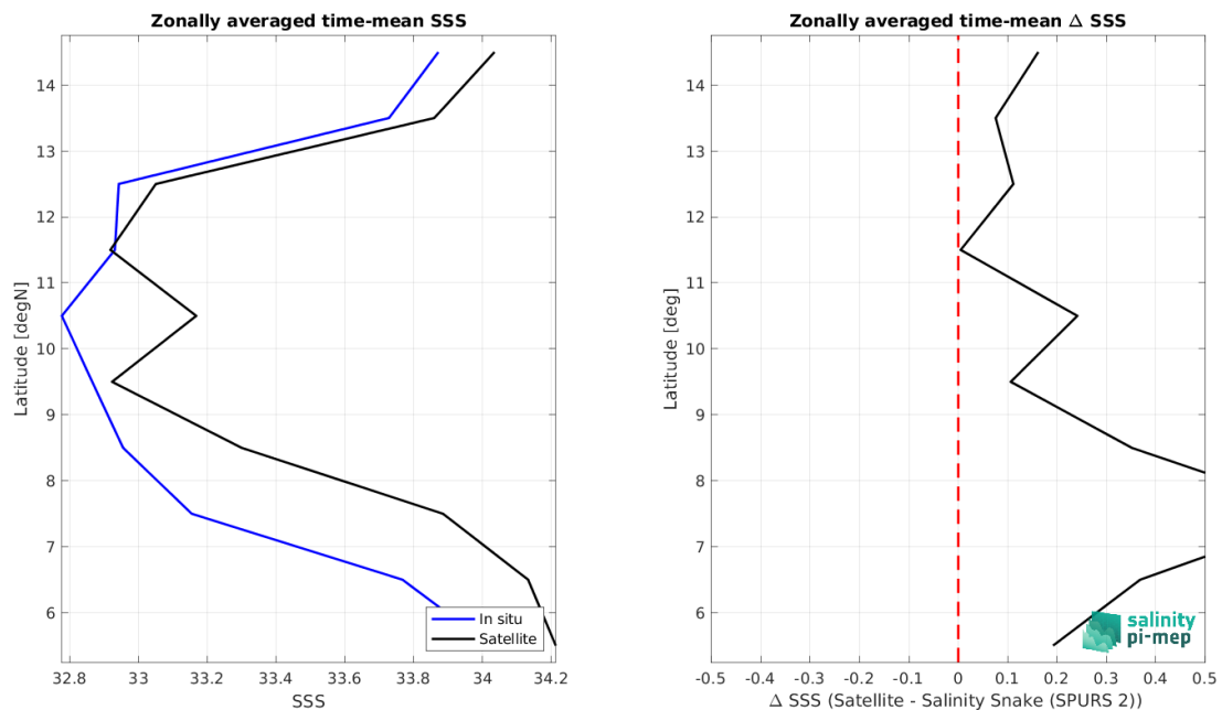
Figure 9: Left panel: Zonal mean SSS from SMOS SSS L3 v335 - Monthly - 25 km (CATDS-CPDC) satellite product (black) and from Salinity Snake (SPURS 2) (blue). Right panel: Zonal mean of \Delta SSS (Satellite - Salinity Snake (SPURS 2)) for all the collected Pi-MEP match-up pairs estimated over the full satellite product period.
