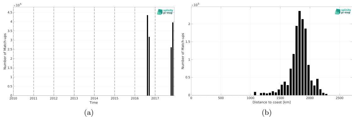
Figure 2: Number of match-ups between Salinity Snake (SPURS 2) and SMOS SSS L3 v335 - Monthly - 25 km (CATDS-CPDC) SSS as a function of time (a) and as function of the distance to coast (b) over the SPURS 2 Pi-MEP region and for the full satellite product period.
