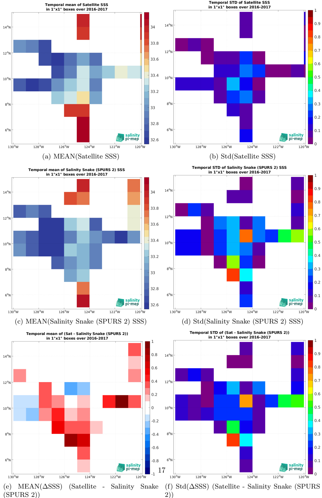
Figure 7: Temporal mean (left) and Std (right) of SSS from SMOS SSS L3 v335 - Monthly - 25 km (CATDS-CPDC) (top), Salinity Snake (SPURS 2) (middle), and of \Delta SSS (Satellite - Salinity Snake (SPURS 2)). Only match-up pairs are used to generate these maps.
