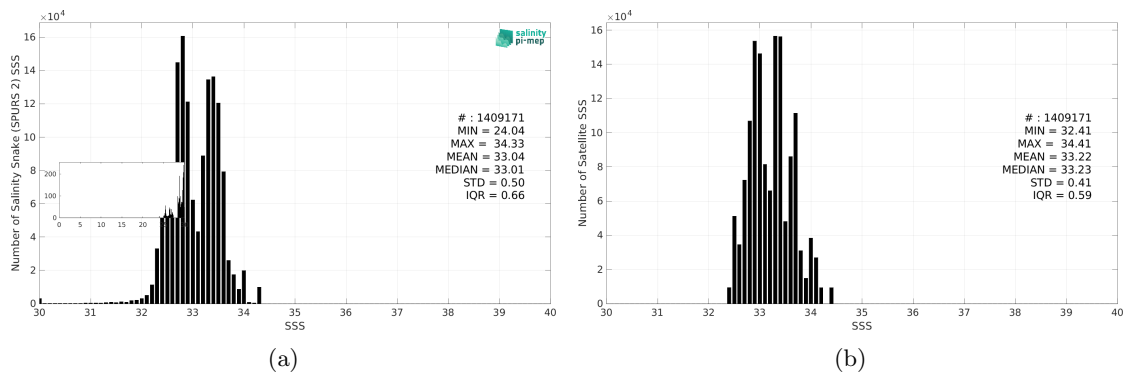
Figure 3: Histograms of SSS from Salinity Snake (SPURS 2) (a) and SMOS SSS L3 v335 - Monthly - 25 km (CATDS-CPDC) (b) considering all match-up pairs per bins of 0.1 over the SPURS 2 Pi-MEP region and for the full satellite product period.
