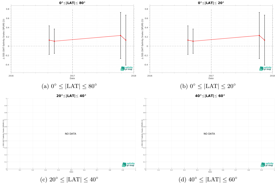
Figure 11: Monthly median (red curves) of \Delta SSS (Satellite - Salinity Snake (SPURS 2)) and \pm 1 Std (black vertical thick bars) as function of time for all the collected Pi-MEP match-up pairs estimated over the SPURS 2 Pi-MEP region and for the full satellite product period are shown for different latitude bands: (a) 80^\circ\text{S}-80^\circ\text{N} , (b) 20^\circ\text{S}-20^\circ\text{N} , (c) 40^\circ\text{S}-20^\circ\text{S} and 20^\circ\text{N}-40^\circ\text{N} and (d) 60^\circ\text{S}-40^\circ\text{S} and 40^\circ\text{N}-60^\circ\text{N} .
