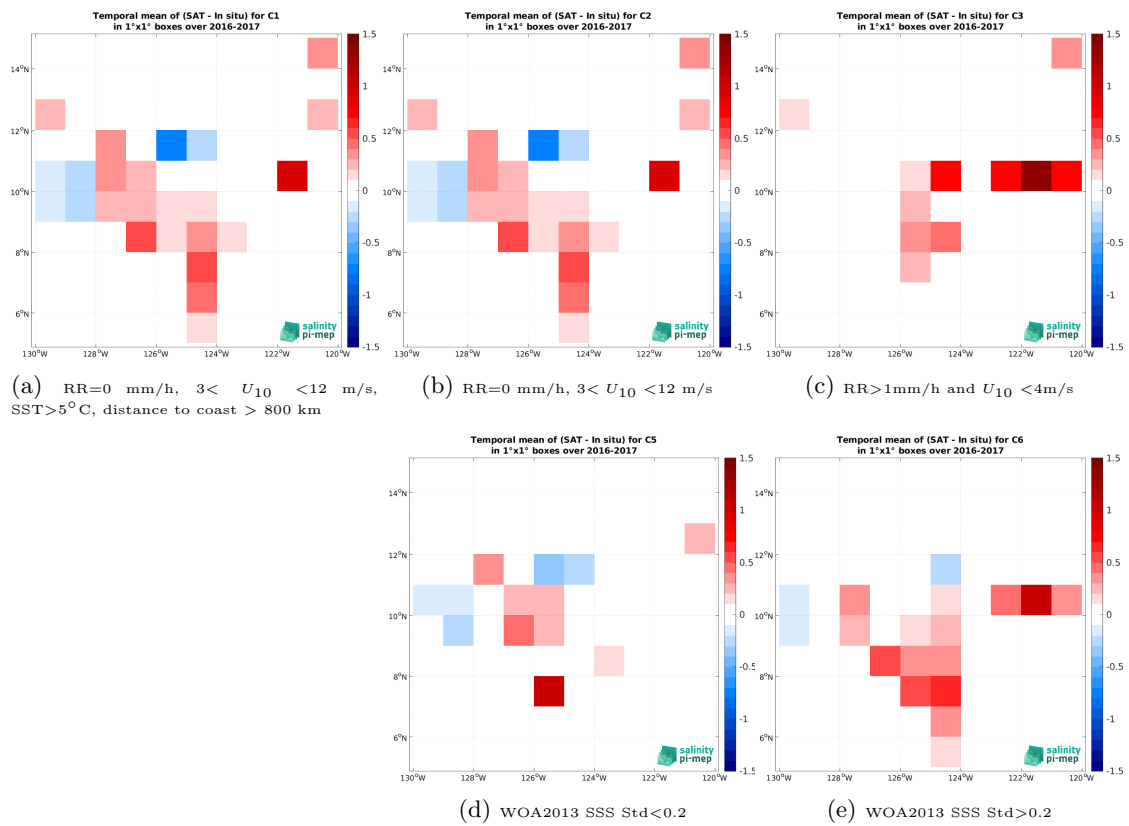
Figure 14: Temporal mean gridded over spatial boxes of size 1^\circ \times 1^\circ of \Delta\text{SSS} (SMOS SSS L3 v335 - Monthly - 25 km (CATDS-CPDC) - Salinity Snake (SPURS 2)) for 5 different subdatasets corresponding to: RR=0 mm/h, 3 < U_{10} < 12 m/s, SST > 5°C, distance to coast > 800 km (a), RR=0 mm/h, 3 < U_{10} < 12 m/s (b), RR > 1mm/h and U_{10} < 4 m/s (c), WOA2013 SSS Std < 0.2 (d), WOA2013 SSS Std > 0.2 (e).
