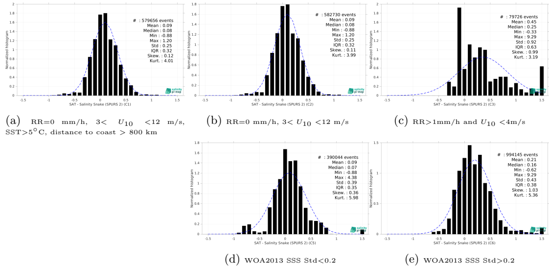
Figure 15: Normalized histogram of \Delta\text{SSS} (SMOS SSS L3 v335 - Monthly - 25 km (CATDS-CPDC) - Salinity Snake (SPURS 2)) for 5 different subdatasets corresponding to: RR=0 mm/h, 3 < U_{10} < 12 m/s, SST>5°C, distance to coast > 800 km (a), RR=0 mm/h, 3 < U_{10} < 12 m/s (b), RR>1mm/h and U_{10} < 4 m/s (c), WOA2013 SSS Std<0.2 (d), WOA2013 SSS Std>0.2 (e).
