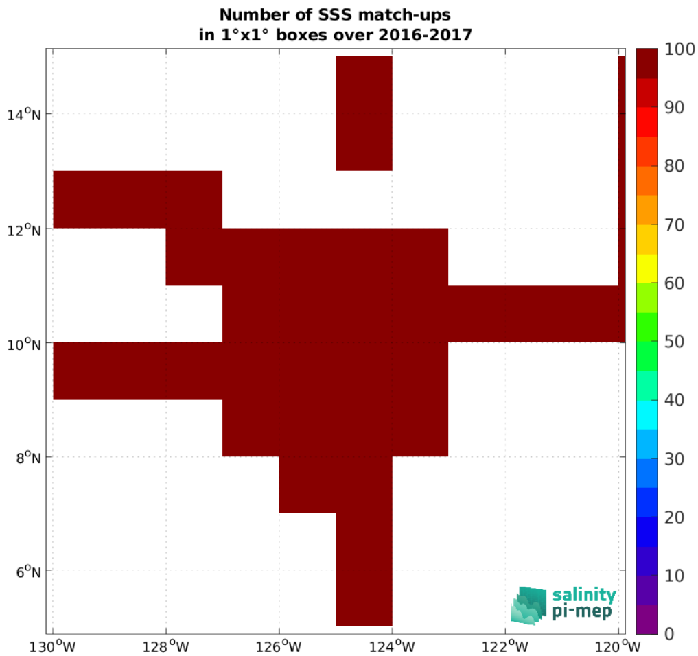
Figure 5: Number of SSS match-ups between Salinity Snake (SPURS 2) SSS and the SMOS SSS L3 v335 - Monthly - 25 km (CATDS-CPDC) SSS product for the SPURS 2 Pi-MEP region over 1^\circ \times 1^\circ boxes and for the full satellite product period.
