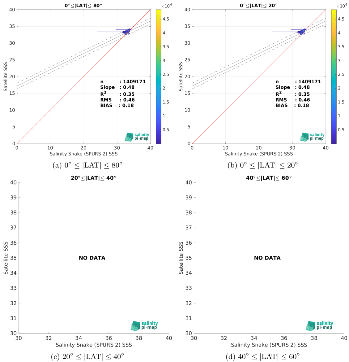
Figure 10: Contour maps of the concentration of SMOS SSS L3 v335 - Monthly - 25 km (CATDS-CPDC) SSS (y-axis) versus Salinity Snake (SPURS 2) SSS (x-axis) at match-up pairs for different latitude bands. For each plot, the red line shows x=y . The black thin and dashed lines indicate a linear fit through the data cloud and the \pm 95\% confidence levels, respectively. The number match-up pairs n , the slope and R^2 coefficient of the linear fit, the root mean square (RMS) and the mean bias between satellite and in situ data are indicated for each latitude band in each plots.
