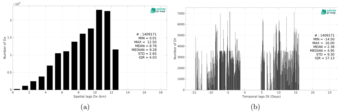
Figure 6: Histograms of the spatial (a) and temporal (b) lags between the location/time of the Salinity Snake (SPURS 2) measurement and the date of the corresponding SMOS SSS L3 v335 - Monthly - 25 km (CATDS-CPDC) SSS pixel.
