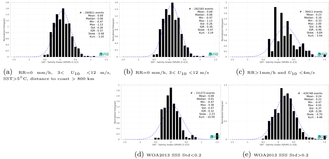
Figure 15: Normalized histogram of \Delta SSS (SMOS SSS L3 v335 - Monthly - 25 km (CATDS-CPDC) - Salinity Snake (SPURS 2)) for 5 different subdatasets corresponding to: RR=0 mm/h, 3 < U_{10} < 12 m/s, SST>5°C, distance to coast > 800 km (a), RR=0 mm/h, 3 < U_{10} < 12 m/s (b), RR>1mm/h and U_{10} < 4 m/s (c), WOA2013 SSS Std<0.2 (d), WOA2013 SSS Std>0.2 (e).
