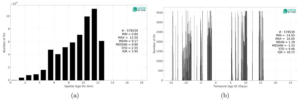
Figure 5: Histograms of the spatial (a) and temporal (b) lags between the location/time of the Salinity Snake (SPURS 2) measurement and the date of the corresponding SMOS SSS L3 v335 - Monthly - 25 km (CATDS-CPDC) SSS pixel.
