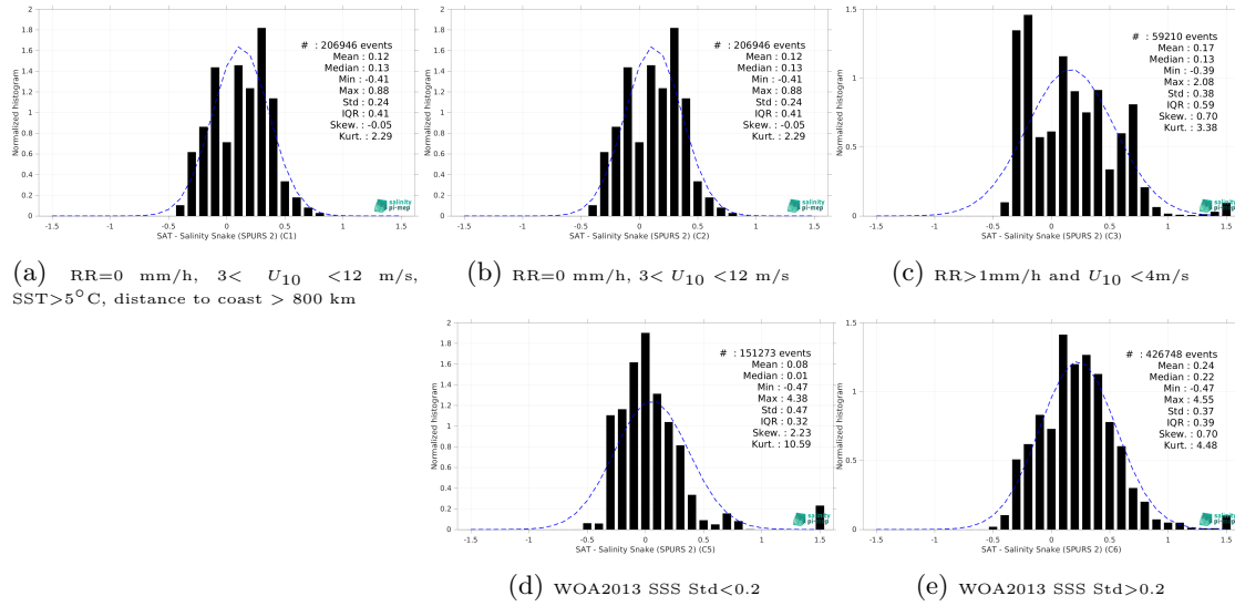
Figure 13: Normalized histogram of \Delta SSS (SMOS SSS L3 v335 - Monthly - 25 km (CATDS-CPDC) - Salinity Snake (SPURS 2)) for 5 different subdatasets corresponding to: RR=0 mm/h, 3 < U_{10} < 12 m/s, SST>5°C, distance to coast > 800 km (a), RR=0 mm/h, 3 < U_{10} < 12 m/s (b), RR>1mm/h and U_{10} < 4 m/s (c), WOA2013 SSS Std<0.2 (d), WOA2013 SSS Std>0.2 (e).
