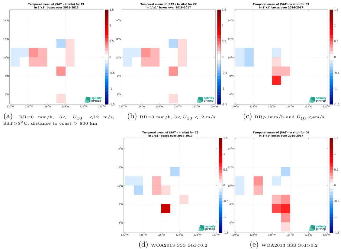
Figure 12: Temporal mean gridded over spatial boxes of size 1^\circ \times 1^\circ of \Delta SSS (SMOS SSS L3 v335 - Monthly - 25 km (CATDS-CPDC) - Salinity Snake (SPURS 2)) for 5 different subdatasets corresponding to:RR=0 mm/h, 3 < U_{10} < 12 m/s, SST>5°C, distance to coast > 800 km (a), RR=0 mm/h, 3 < U_{10} < 12 m/s (b), RR>1mm/h and U_{10} < 4 m/s (c), WOA2013 SSS Std<0.2 (d), WOA2013 SSS Std>0.2 (e).
