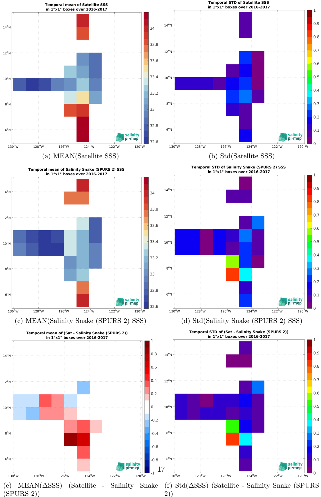
Figure 6: Temporal mean (left) and Std (right) of SSS from SMOS SSS L3 v335 - Monthly - 25 km (CATDS-CPDC) (top), Salinity Snake (SPURS 2) (middle), and of \Delta SSS (Satellite - Salinity Snake (SPURS 2)). Only match-up pairs are used to generate these maps.
