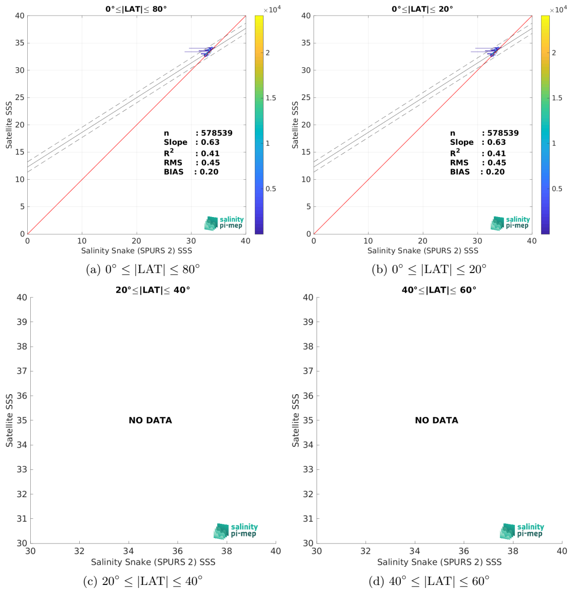
Figure 9: Contour maps of the concentration of SMOS SSS L3 v335 - Monthly - 25 km (CATDS-CPDC) SSS (y-axis) versus Salinity Snake (SPURS 2) SSS (x-axis) at match-up pairs for different latitude bands. For each plot, the red line shows x=y . The black thin and dashed lines indicate a linear fit through the data cloud and the \pm 95\% confidence levels, respectively. The number match-up pairs n , the slope and R^2 coefficient of the linear fit, the root mean square (RMS) and the mean bias between satellite and in situ data are indicated for each latitude band in each plots.
