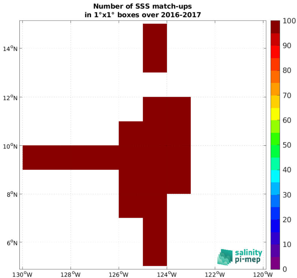
Figure 4: Number of SSS match-ups between Salinity Snake (SPURS 2) SSS and the SMOS SSS L3 v335 - Monthly - 25 km (CATDS-CPDC) SSS product for the SPURS 2 Pi-MEP region over 1^\circ \times 1^\circ boxes and for the full satellite product period.
