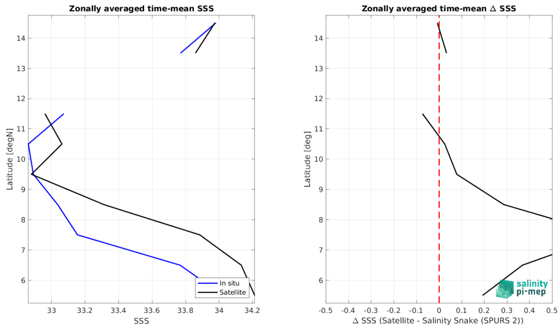
Figure 8: Left panel: Zonal mean SSS from SMOS SSS L3 v335 - Monthly - 25 km (CATDS-CPDC) satellite product (black) and from Salinity Snake (SPURS 2) (blue). Right panel: Zonal mean of \Delta SSS (Satellite - Salinity Snake (SPURS 2)) for all the collected Pi-MEP match-up pairs estimated over the full satellite product period.
