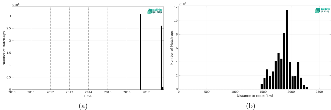
Figure 1: Number of match-ups between Salinity Snake (SPURS 2) and SMOS SSS L3 v335 - Monthly - 25 km (CATDS-CPDC) SSS as a function of time (a) and as function of the distance to coast (b) over the SPURS 2 Pi-MEP region and for the full satellite product period.
