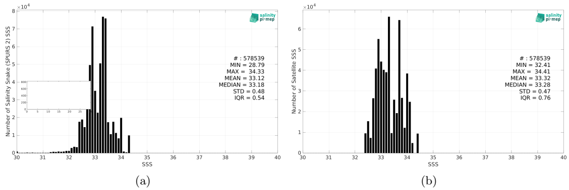
Figure 2: Histograms of SSS from Salinity Snake (SPURS 2) (a) and SMOS SSS L3 v335 - Monthly - 25 km (CATDS-CPDC) (b) considering all match-up pairs per bins of 0.1 over the SPURS 2 Pi-MEP region and for the full satellite product period.
