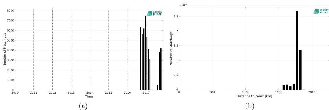
Figure 2: Number of match-ups between Seaglider (SPURS 2) and SMOS SSS L3 v335 - Monthly - 25 km (CATDS-CPDC) SSS as a function of time (a) and as function of the distance to coast (b) over the SPURS 2 Pi-MEP region and for the full satellite product period.
