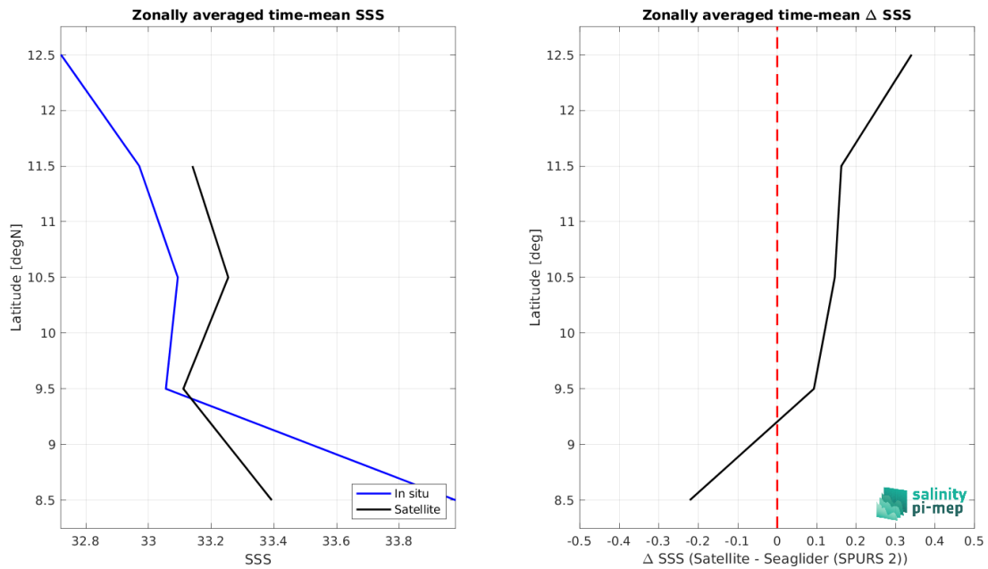
Figure 9: Left panel: Zonal mean SSS from SMOS SSS L3 v335 - Monthly - 25 km (CATDS-CPDC) satellite product (black) and from Seaglider (SPURS 2) (blue). Right panel: Zonal mean of \Delta SSS (Satellite - Seaglider (SPURS 2)) for all the collected Pi-MEP match-up pairs estimated over the full satellite product period.
