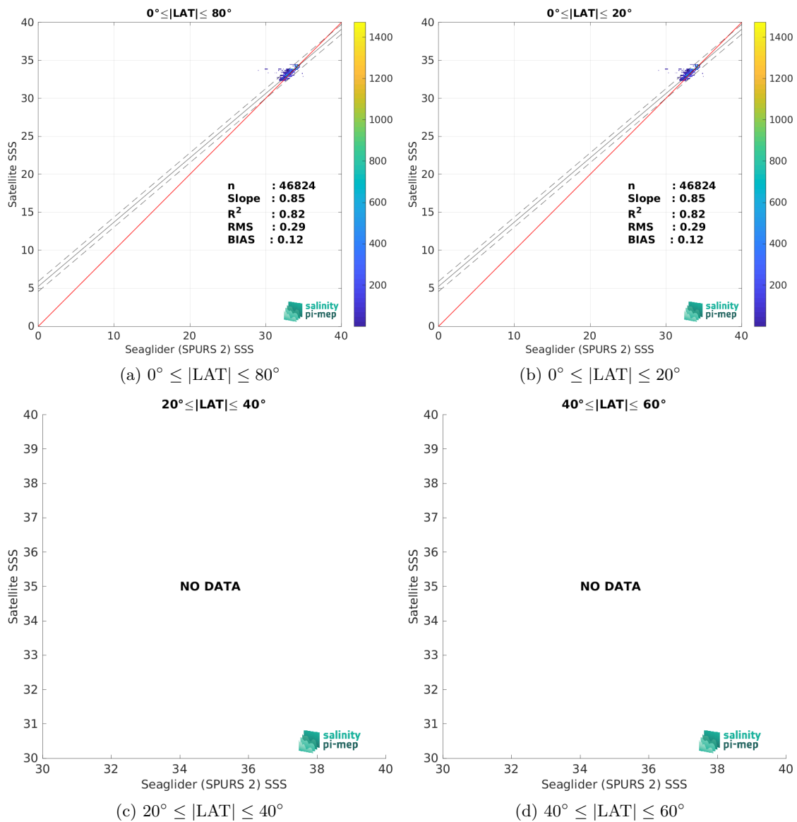
Figure 10: Contour maps of the concentration of SMOS SSS L3 v335 - Monthly - 25 km (CATDS-CPDC) SSS (y-axis) versus Seaglider (SPURS 2) SSS (x-axis) at match-up pairs for different latitude bands. For each plot, the red line shows x=y . The black thin and dashed lines indicate a linear fit through the data cloud and the \pm 95\% confidence levels, respectively. The number match-up pairs n , the slope and R^2 coefficient of the linear fit, the root mean square (RMS) and the mean bias between satellite and in situ data are indicated for each latitude band in each plots.
