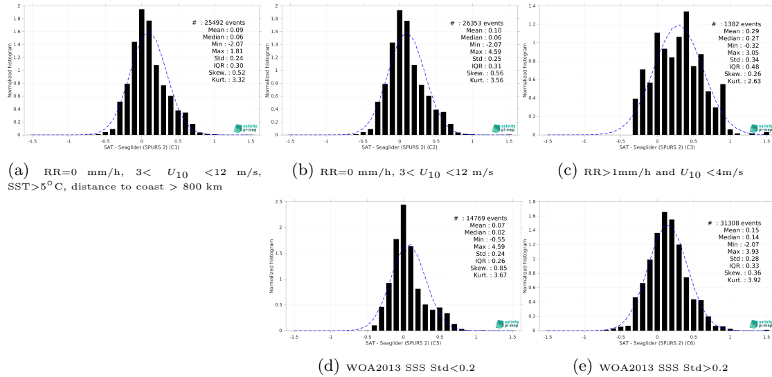
Figure 15: Normalized histogram of \Delta SSS (SMOS SSS L3 v335 - Monthly - 25 km (CATDS-CPDC) - Seaglider (SPURS 2)) for 5 different subdatasets corresponding to: RR=0 mm/h, 3 < U_{10} < 12 m/s, SST>5°C, distance to coast > 800 km (a), RR=0 mm/h, 3 < U_{10} < 12 m/s (b), RR>1mm/h and U_{10} < 4 m/s (c), WOA2013 SSS Std<0.2 (d), WOA2013 SSS Std>0.2 (e).
