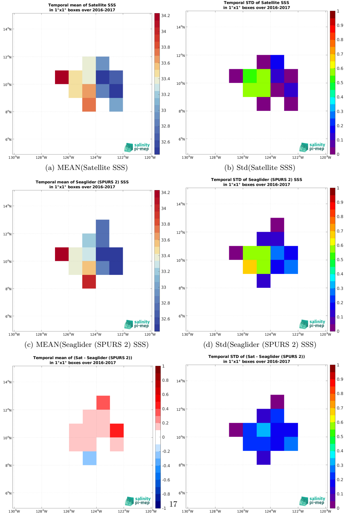
Figure 7: Temporal mean (left) and Std (right) of SSS from SMOS SSS L3 v335 - Monthly - 25 km (CATDS-CPDC) (top), Seaglider (SPURS 2) (middle), and of \Delta SSS (Satellite - Seaglider (SPURS 2)). Only match-up pairs are used to generate these maps.
