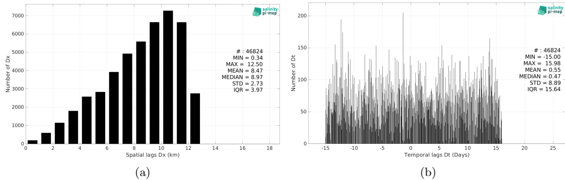
Figure 6: Histograms of the spatial (a) and temporal (b) lags between the location/time of the Seaglider (SPURS 2) measurement and the date of the corresponding SMOS SSS L3 v335 - Monthly - 25 km (CATDS-CPDC) SSS pixel.
