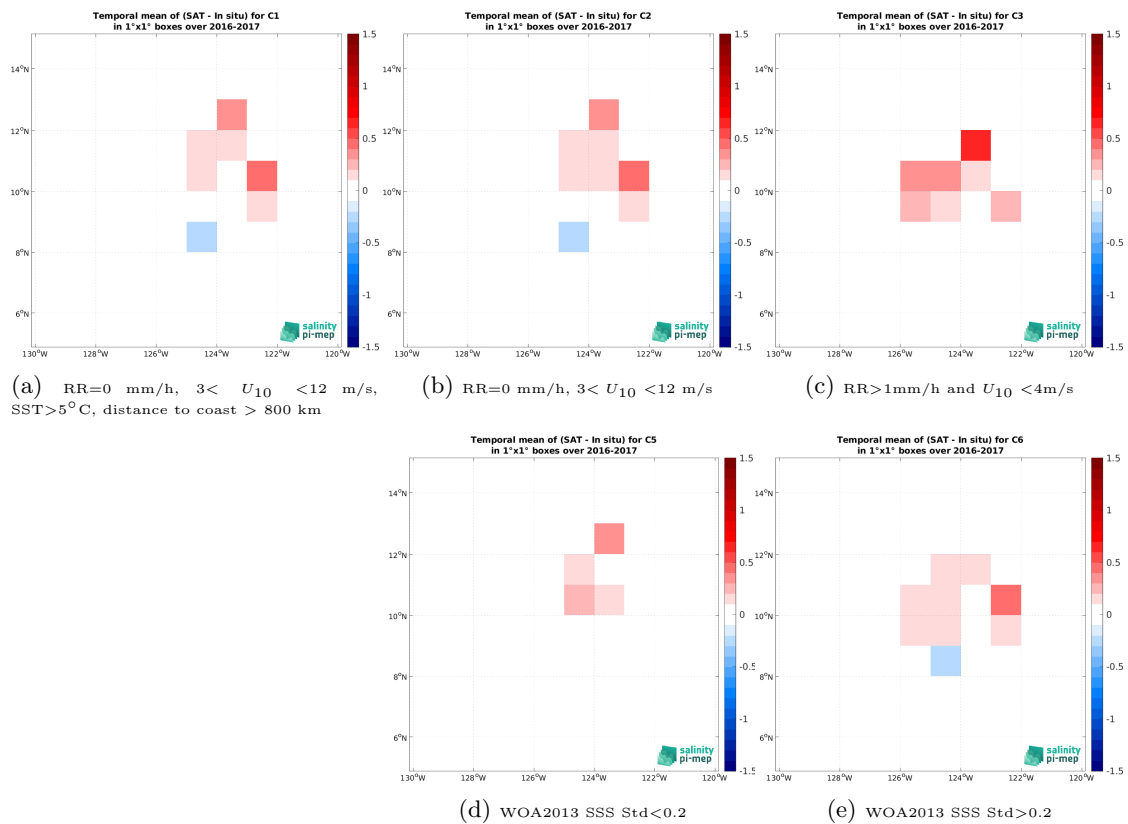
Figure 14: Temporal mean gridded over spatial boxes of size 1^\circ \times 1^\circ of \Delta SSS (SMOS SSS L3 v335 - Monthly - 25 km (CATDS-CPDC) - Seaglider (SPURS 2)) for 5 different subdatasets corresponding to:RR=0 mm/h, 3 < U_{10} < 12 m/s, SST >5^\circ C, distance to coast > 800 km (a), RR=0 mm/h, 3 < U_{10} < 12 m/s (b), RR >1 mm/h and U_{10} < 4 m/s (c), WOA2013 SSS Std <0.2 (d), WOA2013 SSS Std >0.2 (e).
