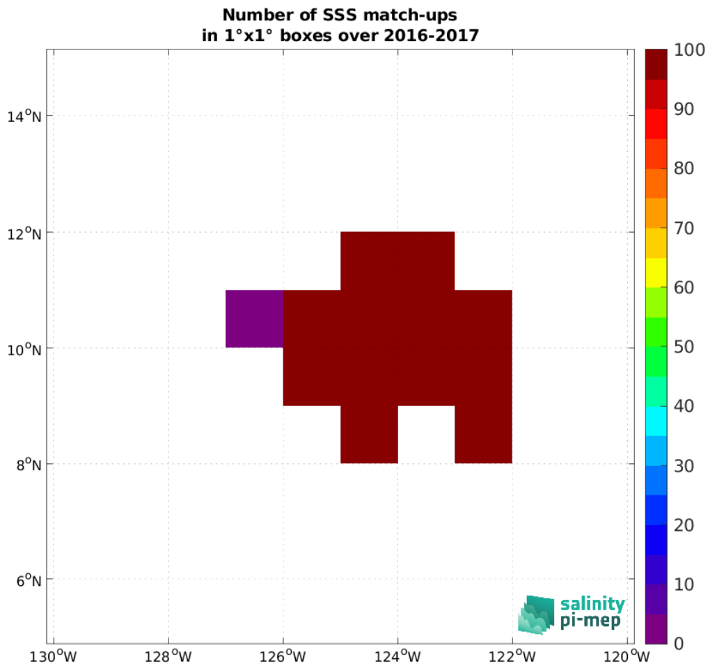
Figure 5: Number of SSS match-ups between Seaglider (SPURS 2) SSS and the SMOS SSS L3 v335 - Monthly - 25 km (CATDS-CPDC) SSS product for the SPURS 2 Pi-MEP region over 1^\circ \times 1^\circ boxes and for the full satellite product period.
