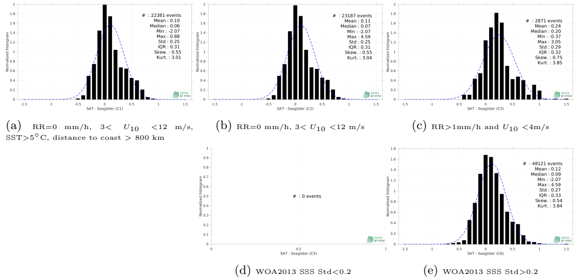
Figure 13: Normalized histogram of \Delta SSS (SMOS SSS L3 v335 - Monthly - 25 km (CATDS-CPDC) - Seaglider) for 5 different subdatasets corresponding to: RR=0 mm/h, 3 < U_{10} < 12 m/s, SST > 5°C, distance to coast > 800 km (a), RR=0 mm/h, 3 < U_{10} < 12 m/s (b), RR > 1mm/h and U_{10} < 4 m/s (c), WOA2013 SSS Std < 0.2 (d), WOA2013 SSS Std > 0.2 (e).
