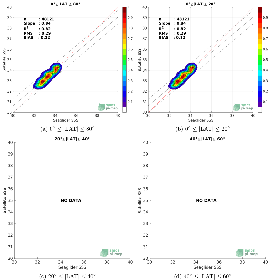
Figure 9: Contour maps of the concentration of SMOS SSS L3 v335 - Monthly - 25 km (CATDS-CPDC) SSS (y-axis) versus Seaglider SSS (x-axis) at match-up pairs for different latitude bands. For each plot, the red line shows x=y . The black thin and dashed lines indicate a linear fit through the data cloud and the \pm 95\% confidence levels, respectively. The number match-up pairs n , the slope and R^2 coefficient of the linear fit, the root mean square (RMS) and the mean bias between satellite and in situ data are indicated for each latitude band in each plots.
