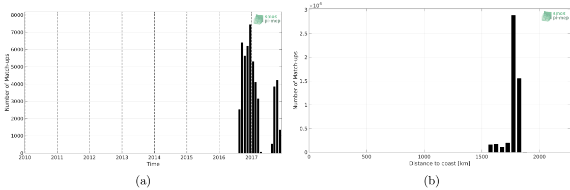
Figure 1: Number of match-ups between Seaglider and SMOS SSS L3 v335 - Monthly - 25 km (CATDS-CPDC) SSS as a function of time (a) and as function of the distance to coast (b) over the SPURS 2 Pi-MEP region and for the full satellite product period.
