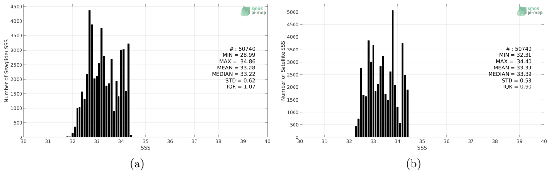
Figure 2: Histograms of SSS from Seaglider (a) and SMOS SSS L3 v335 - Monthly - 25 km (CATDS-CPDC) (b) considering all match-up pairs per bins of 0.1 over the SPURS 2 Pi-MEP region and for the full satellite product period.
