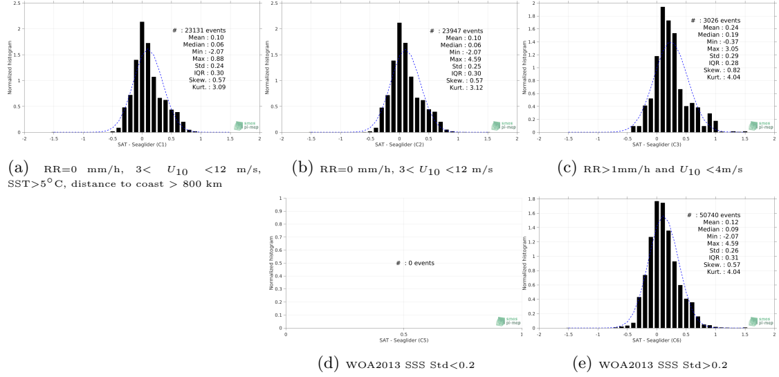
Figure 12: Normalized histogram of \Delta SSS (SMOS SSS L3 v335 - Monthly - 25 km (CATDS-CPDC) - Seaglider) for 5 different subdatasets corresponding to: RR=0 mm/h, 3 < U_{10} < 12 m/s, SST>5°C, distance to coast > 800 km (a), RR=0 mm/h, 3 < U_{10} < 12 m/s (b), RR>1mm/h and U_{10} < 4 m/s (c), WOA2013 SSS Std<0.2 (d), WOA2013 SSS Std>0.2 (e).
