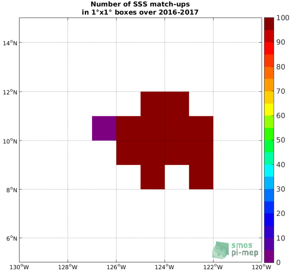
Figure 3: Number of SSS match-ups between Seaglider SSS and the SMOS SSS L3 v335 - Monthly - 25 km (CATDS-CPDC) SSS product for the SPURS 2 Pi-MEP region over 1^\circ \times 1^\circ boxes and for the full satellite product period.
