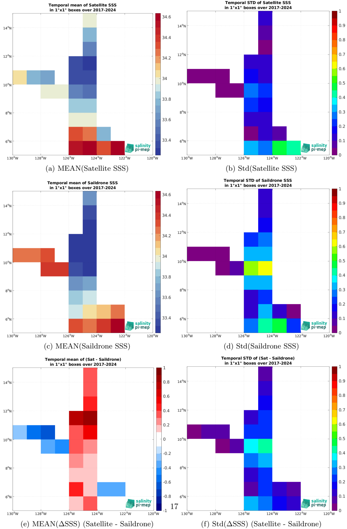
Figure 7: Temporal mean (left) and Std (right) of SSS from SMOS SSS L3 v335 - Monthly - 25 km (CATDS-CPDC) (top), Saildrone (middle), and of \Delta SSS (Satellite - Saildrone). Only match-up pairs are used to generate these maps.
