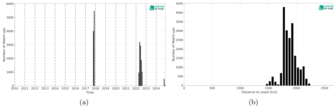
Figure 2: Number of match-ups between Saildrone and SMOS SSS L3 v335 - Monthly - 25 km (CATDS-CPDC) SSS as a function of time (a) and as function of the distance to coast (b) over the SPURS 2 Pi-MEP region and for the full satellite product period.
