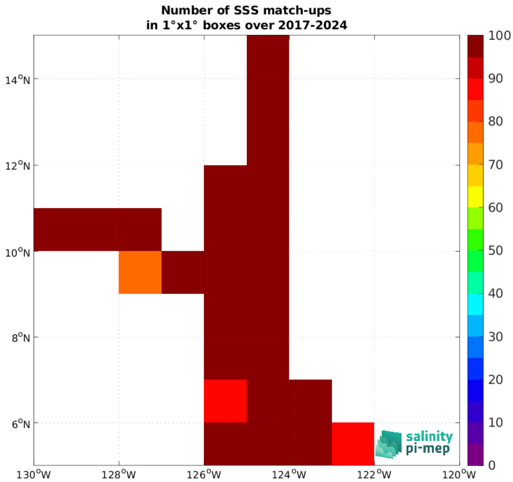
Figure 5: Number of SSS match-ups between Saildrone SSS and the SMOS SSS L3 v335 - Monthly - 25 km (CATDS-CPDC) SSS product for the SPURS 2 Pi-MEP region over 1°x1° boxes and for the full satellite product period.
