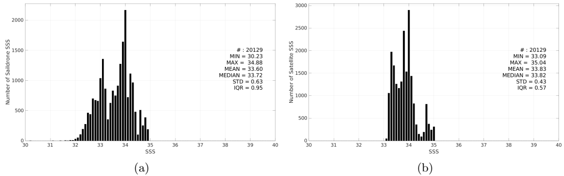
Figure 3: Histograms of SSS from Sairdrona (a) and SMOS SSS L3 v335 - Monthly - 25 km (CATDS-CPDC) (b) considering all match-up pairs per bins of 0.1 over the SPURS 2 Pi-MEP region and for the full satellite product period.
