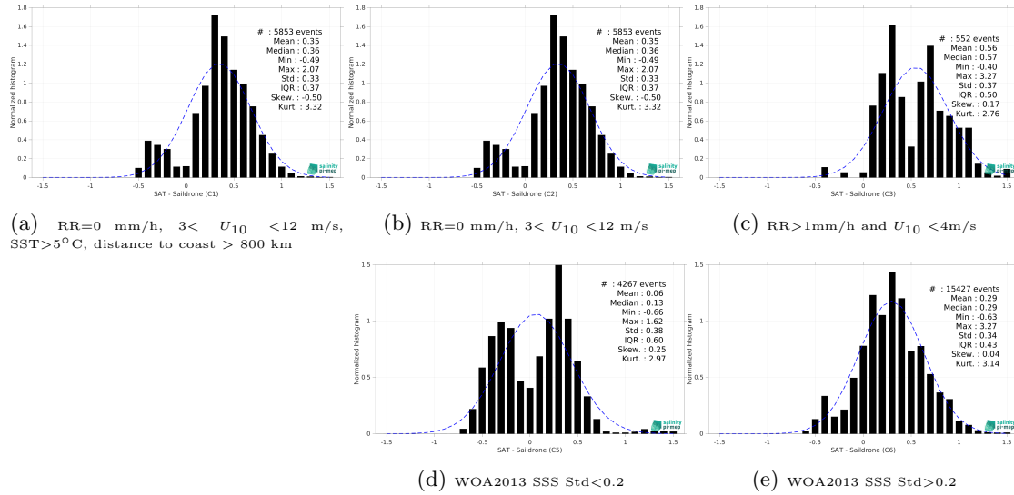
Figure 15: Normalized histogram of \Delta SSS (SMOS SSS L3 v335 - Monthly - 25 km (CATDS-CPDC) - Sairdrone) for 5 different subdatasets corresponding to: RR=0 mm/h, 3 < U_{10} < 12 m/s, SST>5°C, distance to coast > 800 km (a), RR=0 mm/h, 3 < U_{10} < 12 m/s (b), RR>1mm/h and U_{10} < 4 m/s (c), WOA2013 SSS Std<0.2 (d), WOA2013 SSS Std>0.2 (e).
