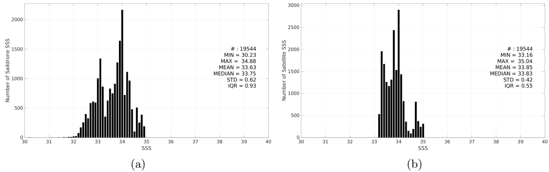
Figure 3: Histograms of SSS from Saildrone (a) and SMOS SSS L3 v335 - Monthly - 25 km (CATDS-CPDC) (b) considering all match-up pairs per bins of 0.1 over the SPURS 2 Pi-MEP region and for the full satellite product period.
