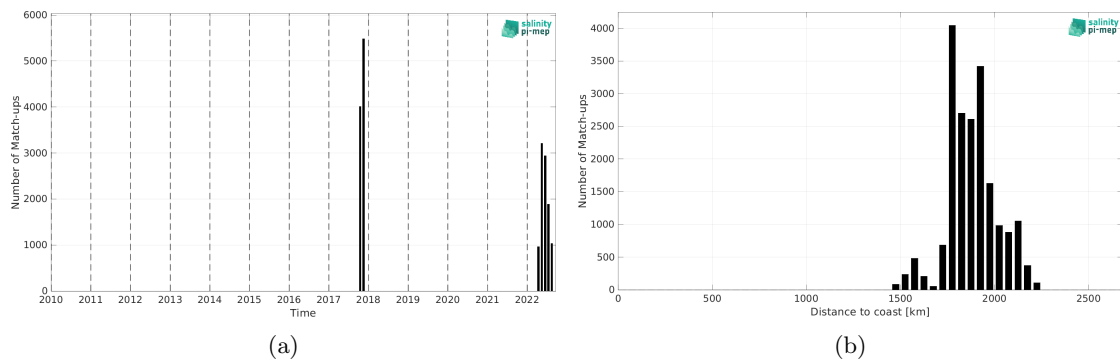
Figure 2: Number of match-ups between Sailability and SMOS SSS L3 v335 - Monthly - 25 km (CATDS-CPDC) SSS as a function of time (a) and as function of the distance to coast (b) over the SPURS 2 Pi-MEP region and for the full satellite product period.
