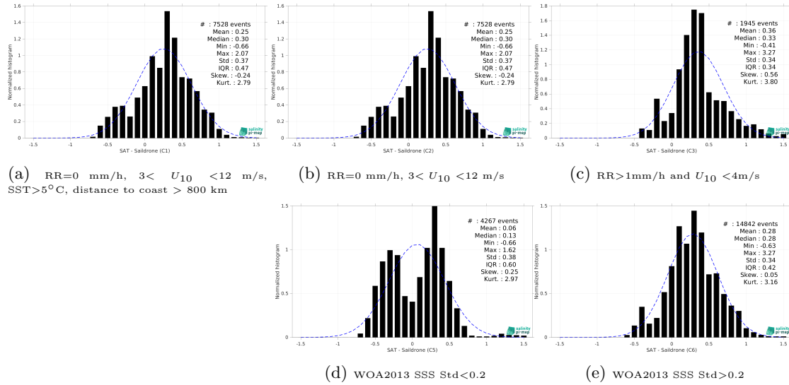
Figure 13: Normalized histogram of \Delta SSS (SMOS SSS L3 v335 - Monthly - 25 km (CATDS-CPDC) - Sailsdrone) for 5 different subdatasets corresponding to: RR=0 mm/h, 3 < U_{10} < 12 m/s, SST>5°C, distance to coast > 800 km (a), RR=0 mm/h, 3 < U_{10} < 12 m/s (b), RR>1mm/h and U_{10} < 4 m/s (c), WOA2013 SSS Std<0.2 (d), WOA2013 SSS Std>0.2 (e).
