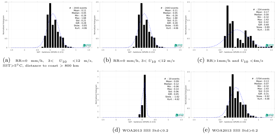
Figure 15: Normalized histogram of \Delta SSS (SMOS SSS L3 v335 - Monthly - 25 km (CATDS-CPDC) - Saïdrone (SPURS 2)) for 5 different subdatasets corresponding to: RR=0 mm/h, 3 < U_{10} < 12 m/s, SST > 5°C, distance to coast > 800 km (a), RR=0 mm/h, 3 < U_{10} < 12 m/s (b), RR > 1mm/h and U_{10} < 4 m/s (c), WOA2013 SSS Std < 0.2 (d), WOA2013 SSS Std > 0.2 (e).
