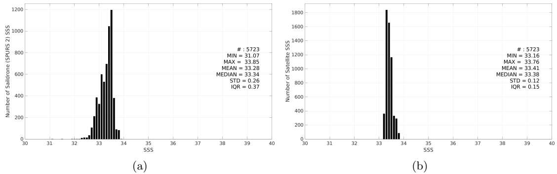
Figure 3: Histograms of SSS from Saildrone (SPURS 2) (a) and SMOS SSS L3 v335 - Monthly - 25 km (CATDS-CPDC) (b) considering all match-up pairs per bins of 0.1 over the SPURS 2 Pi-MEP region and for the full satellite product period.
