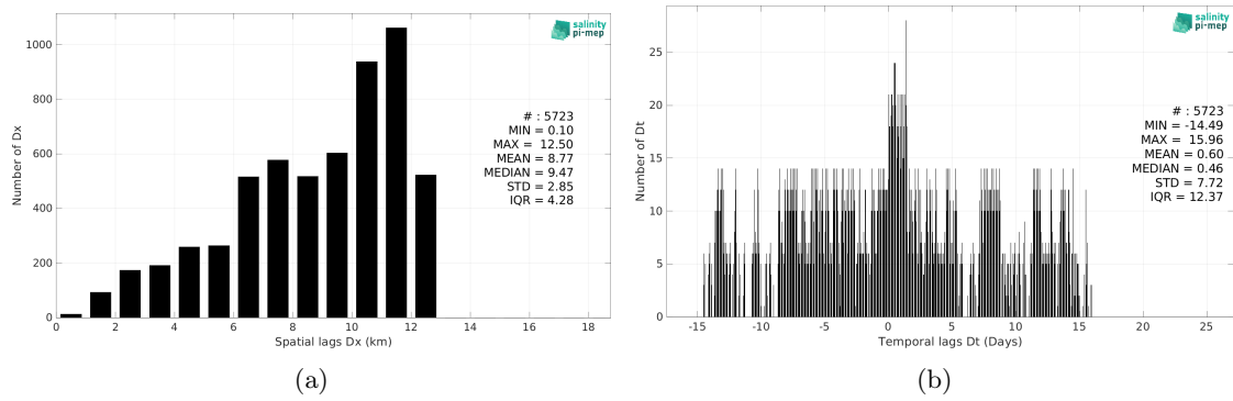
Figure 6: Histograms of the spatial (a) and temporal (b) lags between the location/time of the Saildrone (SPURS 2) measurement and the date of the corresponding SMOS SSS L3 v335 - Monthly - 25 km (CATDS-CPDC) SSS pixel.
