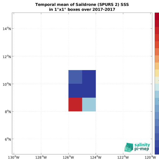
(c) MEAN(Saildrone (SPURS 2) SSS)
