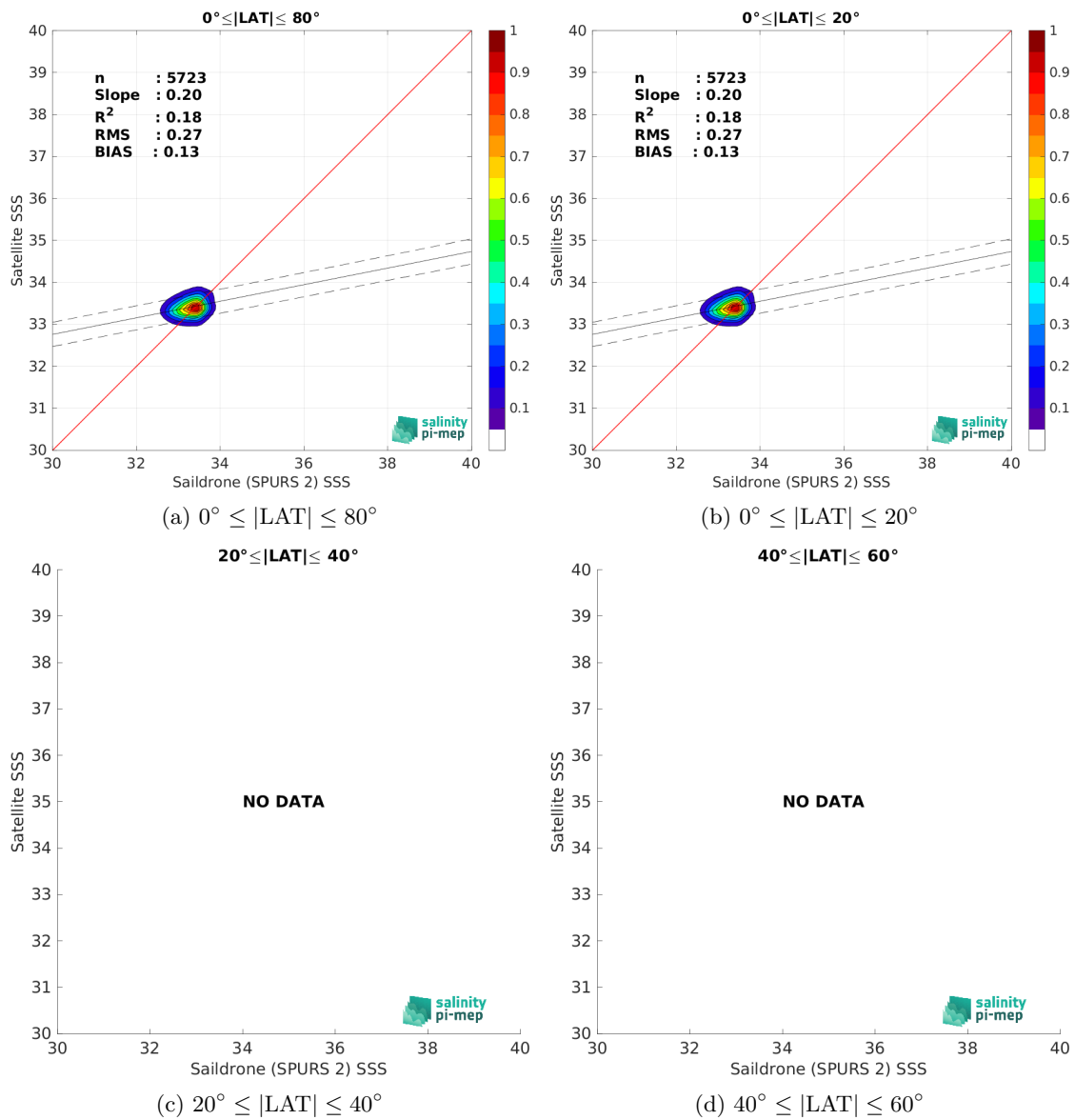
Figure 10: Contour maps of the concentration of SMOS SSS L3 v335 - Monthly - 25 km (CATDS-CPDC) SSS (y-axis) versus Saildrone (SPURS 2) SSS (x-axis) at match-up pairs for different latitude bands. For each plot, the red line shows x=y . The black thin and dashed lines indicate a linear fit through the data cloud and the \pm 95\% confidence levels, respectively. The number match-up pairs n , the slope and R^2 coefficient of the linear fit, the root mean square (RMS) and the mean bias between satellite and in situ data are indicated for each latitude band in each plots.
