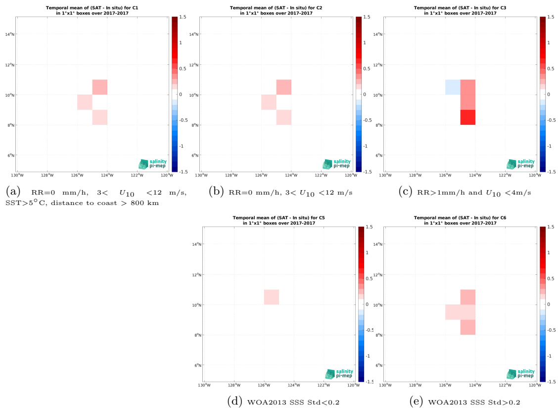
Figure 14: Temporal mean gridded over spatial boxes of size 1^\circ \times 1^\circ of \Delta SSS (SMOS SSS L3 v335 - Monthly - 25 km (CATDS-CPDC) - Saildrone (SPURS 2)) for 5 different subdatasets corresponding to:RR=0 mm/h, 3 < U_{10} < 12 m/s, SST >5^\circ C, distance to coast > 800 km (a), RR=0 mm/h, 3 < U_{10} < 12 m/s (b), RR >1 mm/h and U_{10} < 4 m/s (c), WOA2013 SSS Std <0.2 (d), WOA2013 SSS Std >0.2 (e).
