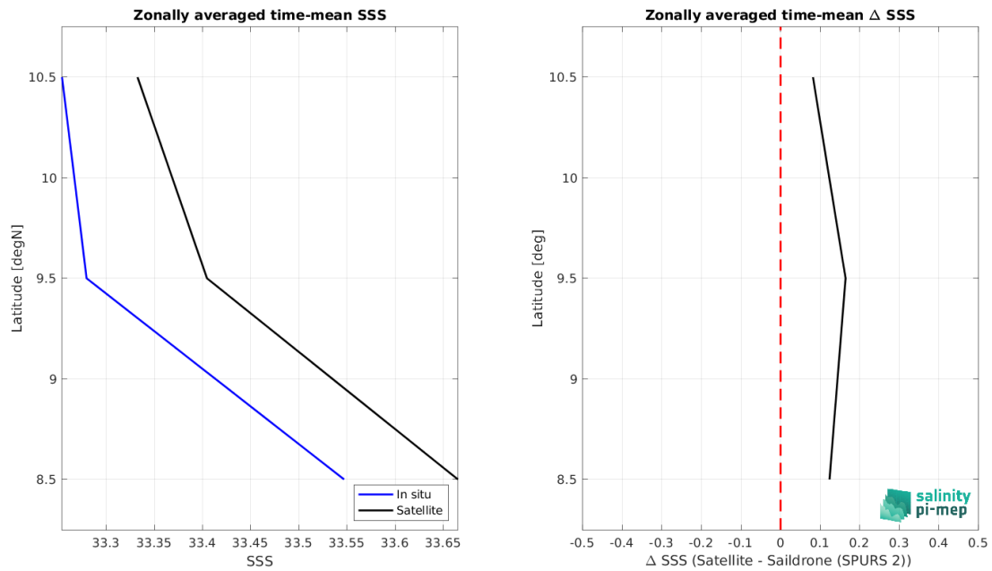
Figure 9: Left panel: Zonal mean SSS from SMOS SSS L3 v335 - Monthly - 25 km (CATDS-CPDC) satellite product (black) and from Sairdron (SPURS 2) (blue). Right panel: Zonal mean of \Delta SSS (Satellite - Sairdron (SPURS 2)) for all the collected Pi-MEP match-up pairs estimated over the full satellite product period.
