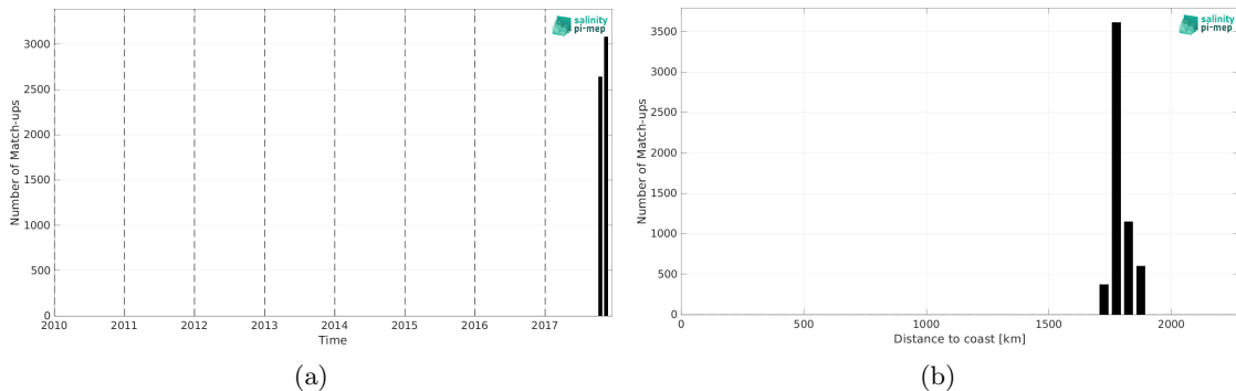
Figure 2: Number of match-ups between Saildrone (SPURS 2) and SMOS SSS L3 v335 - Monthly - 25 km (CATDS-CPDC) SSS as a function of time (a) and as function of the distance to coast (b) over the SPURS 2 Pi-MEP region and for the full satellite product period.
