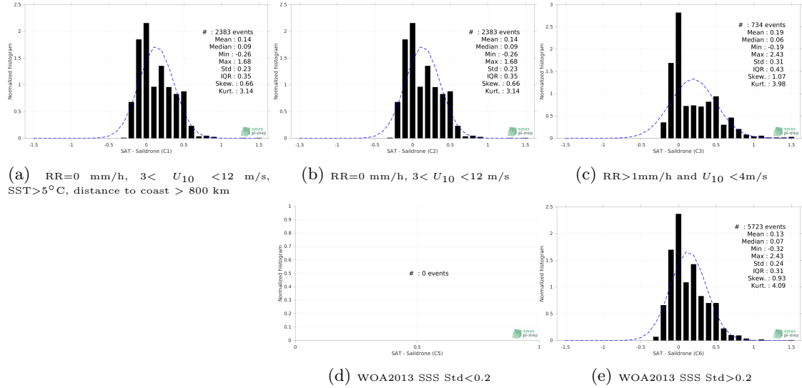
Figure 12: Normalized histogram of \Delta SSS (SMOS SSS L3 v335 - Monthly - 25 km (CATDS-CPDC) - Saildrone) for 5 different subdatasets corresponding to: RR=0 mm/h, 3 < U_{10} < 12 m/s, SST > 5°C, distance to coast > 800 km (a), RR=0 mm/h, 3 < U_{10} < 12 m/s (b), RR > 1mm/h and U_{10} < 4 m/s (c), WOA2013 SSS Std < 0.2 (d), WOA2013 SSS Std > 0.2 (e).
