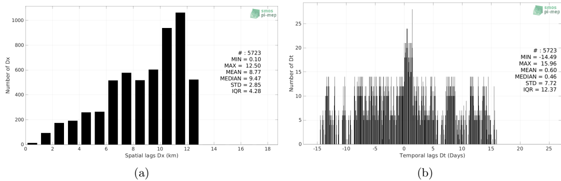
Figure 4: Histograms of the spatial (a) and temporal (b) lags between the location/time of the Saildrone measurement and the date of the corresponding SMOS SSS L3 v335 - Monthly - 25 km (CATDS-CPDC) SSS pixel.
