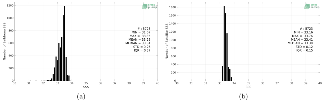
Figure 2: Histograms of SSS from Sairdrone (a) and SMOS SSS L3 v335 - Monthly - 25 km (CATDS-CPDC) (b) considering all match-up pairs per bins of 0.1 over the SPURS 2 Pi-MEP region and for the full satellite product period.
