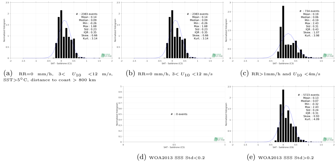
Figure 12: Normalized histogram of \Delta SSS (SMOS SSS L3 v335 - Monthly - 25 km (CATDS-CPDC) - Sairdrone) for 5 different subdatasets corresponding to: RR=0 mm/h, 3 < U_{10} < 12 m/s, SST > 5°C, distance to coast > 800 km (a), RR=0 mm/h, 3 < U_{10} < 12 m/s (b), RR > 1mm/h and U_{10} < 4 m/s (c), WOA2013 SSS Std < 0.2 (d), WOA2013 SSS Std > 0.2 (e).
