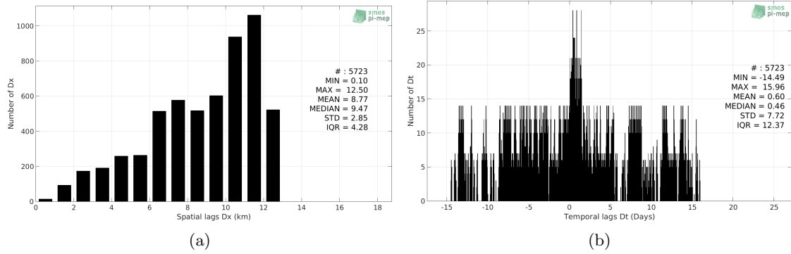
Figure 4: Histograms of the spatial (a) and temporal (b) lags between the location/time of the Sairdrone measurement and the date of the corresponding SMOS SSS L3 v335 - Monthly - 25 km (CATDS-CPDC) SSS pixel.
