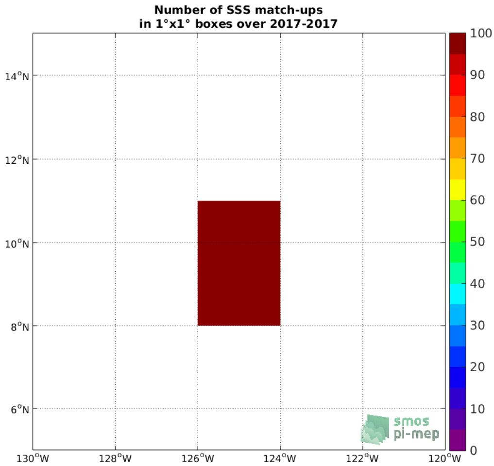
Figure 3: Number of SSS match-ups between Saildrone SSS and the SMOS SSS L3 v335 - Monthly - 25 km (CATDS-CPDC) SSS product for the SPURS 2 Pi-MEP region over 1°x1° boxes and for the full satellite product period.
