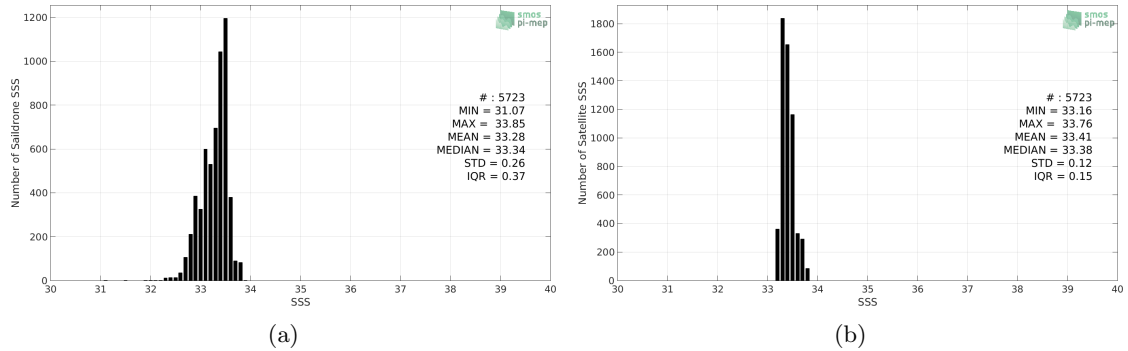
Figure 2: Histograms of SSS from Saildrone (a) and SMOS SSS L3 v335 - Monthly - 25 km (CATDS-CPDC) (b) considering all match-up pairs per bins of 0.1 over the SPURS 2 Pi-MEP region and for the full satellite product period.
