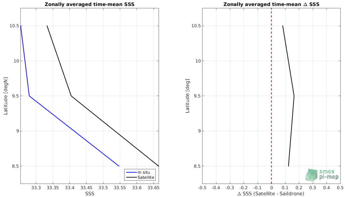
Figure 7: Left panel: Zonal mean SSS from SMOS SSS L3 v335 - Monthly - 25 km (CATDS-CPDC) satellite product (black) and from Sairdrone (blue). Right panel: Zonal mean of \Delta SSS (Satellite - Sairdrone) for all the collected Pi-MEP match-up pairs estimated over the full satellite product period.
