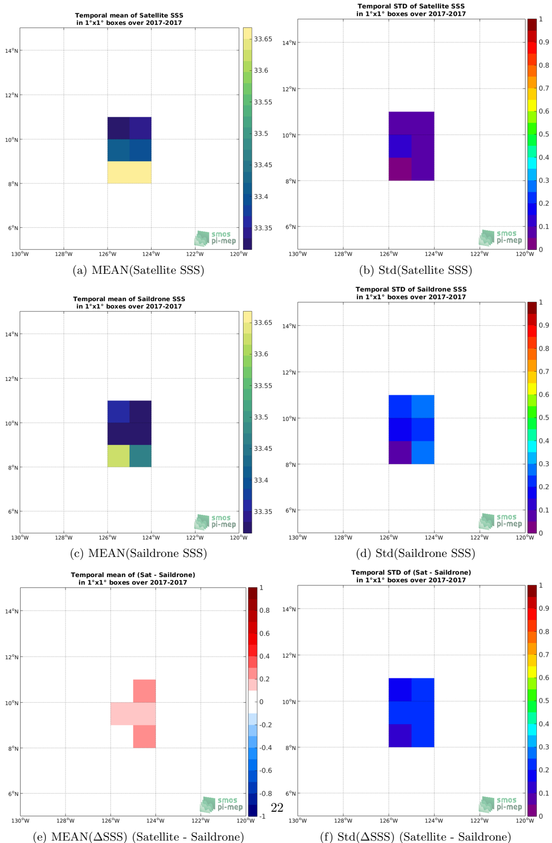
Figure 5: Temporal mean (left) and Std (right) of SSS from SMOS SSS L3 v335 - Monthly - 25 km (CATDS-CPDC) (top), Saildrone (middle), and of \Delta SSS (Satellite - Saildrone). Only match-up pairs are used to generate these maps.
