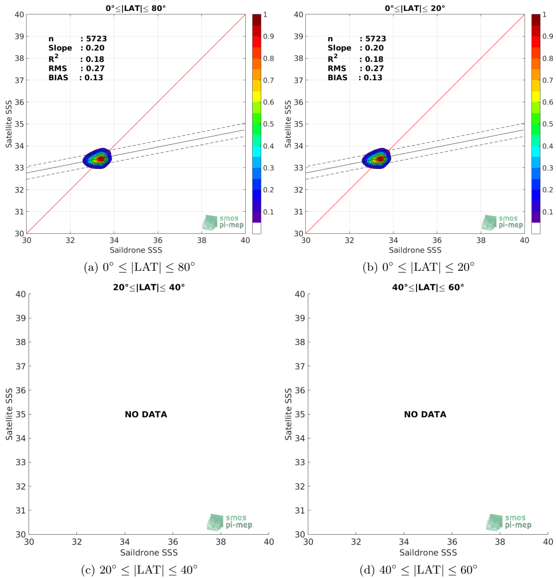
Figure 8: Contour maps of the concentration of SMOS SSS L3 v335 - Monthly - 25 km (CATDS-CPDC) SSS (y-axis) versus SAILDRONE SSS (x-axis) at match-up pairs for different latitude bands. For each plot, the red line shows x=y . The black thin and dashed lines indicate a linear fit through the data cloud and the \pm 95\% confidence levels, respectively. The number match-up pairs n , the slope and R^2 coefficient of the linear fit, the root mean square (RMS) and the mean bias between satellite and in situ data are indicated for each latitude band in each plots.
