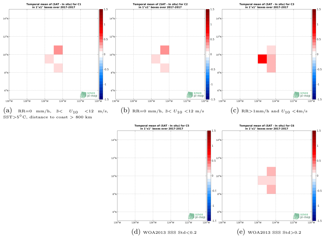
Figure 11: Temporal mean gridded over spatial boxes of size 1^\circ \times 1^\circ of \Delta SSS (SMOS SSS L3 v335 - Monthly - 25 km (CATDS-CPDC) - Saildrone) for 5 different subdatasets corresponding to:RR=0 mm/h, 3 < U_{10} < 12 m/s, SST >5^\circ C, distance to coast > 800 km (a), RR=0 mm/h, 3 < U_{10} < 12 m/s (b), RR >1 mm/h and U_{10} < 4 m/s (c), WOA2013 SSS Std <0.2 (d), WOA2013 SSS Std >0.2 (e).
