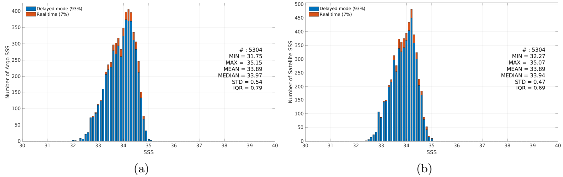
Figure 3: Histograms of SSS from Argo (a) and SMOS SSS L3 v335 - Monthly - 25 km (CATDS-CPDC) (b) considering all match-up pairs per bins of 0.1 over the SPURS 2 Pi-MEP region and for the full satellite product period.
