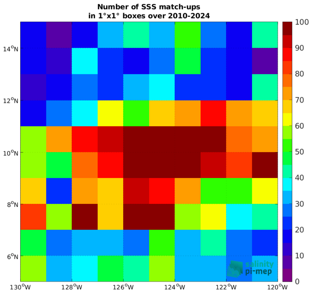
Figure 5: Number of SSS match-ups between Argo SSS and the SMOS SSS L3 v335 - Monthly - 25 km (CATDS-CPDC) SSS product for the SPURS 2 Pi-MEP region over 1°x1° boxes and for the full satellite product period.
