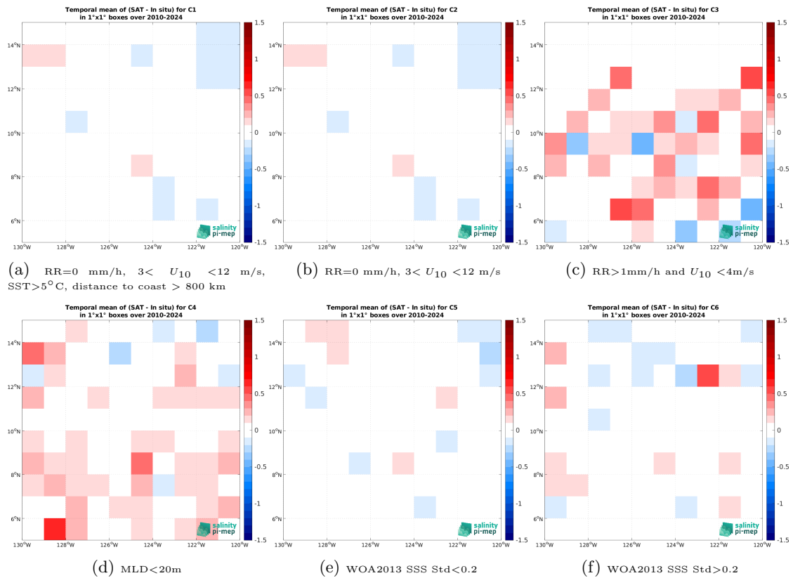
Figure 14: Temporal mean gridded over spatial boxes of size 1^\circ \times 1^\circ of \Delta\text{SSS} (SMOS SSS L3 v335 - Monthly - 25 km (CATDS-CPDC) - Argo) for 6 different subdatasets corresponding to:RR=0 mm/h, 3 < U_{10} < 12 m/s, SST>5°C, distance to coast > 800 km (a), RR=0 mm/h, 3 < U_{10} < 12 m/s (b), RR>1mm/h and U_{10} < 4 m/s (c),MLD<20m (d),WOA2013 SSS Std<0.2 (e),WOA2013 SSS Std>0.2 (f).
