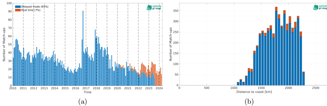
Figure 2: Number of match-ups between Argo and SMOS SSS L3 v335 - Monthly - 25 km (CATDS-CPDC) SSS as a function of time (a) and as function of the distance to coast (b) over the SPURS 2 Pi-MEP region and for the full satellite product period.
