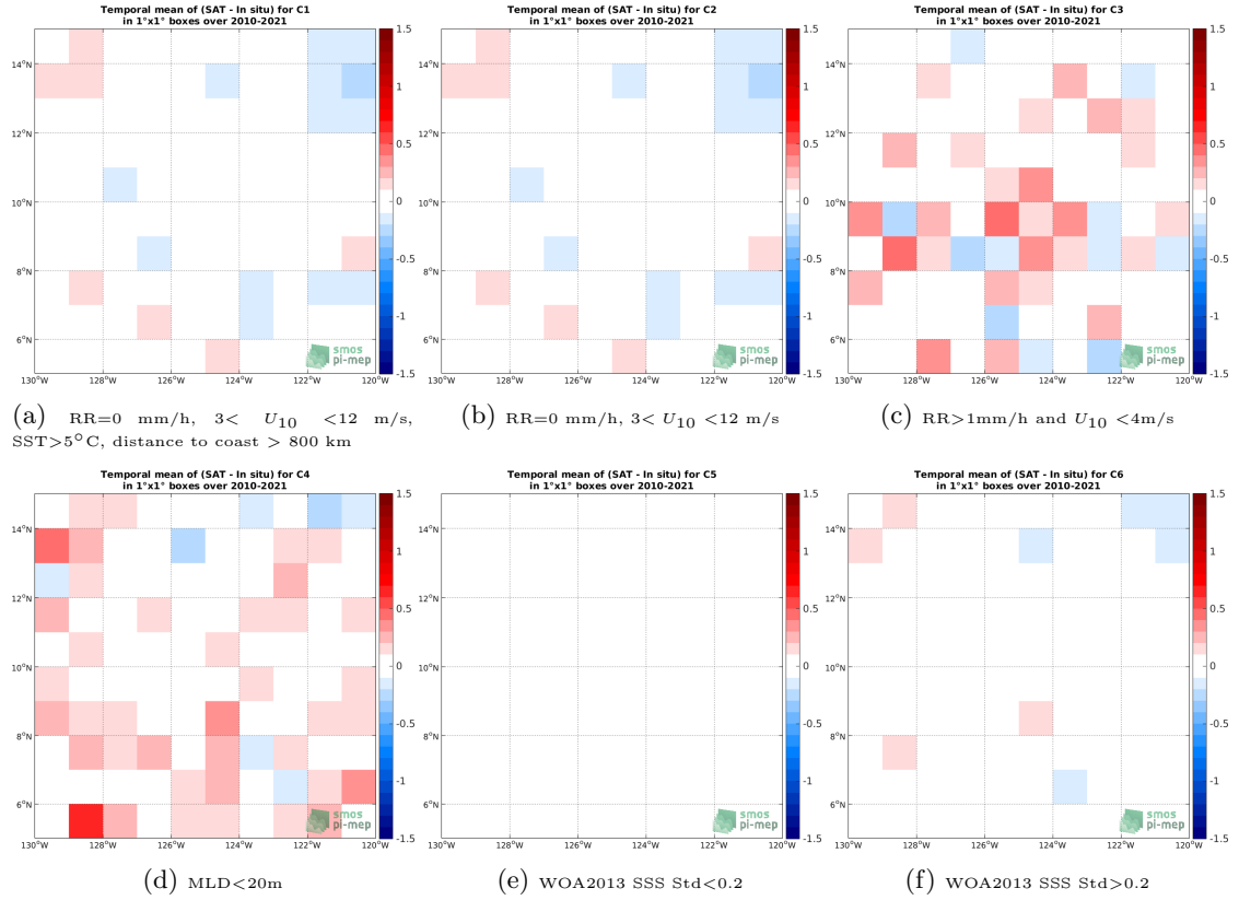
Figure 12: Temporal mean gridded over spatial boxes of size 1^\circ \times 1^\circ of \Delta SSS (SMOS SSS L3 v335 - Monthly - 25 km (CATDS-CPDC) - Argo) for 6 different subdatasets corresponding to: RR=0 mm/h, 3 < U_{10} < 12 m/s, SST > 5^\circ C , distance to coast > 800 km (a), RR=0 mm/h, 3 < U_{10} < 12 m/s (b), RR > 1 mm/h and U_{10} < 4 m/s (c), MLD < 20 m (d), WOA2013 SSS Std < 0.2 (e), WOA2013 SSS Std > 0.2 (f).
