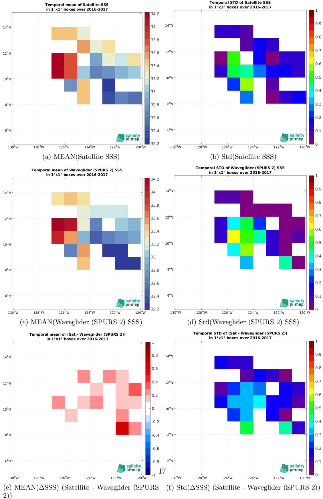
Figure 7: Temporal mean (left) and Std (right) of SSS from SMOS SSS L3 v335 - 10 Days - 25 km (CATDS-CPDC) (top), Waveglider (SPURS 2) (middle), and of \Delta SSS (Satellite - Waveglider (SPURS 2)). Only match-up pairs are used to generate these maps.
