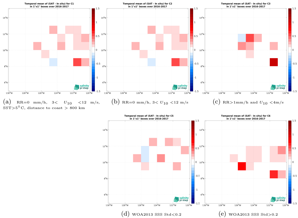
Figure 14: Temporal mean gridded over spatial boxes of size 1^\circ \times 1^\circ of \Delta SSS (SMOS SSS L3 v335 - 10 Days - 25 km (CATDS-CPDC) - Waveglider (SPURS 2)) for 5 different subdatasets corresponding to:RR=0 mm/h, 3 < U_{10} < 12 m/s, SST >5^\circ C, distance to coast > 800 km (a), RR=0 mm/h, 3 < U_{10} < 12 m/s (b), RR >1 mm/h and U_{10} < 4 m/s (c), WOA2013 SSS Std <0.2 (d), WOA2013 SSS Std >0.2 (e).
