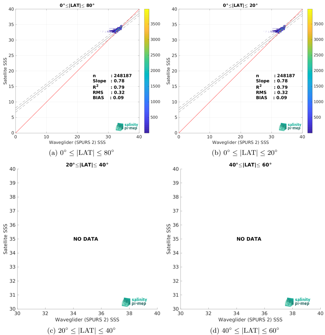
Figure 10: Contour maps of the concentration of SMOS SSS L3 v335 - 10 Days - 25 km (CATDS-CPDC) SSS (y-axis) versus Waveglider (SPURS 2) SSS (x-axis) at match-up pairs for different latitude bands. For each plot, the red line shows x=y . The black thin and dashed lines indicate a linear fit through the data cloud and the \pm 95\% confidence levels, respectively. The number match-up pairs n , the slope and R^2 coefficient of the linear fit, the root mean square (RMS) and the mean bias between satellite and in situ data are indicated for each latitude band in each plots.
