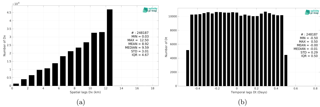
Figure 6: Histograms of the spatial (a) and temporal (b) lags between the location/time of the Waveglider (SPURS 2) measurement and the date of the corresponding SMOS SSS L3 v335 - 10 Days - 25 km (CATDS-CPDC) SSS pixel.
