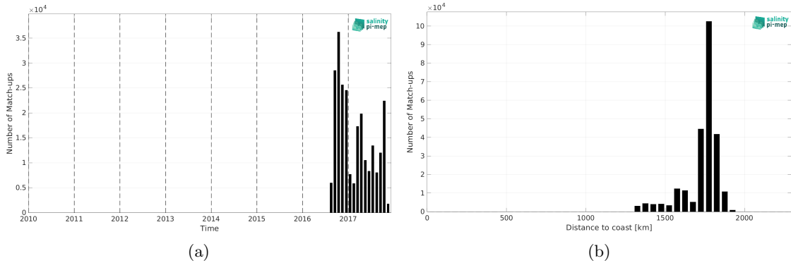
Figure 2: Number of match-ups between Waveglider (SPURS 2) and SMOS SSS L3 v335 - 10 Days - 25 km (CATDS-CPDC) SSS as a function of time (a) and as function of the distance to coast (b) over the SPURS 2 Pi-MEP region and for the full satellite product period.
