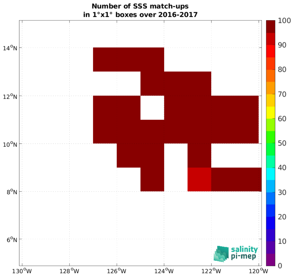
Figure 5: Number of SSS match-ups between Waveglider (SPURS 2) SSS and the SMOS SSS L3 v335 - 10 Days - 25 km (CATDS-CPDC) SSS product for the SPURS 2 Pi-MEP region over 1^\circ \times 1^\circ boxes and for the full satellite product period.
