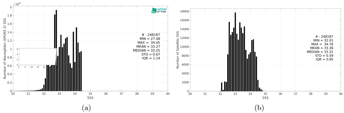
Figure 3: Histograms of SSS from Waveglider (SPURS 2) (a) and SMOS SSS L3 v335 - 10 Days - 25 km (CATDS-CPDC) (b) considering all match-up pairs per bins of 0.1 over the SPURS 2 Pi-MEP region and for the full satellite product period.
