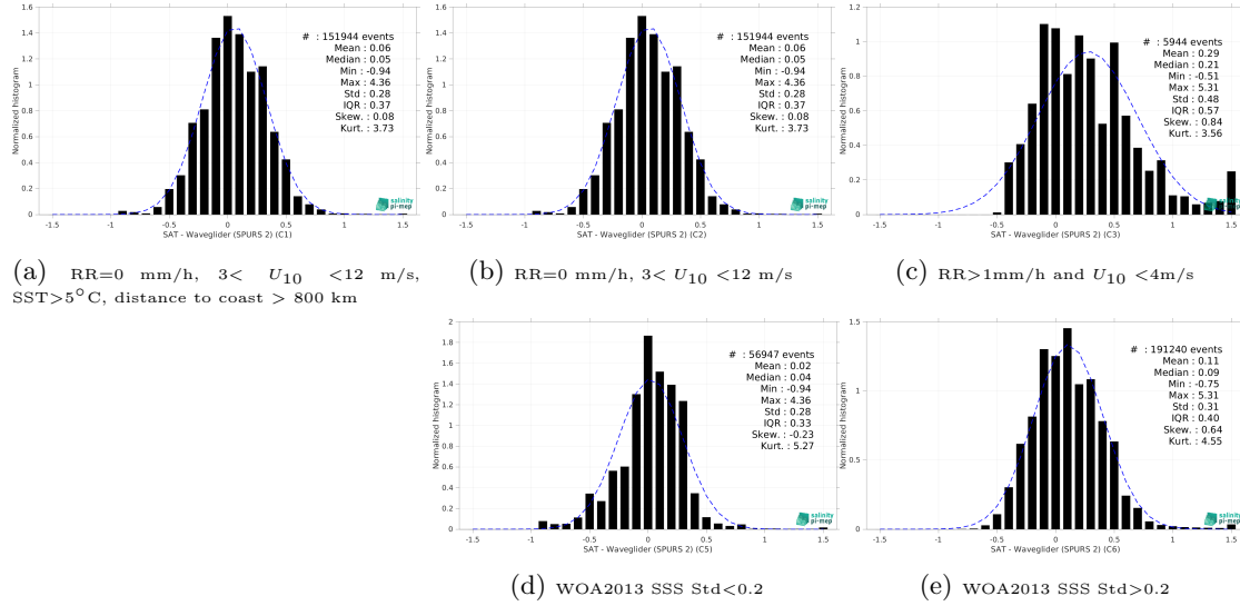
Figure 15: Normalized histogram of \Delta SSS (SMOS SSS L3 v335 - 10 Days - 25 km (CATDS-CPDC) - Waveglider (SPURS 2) for 5 different subdatasets corresponding to: RR=0 mm/h, 3 < U_{10} < 12 m/s, SST > 5°C, distance to coast > 800 km (a), RR=0 mm/h, 3 < U_{10} < 12 m/s (b), RR > 1mm/h and U_{10} < 4 m/s (c), WOA2013 SSS Std < 0.2 (d), WOA2013 SSS Std > 0.2 (e).
