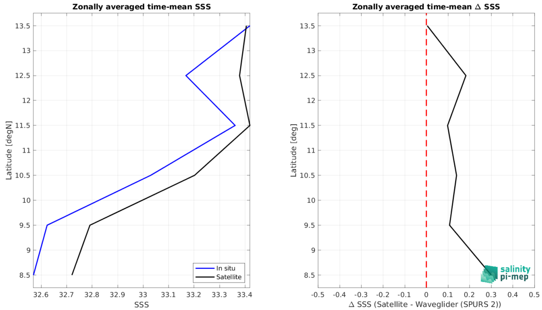
Figure 9: Left panel: Zonal mean SSS from SMOS SSS L3 v335 - 10 Days - 25 km (CATDS-CPDC) satellite product (black) and from Waveglider (SPURS 2) (blue). Right panel: Zonal mean of \Delta SSS (Satellite - Waveglider (SPURS 2)) for all the collected Pi-MEP match-up pairs estimated over the full satellite product period.
