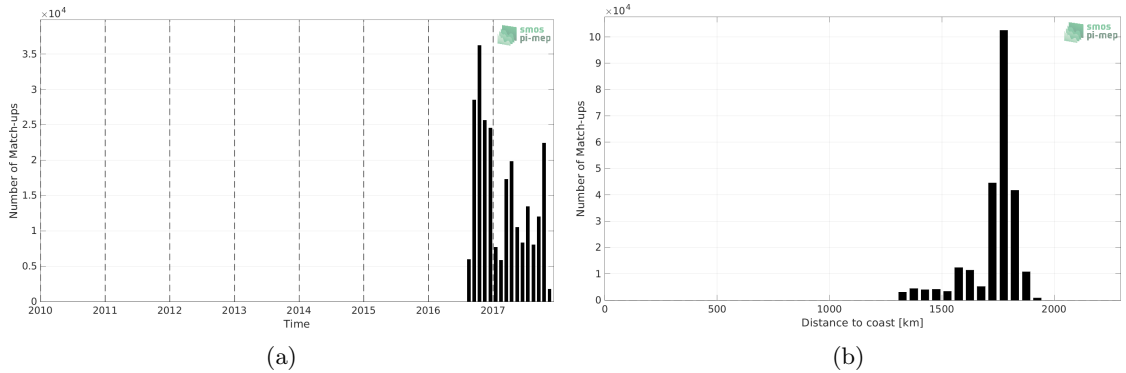
Figure 1: Number of match-ups between Waveglider (SPURS 2) and SMOS SSS L3 v335 - 10 Days - 25 km (CATDS-CPDC) SSS as a function of time (a) and as function of the distance to coast (b) over the SPURS 2 Pi-MEP region and for the full satellite product period.
