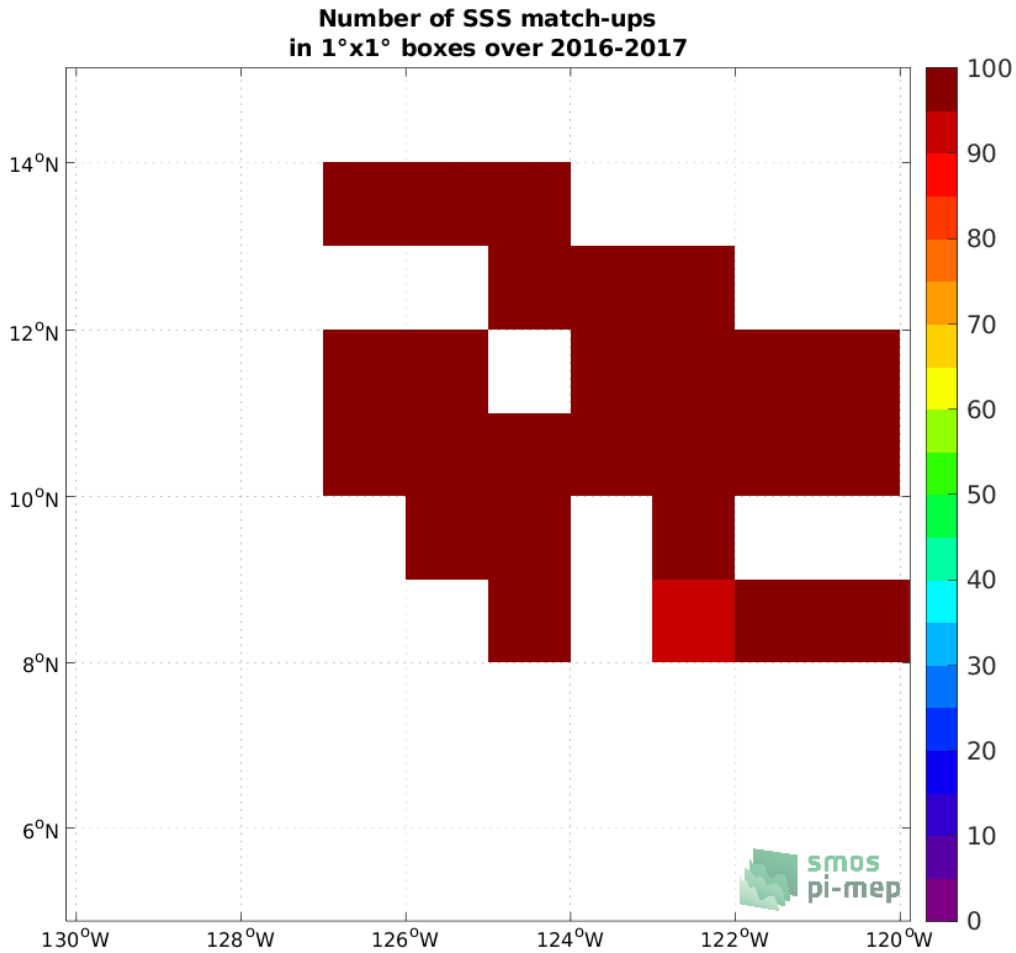
Figure 4: Number of SSS match-ups between Waveglider (SPURS 2) SSS and the SMOS SSS L3 v335 - 10 Days - 25 km (CATDS-CPDC) SSS product for the SPURS 2 Pi-MEP region over 1^\circ \times 1^\circ boxes and for the full satellite product period.
