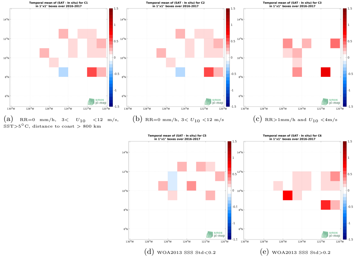
Figure 12: Temporal mean gridded over spatial boxes of size 1^{\circ}\times 1^{\circ} of \Delta\text{SSS} (SMOS SSS L3 v335 - 10 Days - 25 km (CATDS-CPDC) - Waveglider (SPURS 2)) for 5 different subdatasets corresponding to:RR=0 mm/h, 3 < U_{10} < 12 m/s, SST >5^{\circ}\text{C} , distance to coast > 800 km (a), RR=0 mm/h, 3 < U_{10} < 12 m/s (b), RR >1 mm/h and U_{10} < 4 m/s (c), WOA2013 SSS Std <0.2 (d), WOA2013 SSS Std >0.2 (e).
