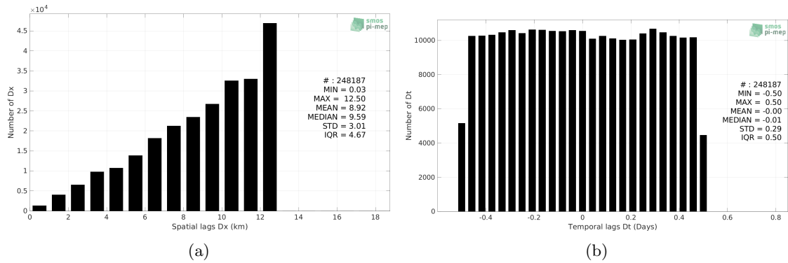
Figure 5: Histograms of the spatial (a) and temporal (b) lags between the location/time of the Waveglider (SPURS 2) measurement and the date of the corresponding SMOS SSS L3 v335 - 10 Days - 25 km (CATDS-CPDC) SSS pixel.
