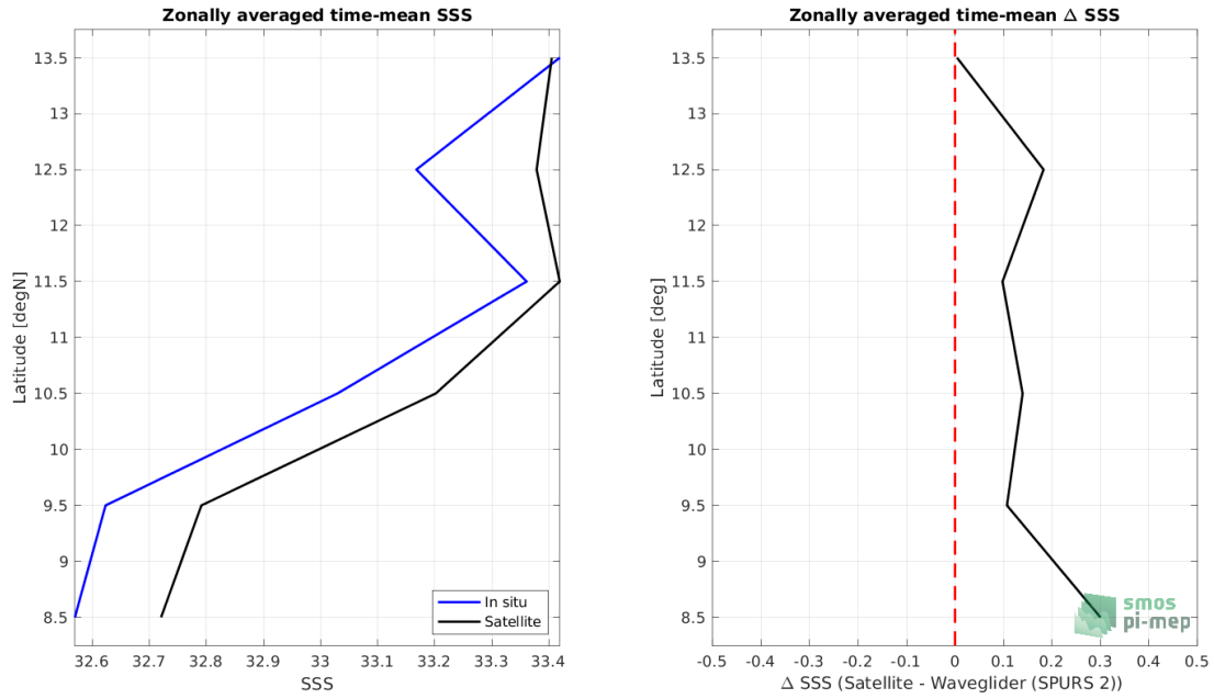
Figure 8: Left panel: Zonal mean SSS from SMOS SSS L3 v335 - 10 Days - 25 km (CATDS-CPDC) satellite product (black) and from Waveglider (SPURS 2) (blue). Right panel: Zonal mean of \Delta SSS (Satellite - Waveglider (SPURS 2)) for all the collected Pi-MEP match-up pairs estimated over the full satellite product period.
