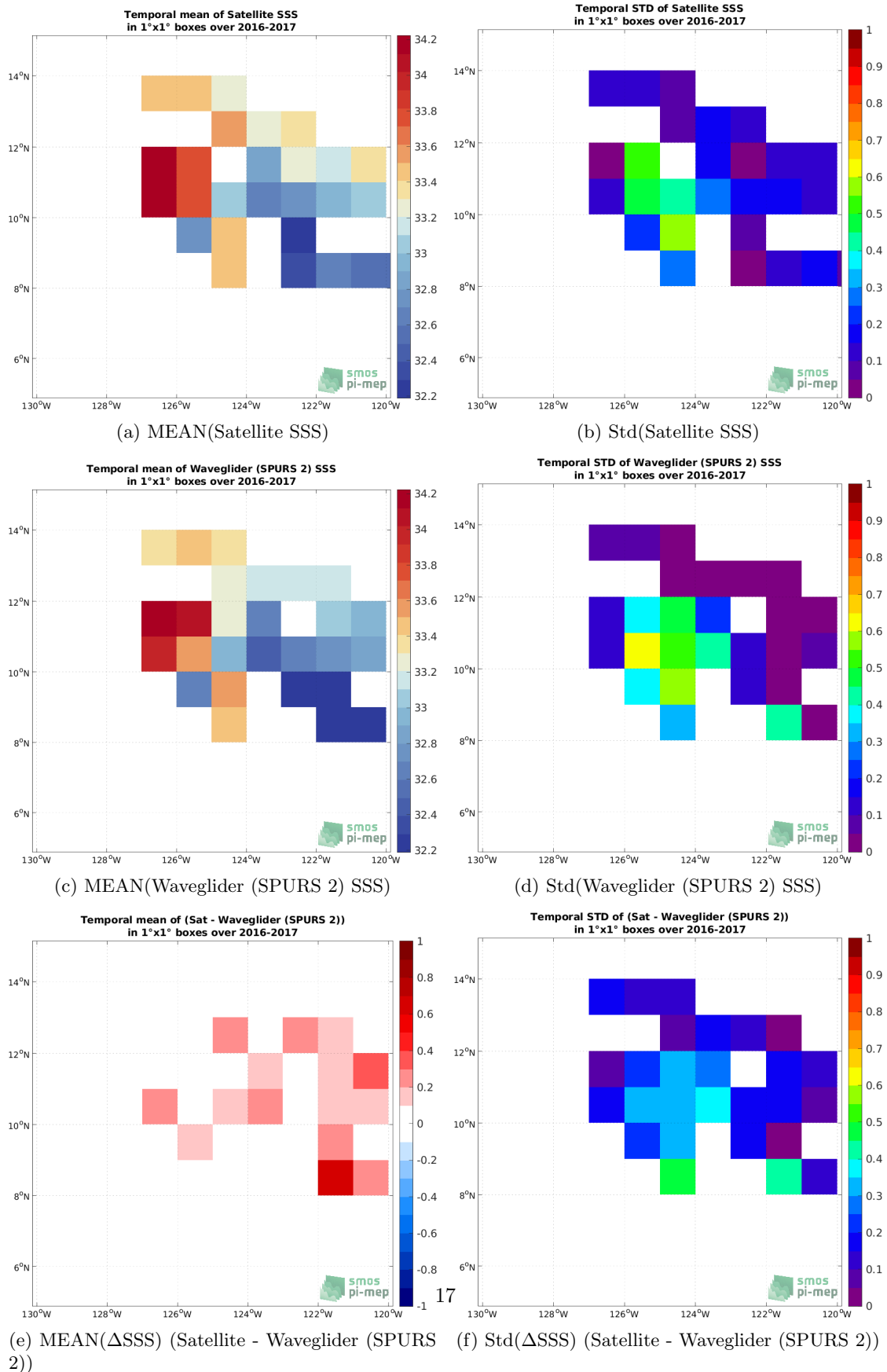
Figure 6: Temporal mean (left) and Std (right) of SSS from SMOS SSS L3 v335 - 10 Days - 25 km (CATDS-CPDC) (top), Waveglider (SPURS 2) (middle), and of \Delta SSS (Satellite - Waveglider (SPURS 2)). Only match-up pairs are used to generate these maps.
