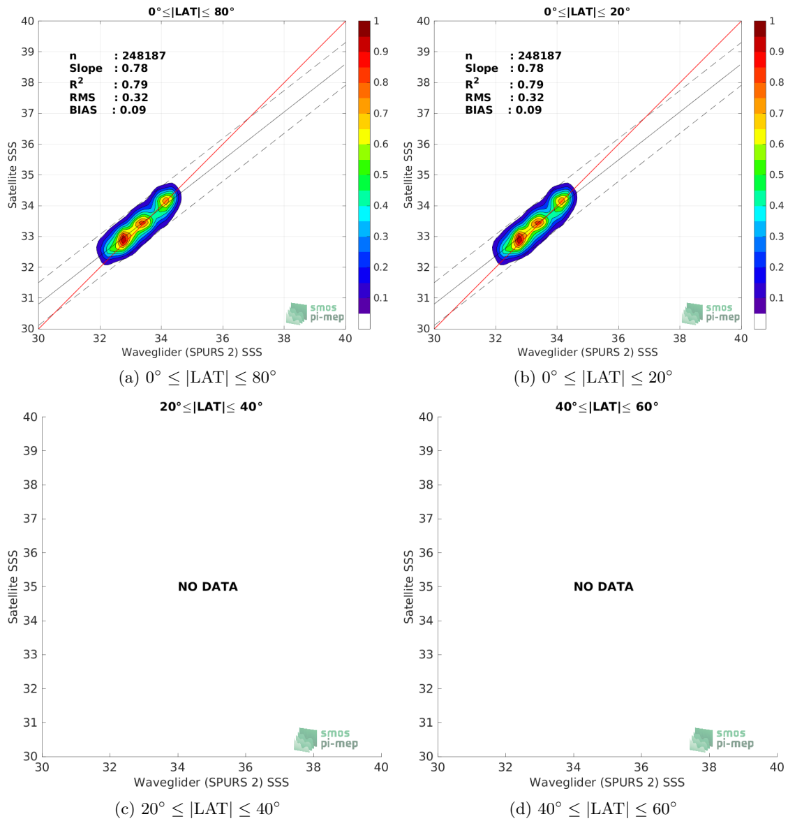
Figure 9: Contour maps of the concentration of SMOS SSS L3 v335 - 10 Days - 25 km (CATDS-CPDC) SSS (y-axis) versus Waveglider (SPURS 2) SSS (x-axis) at match-up pairs for different latitude bands. For each plot, the red line shows x=y . The black thin and dashed lines indicate a linear fit through the data cloud and the \pm 95\% confidence levels, respectively. The number match-up pairs n , the slope and R^2 coefficient of the linear fit, the root mean square (RMS) and the mean bias between satellite and in situ data are indicated for each latitude band in each plots.
