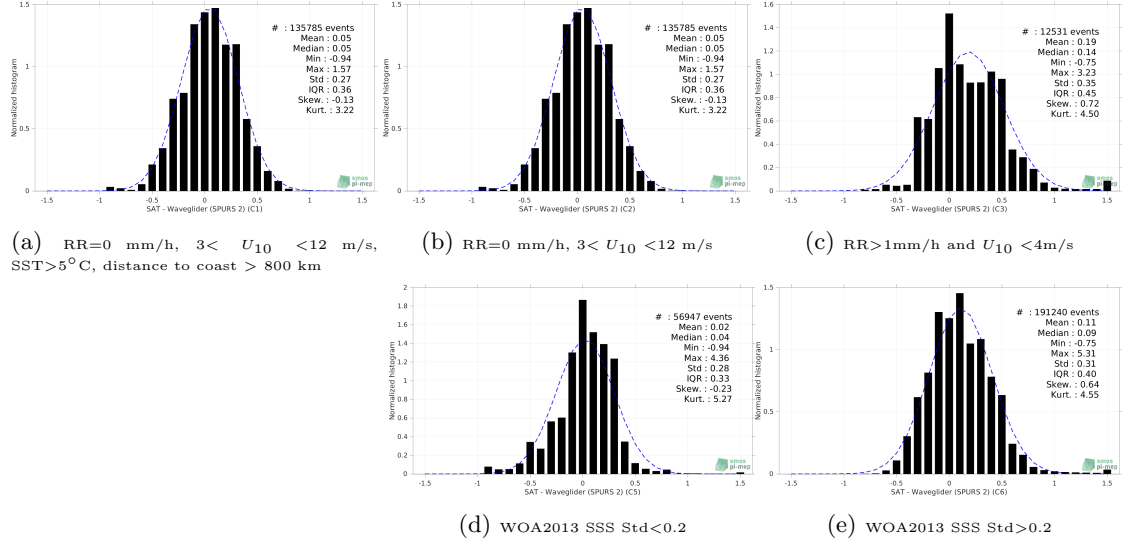
Figure 13: Normalized histogram of \Delta SSS (SMOS SSS L3 v335 - 10 Days - 25 km (CATDS-CPDC) - Waveglider (SPURS 2) for 5 different subdatasets corresponding to: RR=0 mm/h, 3 < U_{10} < 12 m/s, SST > 5°C, distance to coast > 800 km (a), RR=0 mm/h, 3 < U_{10} < 12 m/s (b), RR > 1mm/h and U_{10} < 4 m/s (c), WOA2013 SSS Std < 0.2 (d), WOA2013 SSS Std > 0.2 (e).
