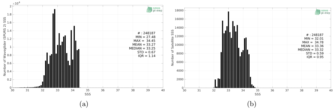
Figure 2: Histograms of SSS from Waveglider (SPURS 2) (a) and SMOS SSS L3 v335 - 10 Days - 25 km (CATDS-CPDC) (b) considering all match-up pairs per bins of 0.1 over the SPURS 2 Pi-MEP region and for the full satellite product period.
