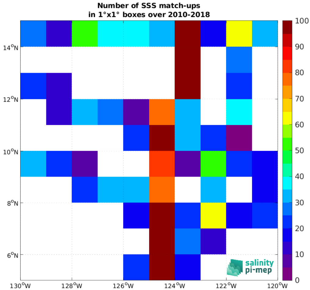
Figure 5: Number of SSS match-ups between TSG (SAMOS) SSS and the SMOS SSS L3 v335 - 10 Days - 25 km (CATDS-CPDC) SSS product for the SPURS 2 Pi-MEP region over 1°x1° boxes and for the full satellite product period.
