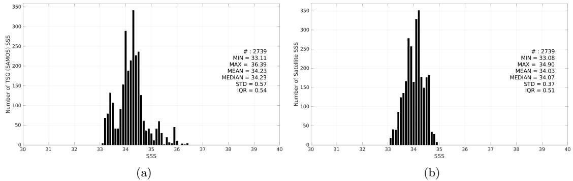
Figure 3: Histograms of SSS from TSG (SAMOS) (a) and SMOS SSS L3 v335 - 10 Days - 25 km (CATDS-CPDC) (b) considering all match-up pairs per bins of 0.1 over the SPURS 2 Pi-MEP region and for the full satellite product period.
