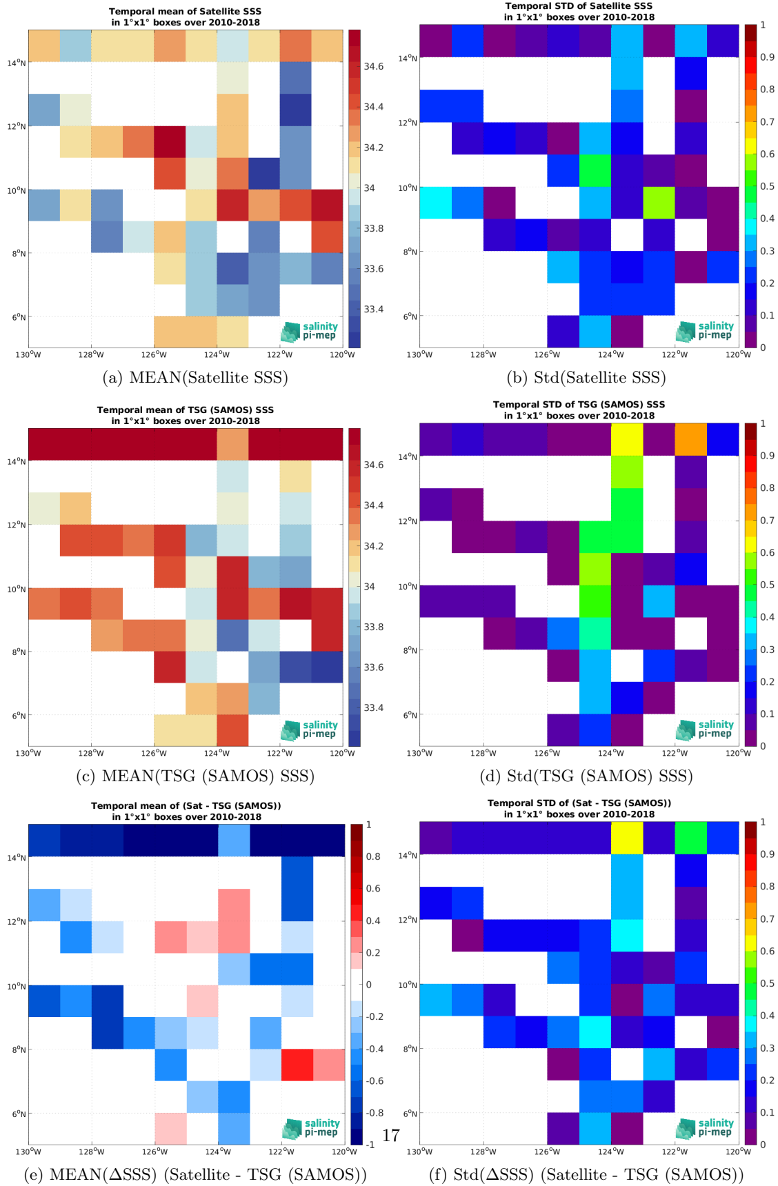
Figure 7: Temporal mean (left) and Std (right) of SSS from SMOS SSS L3 v335 - 10 Days - 25 km (CATDS-CPDC) (top), TSG (SAMOS) (middle), and of \Delta SSS (Satellite - TSG (SAMOS)). Only match-up pairs are used to generate these maps.
