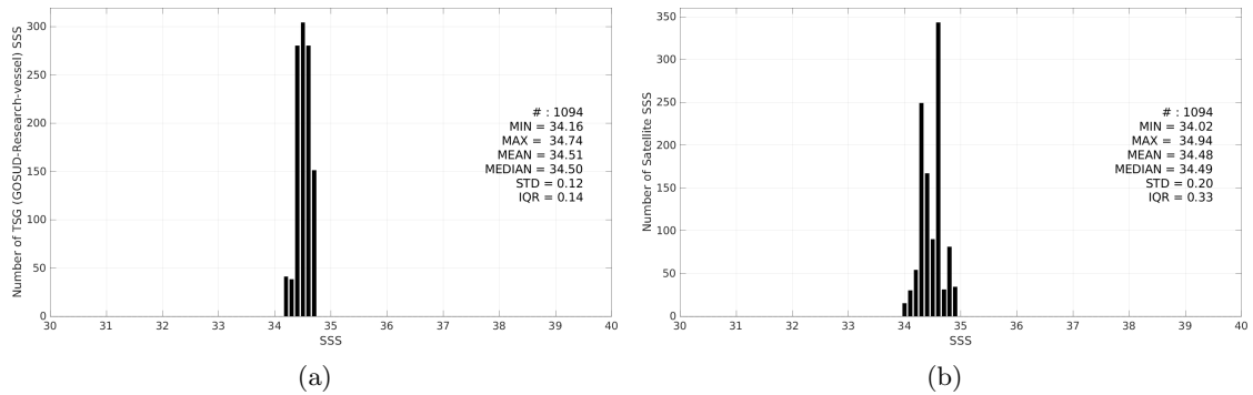
Figure 3: Histograms of SSS from TSG (GOSUD-Research-vessel) (a) and SMOS SSS L3 v335 - 10 Days - 25 km (CATDS-CPDC) (b) considering all match-up pairs per bins of 0.1 over the SPURS 2 Pi-MEP region and for the full satellite product period.
