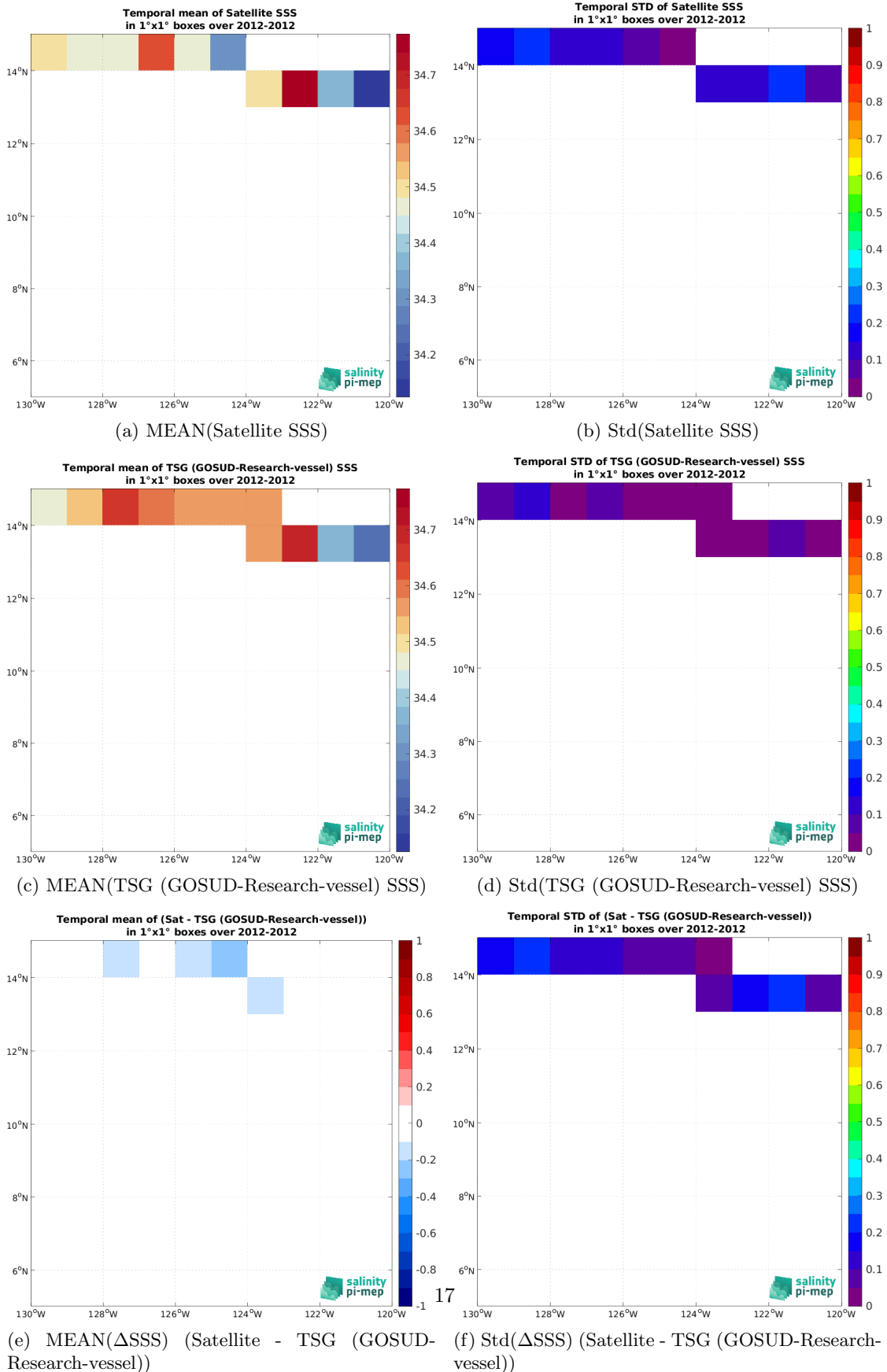
Figure 7: Temporal mean (left) and Std (right) of SSS from SMOS SSS L3 v335 - 10 Days - 25 km (CATDS-CPDC) (top), TSG (GOSUD-Research-vessel) (middle), and of \Delta SSS (Satellite - TSG (GOSUD-Research-vessel)). Only match-up pairs are used to generate these maps.
