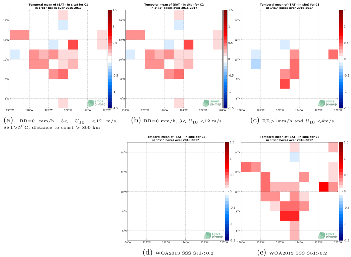
Figure 11: Temporal mean gridded over spatial boxes of size 1^\circ \times 1^\circ of \Delta\text{SSS} (SMOS SSS L3 v335 - 10 Days - 25 km (CATDS-CPDC) - Salinity Snake) for 5 different subdatasets corresponding to:RR=0 mm/h, 3 < U_{10} < 12 m/s, SST >5^\circ\text{C} , distance to coast > 800 km (a), RR=0 mm/h, 3 < U_{10} < 12 m/s (b), RR >1 mm/h and U_{10} < 4 m/s (c), WOA2013 SSS Std <0.2 (d), WOA2013 SSS Std >0.2 (e).
