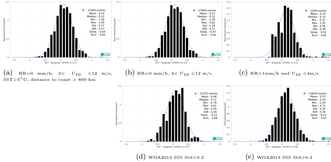
Figure 15: Normalized histogram of \Delta SSS (SMOS SSS L3 v335 - 10 Days - 25 km (CATDS-CPDC) - Seaglider (SPURS 2)) for 5 different subdatasets corresponding to: RR=0 mm/h, 3 < U_{10} < 12 m/s, SST>5°C, distance to coast > 800 km (a), RR=0 mm/h, 3 < U_{10} < 12 m/s (b), RR>1mm/h and U_{10} < 4 m/s (c), WOA2013 SSS Std<0.2 (d), WOA2013 SSS Std>0.2 (e).
