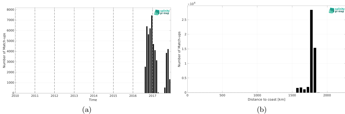
Figure 2: Number of match-ups between Seaglider (SPURS 2) and SMOS SSS L3 v335 - 10 Days - 25 km (CATDS-CPDC) SSS as a function of time (a) and as function of the distance to coast (b) over the SPURS 2 Pi-MEP region and for the full satellite product period.
