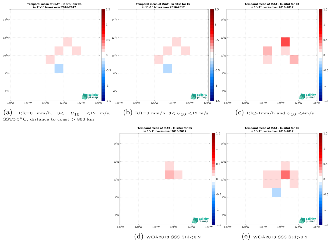
Figure 14: Temporal mean gridded over spatial boxes of size 1^\circ \times 1^\circ of \Delta SSS (SMOS SSS L3 v335 - 10 Days - 25 km (CATDS-CPDC) - Seaglider (SPURS 2)) for 5 different subdatasets corresponding to:RR=0 mm/h, 3 < U_{10} < 12 m/s, SST >5^\circ C, distance to coast > 800 km (a), RR=0 mm/h, 3 < U_{10} < 12 m/s (b), RR >1 mm/h and U_{10} < 4 m/s (c), WOA2013 SSS Std <0.2 (d), WOA2013 SSS Std >0.2 (e).
