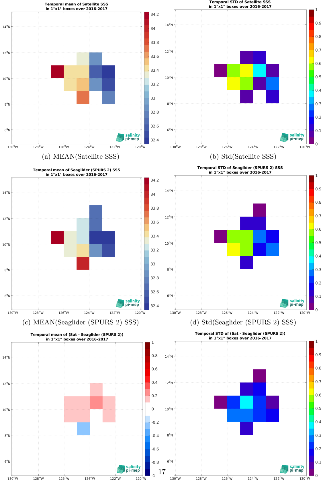
Figure 7: Temporal mean (left) and Std (right) of SSS from SMOS SSS L3 v335 - 10 Days - 25 km (CATDS-CPDC) (top), Seaglider (SPURS 2) (middle), and of \Delta SSS (Satellite - Seaglider (SPURS 2)). Only match-up pairs are used to generate these maps.
