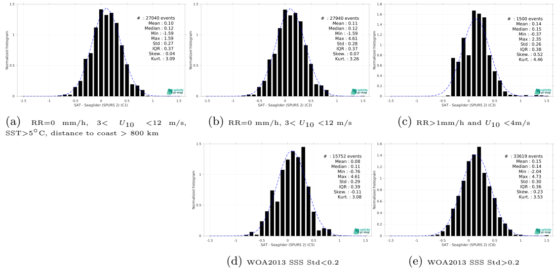
Figure 15: Normalized histogram of \Delta\text{SSS} (SMOS SSS L3 v335 - 10 Days - 25 km (CATDS-CPDC) - Seaglider (SPURS 2)) for 5 different subdatasets corresponding to: RR=0 mm/h, 3 < U_{10} < 12 m/s, SST>5°C, distance to coast > 800 km (a), RR=0 mm/h, 3 < U_{10} < 12 m/s (b), RR>1mm/h and U_{10} < 4 m/s (c), WOA2013 SSS Std<0.2 (d), WOA2013 SSS Std>0.2 (e).
