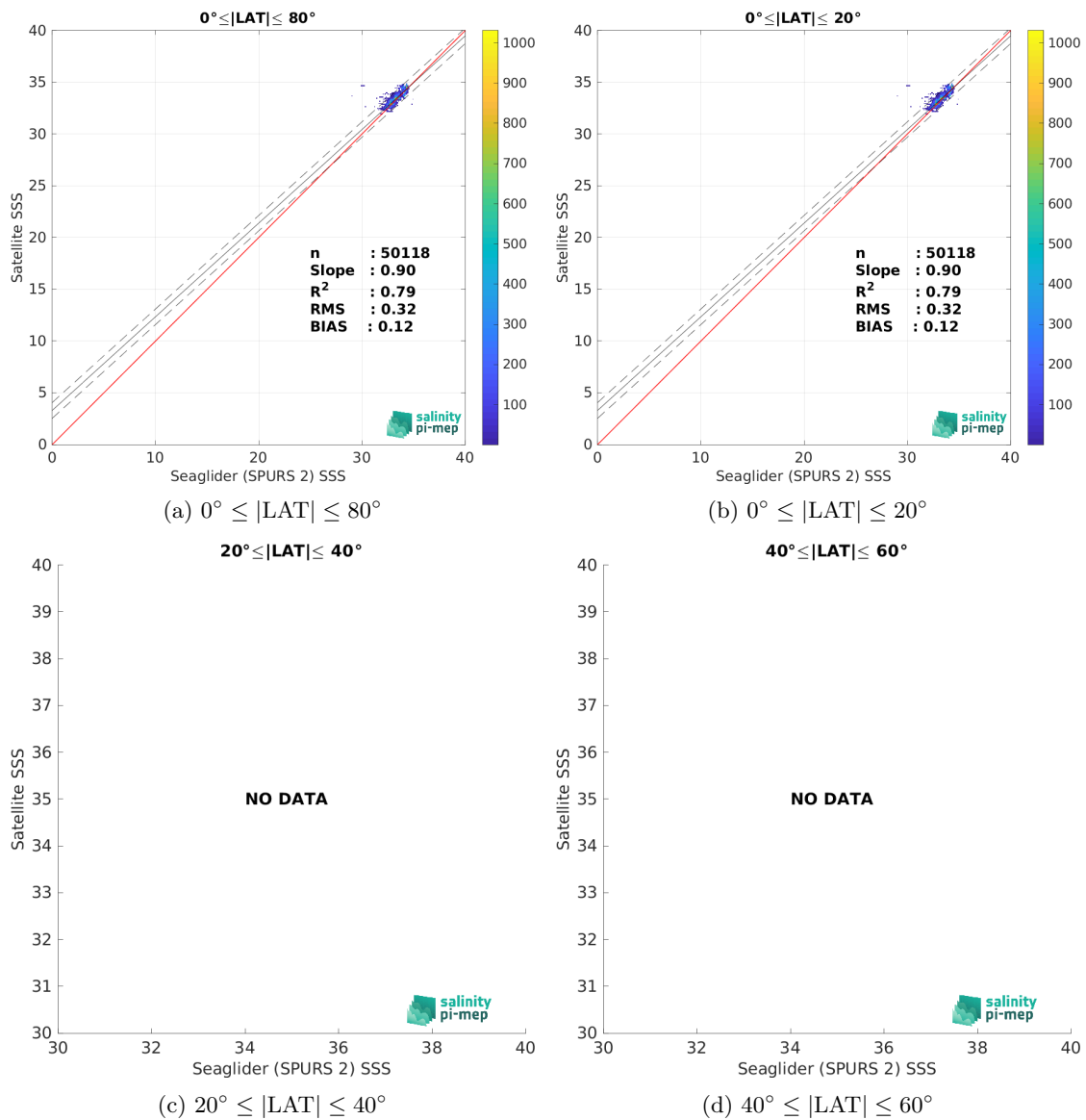
Figure 10: Contour maps of the concentration of SMOS SSS L3 v335 - 10 Days - 25 km (CATDS-CPDC) SSS (y-axis) versus Seaglider (SPURS 2) SSS (x-axis) at match-up pairs for different latitude bands. For each plot, the red line shows x=y . The black thin and dashed lines indicate a linear fit through the data cloud and the \pm 95\% confidence levels, respectively. The number match-up pairs n , the slope and R^2 coefficient of the linear fit, the root mean square (RMS) and the mean bias between satellite and in situ data are indicated for each latitude band in each plots.
