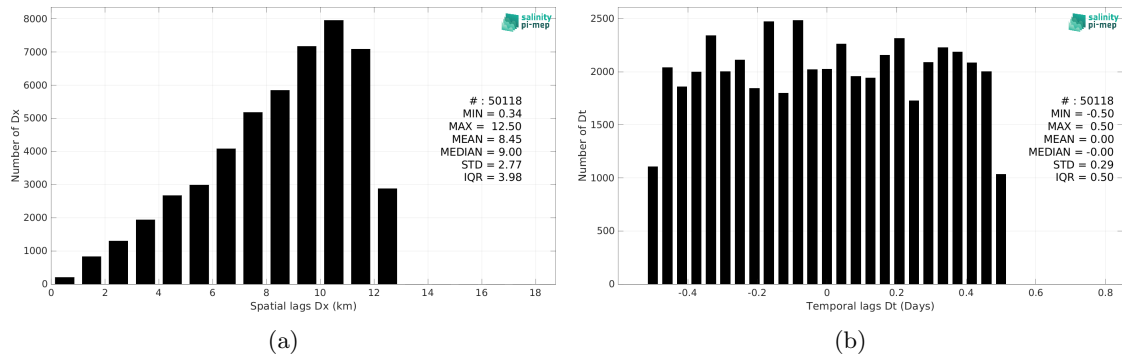
Figure 6: Histograms of the spatial (a) and temporal (b) lags between the location/time of the Seaglider (SPURS 2) measurement and the date of the corresponding SMOS SSS L3 v335 - 10 Days - 25 km (CATDS-CPDC) SSS pixel.
