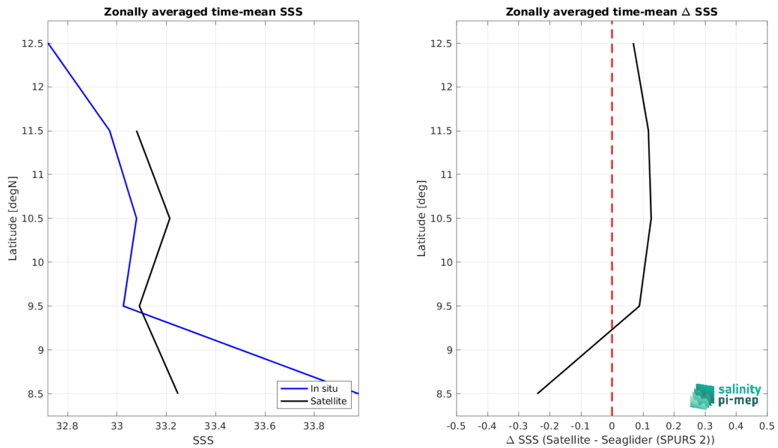
Figure 9: Left panel: Zonal mean SSS from SMOS SSS L3 v335 - 10 Days - 25 km (CATDS-CPDC) satellite product (black) and from Seaglider (SPURS 2) (blue). Right panel: Zonal mean of \Delta SSS (Satellite - Seaglider (SPURS 2)) for all the collected Pi-MEP match-up pairs estimated over the full satellite product period.
