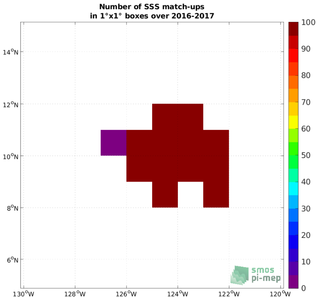
Figure 4: Number of SSS match-ups between Seaglider (SPURS 2) SSS and the SMOS SSS L3 v335 - 10 Days - 25 km (CATDS-CPDC) SSS product for the SPURS 2 Pi-MEP region over 1^\circ \times 1^\circ boxes and for the full satellite product period.
