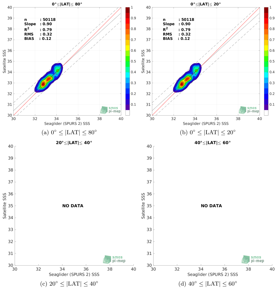
Figure 9: Contour maps of the concentration of SMOS SSS L3 v335 - 10 Days - 25 km (CATDS-CPDC) SSS (y-axis) versus Seaglider (SPURS 2) SSS (x-axis) at match-up pairs for different latitude bands. For each plot, the red line shows x=y . The black thin and dashed lines indicate a linear fit through the data cloud and the \pm 95\% confidence levels, respectively. The number match-up pairs n , the slope and R^2 coefficient of the linear fit, the root mean square (RMS) and the mean bias between satellite and in situ data are indicated for each latitude band in each plots.
