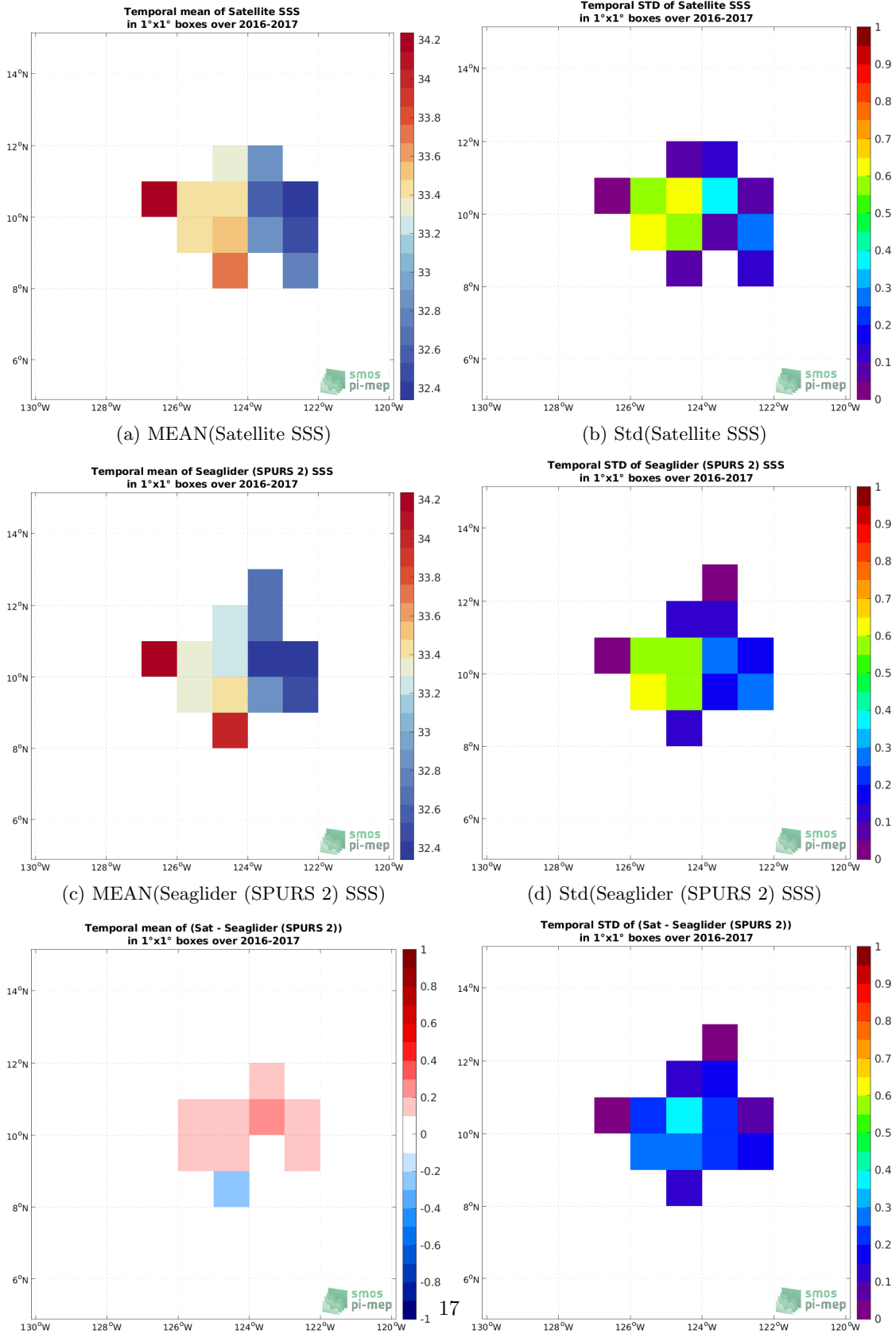
Figure 6: Temporal mean (left) and Std (right) of SSS from SMOS SSS L3 v335 - 10 Days - 25 km (CATDS-CPDC) (top), Seaglider (SPURS 2) (middle), and of \Delta SSS (Satellite - Seaglider (SPURS 2)). Only match-up pairs are used to generate these maps.
