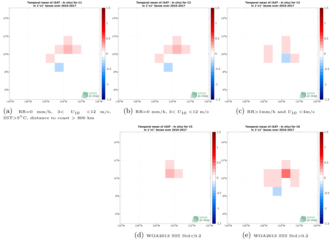
Figure 12: Temporal mean gridded over spatial boxes of size 1^{\circ}\times 1^{\circ} of \Delta\text{SSS} (SMOS SSS L3 v335 - 10 Days - 25 km (CATDS-CPDC) - Seaglider (SPURS 2)) for 5 different subdatasets corresponding to:RR=0 mm/h, 3 < U_{10} < 12 m/s, SST > 5^{\circ}\text{C} , distance to coast > 800 km (a), RR=0 mm/h, 3 < U_{10} < 12 m/s (b), RR > 1 mm/h and U_{10} < 4 m/s (c), WOA2013 SSS Std < 0.2 (d), WOA2013 SSS Std > 0.2 (e).
