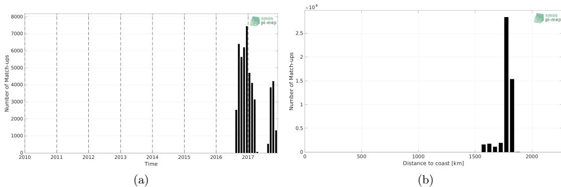
Figure 1: Number of match-ups between Seaglider (SPURS 2) and SMOS SSS L3 v335 - 10 Days - 25 km (CATDS-CPDC) SSS as a function of time (a) and as function of the distance to coast (b) over the SPURS 2 Pi-MEP region and for the full satellite product period.
