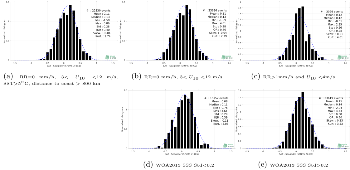
Figure 13: Normalized histogram of \Delta\text{SSS} (SMOS SSS L3 v335 - 10 Days - 25 km (CATDS-CPDC) - Seaglider (SPURS 2)) for 5 different subdatasets corresponding to: RR=0 mm/h, 3 < U_{10} < 12 m/s, SST>5°C, distance to coast > 800 km (a), RR=0 mm/h, 3 < U_{10} < 12 m/s (b), RR>1mm/h and U_{10} < 4 m/s (c), WOA2013 SSS Std<0.2 (d), WOA2013 SSS Std>0.2 (e).
