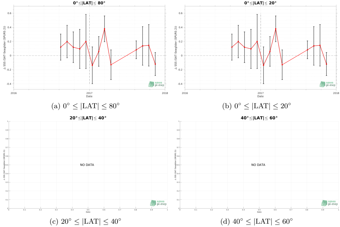
Figure 10: Monthly median (red curves) of \Delta SSS (Satellite - Seaglider (SPURS 2)) and \pm 1 Std (black vertical thick bars) as function of time for all the collected Pi-MEP match-up pairs estimated over the SPURS 2 Pi-MEP region and for the full satellite product period are shown for different latitude bands: (a) 80^\circ\text{S}-80^\circ\text{N} , (b) 20^\circ\text{S}-20^\circ\text{N} , (c) 40^\circ\text{S}-20^\circ\text{S} and 20^\circ\text{N}-40^\circ\text{N} and (d) 60^\circ\text{S}-40^\circ\text{S} and 40^\circ\text{N}-60^\circ\text{N} .
