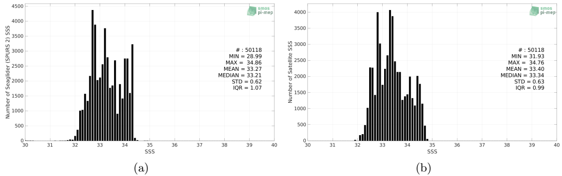
Figure 2: Histograms of SSS from Seaglider (SPURS 2) (a) and SMOS SSS L3 v335 - 10 Days - 25 km (CATDS-CPDC) (b) considering all match-up pairs per bins of 0.1 over the SPURS 2 Pi-MEP region and for the full satellite product period.
