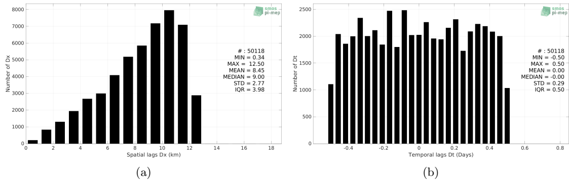
Figure 5: Histograms of the spatial (a) and temporal (b) lags between the location/time of the Seaglider (SPURS 2) measurement and the date of the corresponding SMOS SSS L3 v335 - 10 Days - 25 km (CATDS-CPDC) SSS pixel.
