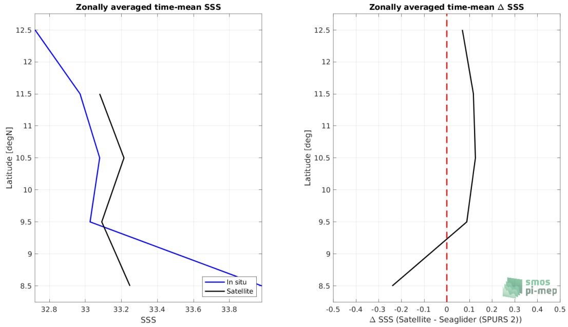
Figure 8: Left panel: Zonal mean SSS from SMOS SSS L3 v335 - 10 Days - 25 km (CATDS-CPDC) satellite product (black) and from Seaglider (SPURS 2) (blue). Right panel: Zonal mean of \Delta SSS (Satellite - Seaglider (SPURS 2)) for all the collected Pi-MEP match-up pairs estimated over the full satellite product period.
