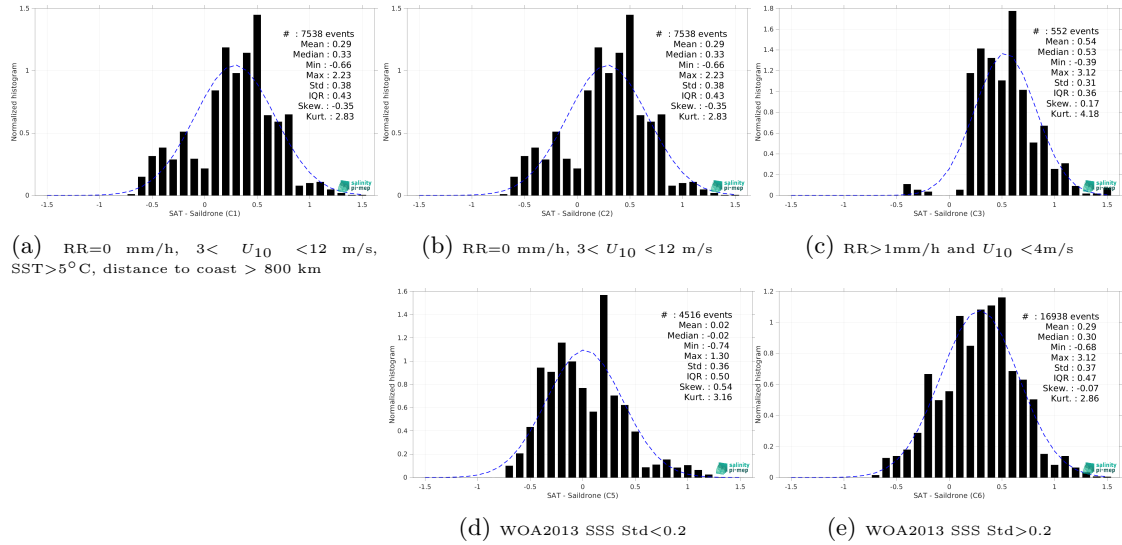
Figure 15: Normalized histogram of \Delta SSS (SMOS SSS L3 v335 - 10 Days - 25 km (CATDS-CPDC) - Sailability) for 5 different subdatasets corresponding to: RR=0 mm/h, 3 < U_{10} < 12 m/s, SST > 5°C, distance to coast > 800 km (a), RR=0 mm/h, 3 < U_{10} < 12 m/s (b), RR > 1mm/h and U_{10} < 4 m/s (c), WOA2013 SSS Std < 0.2 (d), WOA2013 SSS Std > 0.2 (e).
