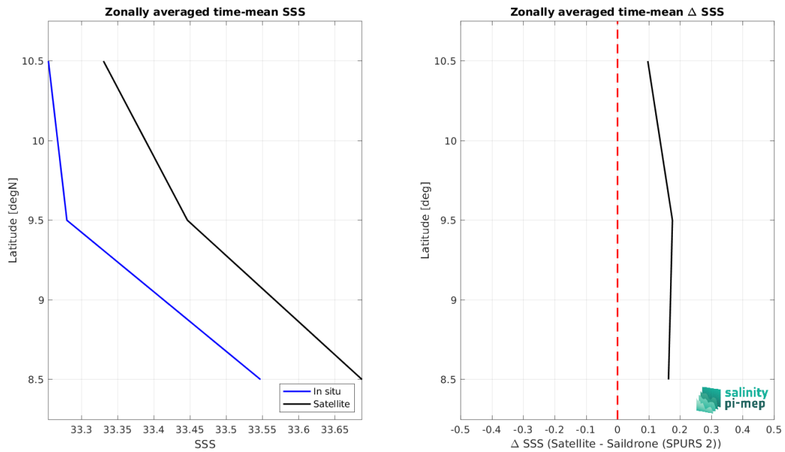
Figure 9: Left panel: Zonal mean SSS from SMOS SSS L3 v335 - 10 Days - 25 km (CATDS-CPDC) satellite product (black) and from Saildrone (SPURS 2) (blue). Right panel: Zonal mean of \Delta SSS (Satellite - Saildrone (SPURS 2)) for all the collected Pi-MEP match-up pairs estimated over the full satellite product period.
