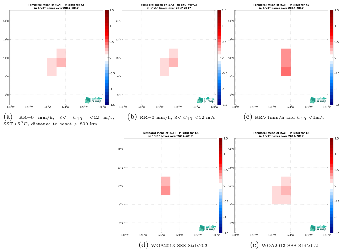
Figure 14: Temporal mean gridded over spatial boxes of size 1^\circ \times 1^\circ of \Delta\text{SSS} (SMOS SSS L3 v335 - 10 Days - 25 km (CATDS-CPDC) - Saildrone (SPURS 2)) for 5 different subdatasets corresponding to:RR=0 mm/h, 3 < U_{10} < 12 m/s, SST>5°C, distance to coast > 800 km (a), RR=0 mm/h, 3 < U_{10} < 12 m/s (b), RR>1mm/h and U_{10} < 4 m/s (c), WOA2013 SSS Std<0.2 (d), WOA2013 SSS Std>0.2 (e).
