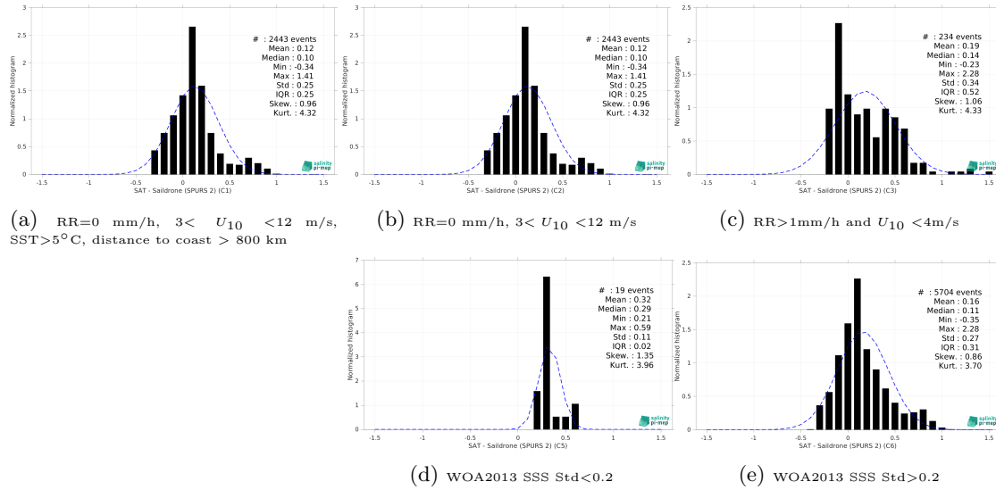
Figure 15: Normalized histogram of \Delta SSS (SMOS SSS L3 v335 - 10 Days - 25 km (CATDS-CPDC) - Saildrone (SPURS 2)) for 5 different subdatasets corresponding to: RR=0 mm/h, 3 < U_{10} < 12 m/s, SST > 5°C, distance to coast > 800 km (a), RR=0 mm/h, 3 < U_{10} < 12 m/s (b), RR > 1mm/h and U_{10} < 4 m/s (c), WOA2013 SSS Std < 0.2 (d), WOA2013 SSS Std > 0.2 (e).
