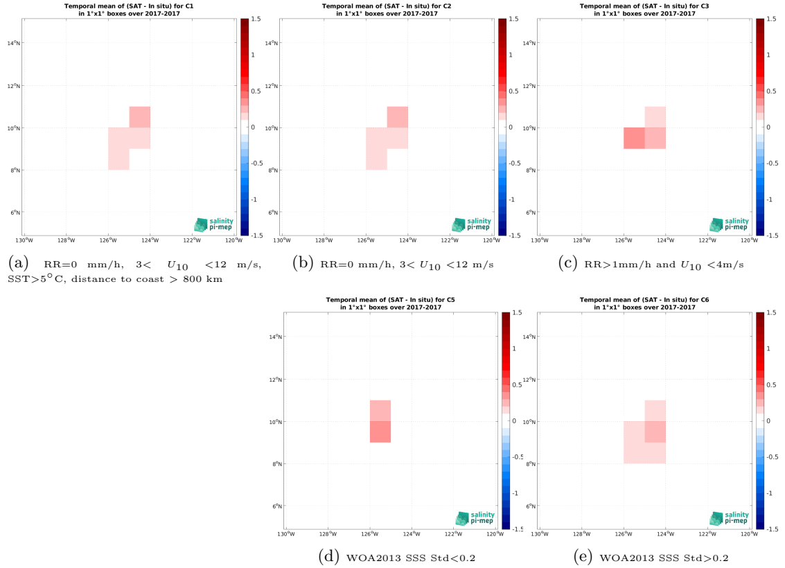
Figure 12: Temporal mean gridded over spatial boxes of size 1^{\circ}\times 1^{\circ} of \Delta\text{SSS} (SMOS SSS L3 v335 - 10 Days - 25 km (CATDS-CPDC) - Sailability (SPURS 2)) for 5 different subdatasets corresponding to: RR=0 mm/h, 3 < U_{10} < 12 m/s, SST > 5^{\circ}\text{C} , distance to coast > 800 km (a), RR=0 mm/h, 3 < U_{10} < 12 m/s (b), RR > 1 mm/h and U_{10} < 4 m/s (c), WOA2013 SSS Std < 0.2 (d), WOA2013 SSS Std > 0.2 (e).
