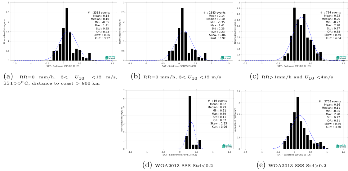
Figure 13: Normalized histogram of \Delta SSS (SMOS SSS L3 v335 - 10 Days - 25 km (CATDS-CPDC) - Saïldrone (SPURS 2)) for 5 different subdatasets corresponding to: RR=0 mm/h, 3 < U_{10} < 12 m/s, SST > 5°C, distance to coast > 800 km (a), RR=0 mm/h, 3 < U_{10} < 12 m/s (b), RR > 1mm/h and U_{10} < 4 m/s (c), WOA2013 SSS Std < 0.2 (d), WOA2013 SSS Std > 0.2 (e).
