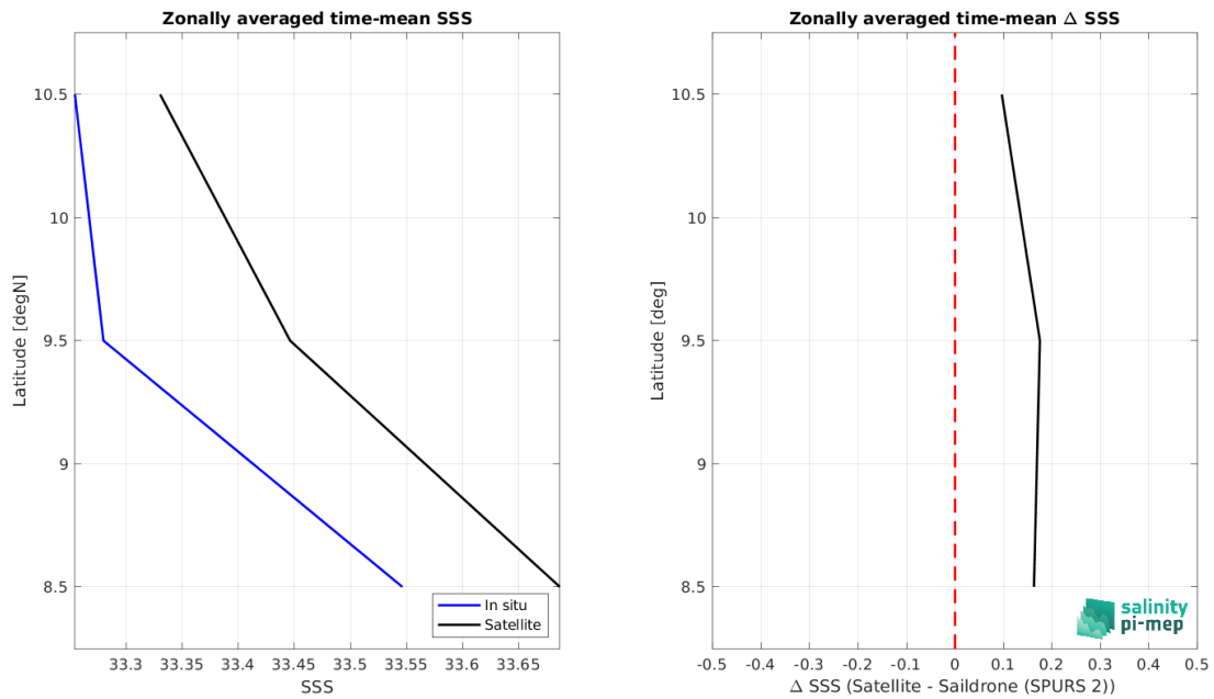
Figure 8: Left panel: Zonal mean SSS from SMOS SSS L3 v335 - 10 Days - 25 km (CATDS-CPDC) satellite product (black) and from Sairdron (SPURS 2) (blue). Right panel: Zonal mean of \Delta SSS (Satellite - Sairdron (SPURS 2)) for all the collected Pi-MEP match-up pairs estimated over the full satellite product period.
