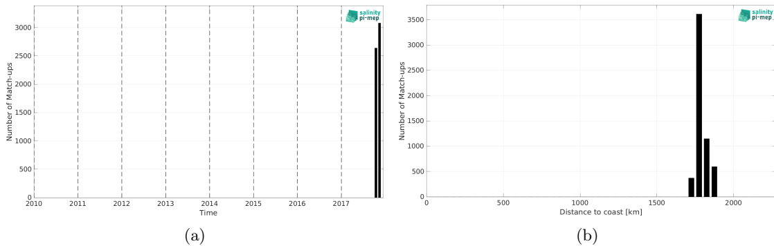
Figure 1: Number of match-ups between Saildrone (SPURS 2) and SMOS SSS L3 v335 - 10 Days - 25 km (CATDS-CPDC) SSS as a function of time (a) and as function of the distance to coast (b) over the SPURS 2 Pi-MEP region and for the full satellite product period.
