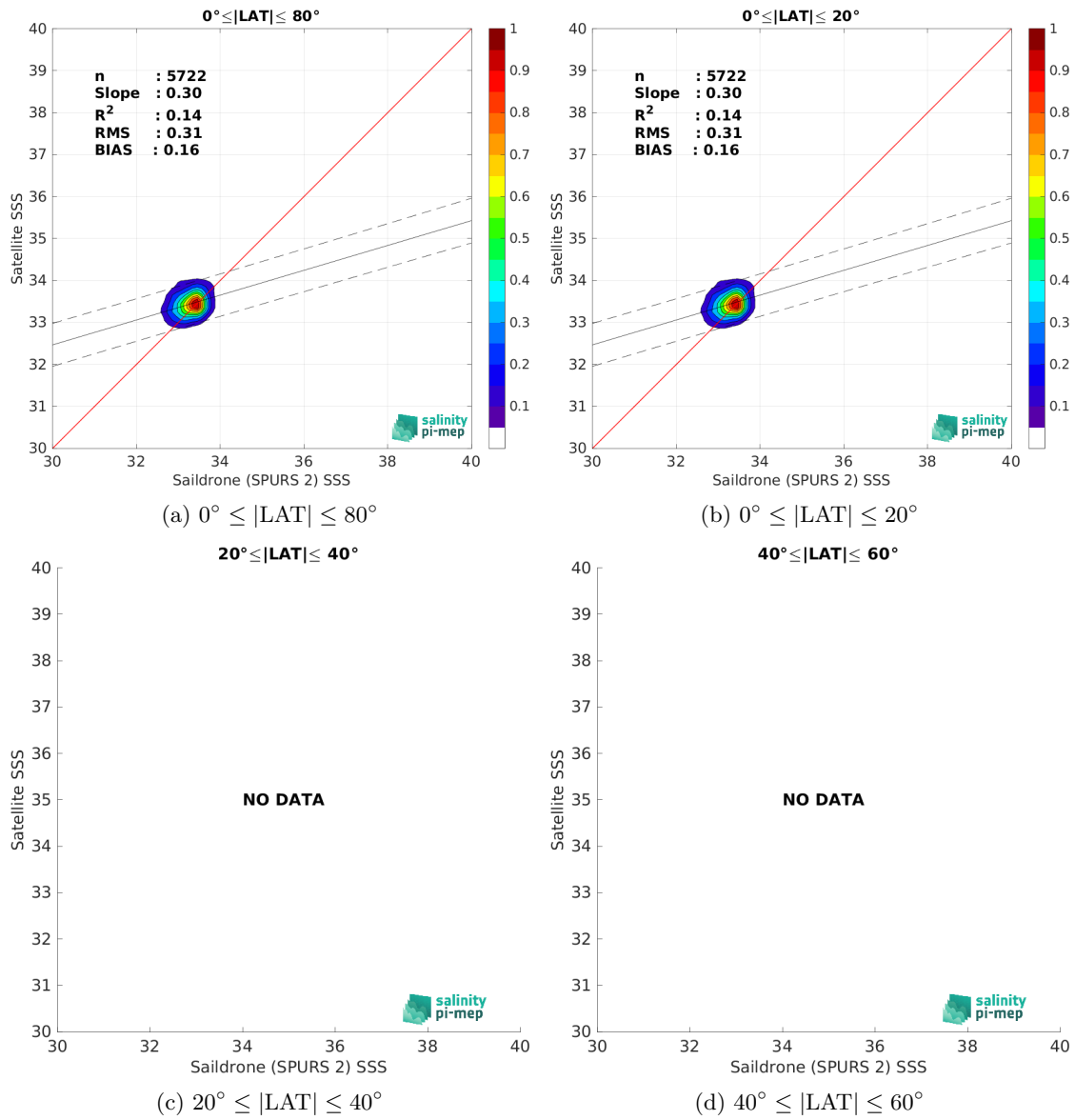
Figure 9: Contour maps of the concentration of SMOS SSS L3 v335 - 10 Days - 25 km (CATDS-CPDC) SSS (y-axis) versus Saildrone (SPURS 2) SSS (x-axis) at match-up pairs for different latitude bands. For each plot, the red line shows x=y . The black thin and dashed lines indicate a linear fit through the data cloud and the \pm 95\% confidence levels, respectively. The number match-up pairs n , the slope and R^2 coefficient of the linear fit, the root mean square (RMS) and the mean bias between satellite and in situ data are indicated for each latitude band in each plots.
