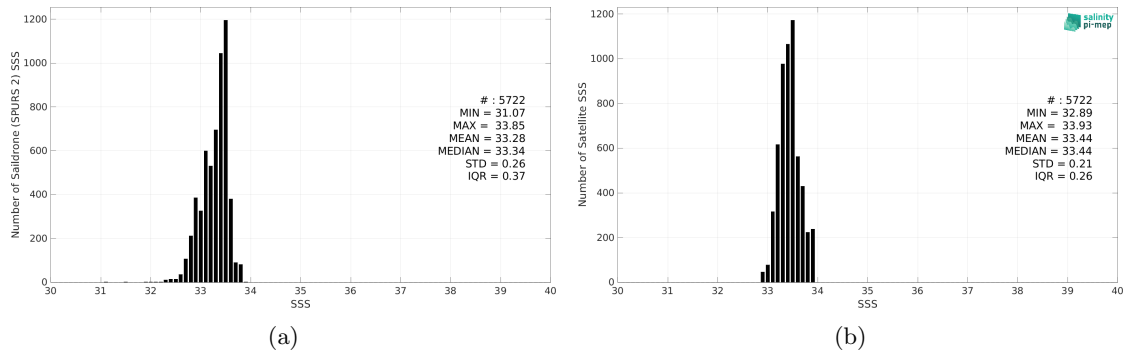
Figure 2: Histograms of SSS from Saildrone (SPURS 2) (a) and SMOS SSS L3 v335 - 10 Days - 25 km (CATDS-CPDC) (b) considering all match-up pairs per bins of 0.1 over the SPURS 2 Pi-MEP region and for the full satellite product period.
