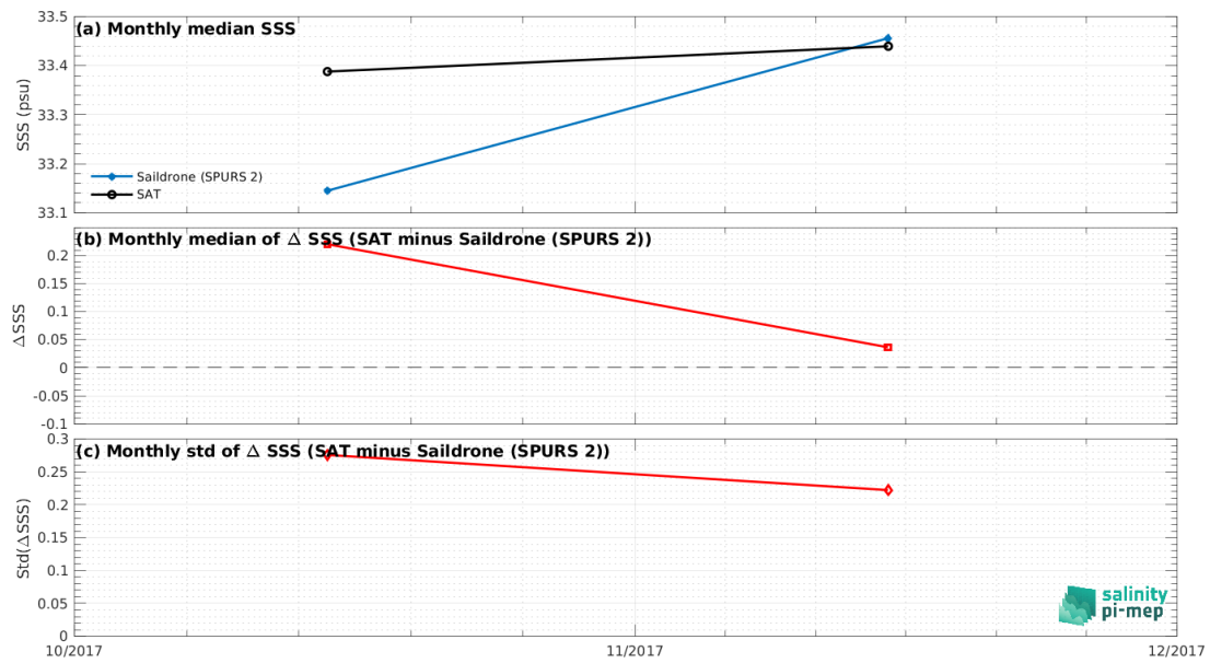
Figure 7: Time series of the monthly median SSS (top), median of \Delta SSS (Satellite - Sairdrone (SPURS 2)) and Std of \Delta SSS (Satellite - Sairdrone (SPURS 2)) over the SPURS 2 Pi-MEP region considering all match-ups collected by the Pi-MEP.
