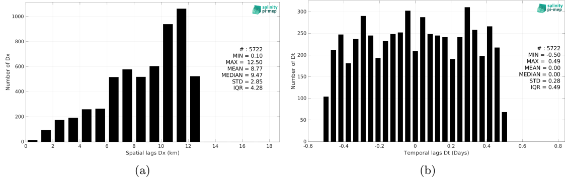
Figure 5: Histograms of the spatial (a) and temporal (b) lags between the location/time of the Saildrone (SPURS 2) measurement and the date of the corresponding SMOS SSS L3 v335 - 10 Days - 25 km (CATDS-CPDC) SSS pixel.
