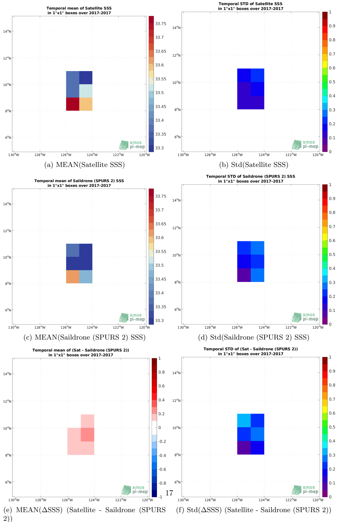
Figure 6: Temporal mean (left) and Std (right) of SSS from SMOS SSS L3 v335 - 10 Days - 25 km (CATDS-CPDC) (top), Saildrone (SPURS 2) (middle), and of \Delta SSS (Satellite - Saildrone (SPURS 2)). Only match-up pairs are used to generate these maps.
