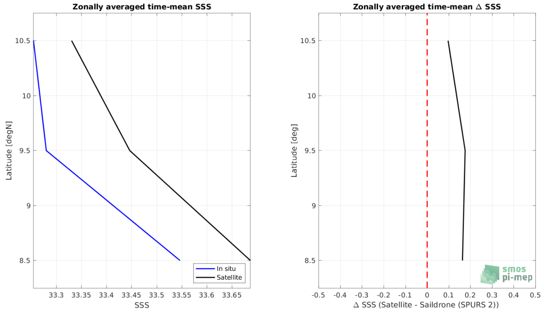
Figure 8: Left panel: Zonal mean SSS from SMOS SSS L3 v335 - 10 Days - 25 km (CATDS-CPDC) satellite product (black) and from Sairdrone (SPURS 2) (blue). Right panel: Zonal mean of \Delta SSS (Satellite - Sairdrone (SPURS 2)) for all the collected Pi-MEP match-up pairs estimated over the full satellite product period.
