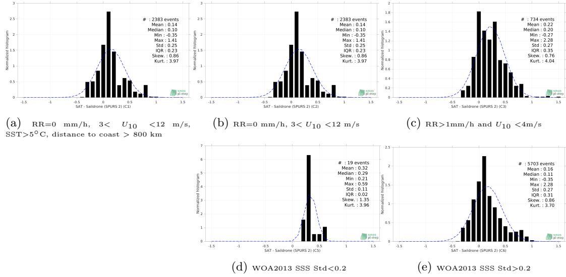
Figure 13: Normalized histogram of \Delta SSS (SMOS SSS L3 v335 - 10 Days - 25 km (CATDS-CPDC) - Saildrone (SPURS 2)) for 5 different subdatasets corresponding to: RR=0 mm/h, 3 < U_{10} < 12 m/s, SST > 5°C, distance to coast > 800 km (a), RR=0 mm/h, 3 < U_{10} < 12 m/s (b), RR > 1mm/h and U_{10} < 4 m/s (c), WOA2013 SSS Std < 0.2 (d), WOA2013 SSS Std > 0.2 (e).
