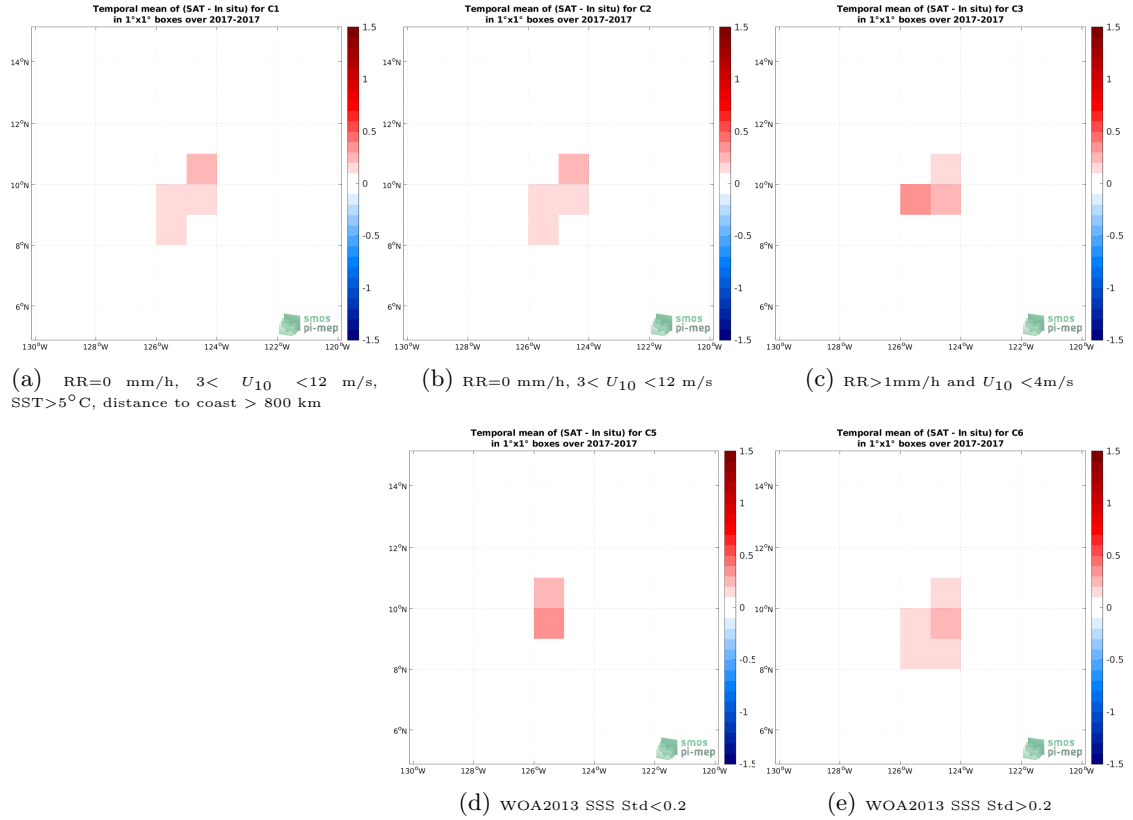
Figure 12: Temporal mean gridded over spatial boxes of size 1^{\circ}\times 1^{\circ} of \Delta\text{SSS} (SMOS SSS L3 v335 - 10 Days - 25 km (CATDS-CPDC) - Saldrone (SPURS 2)) for 5 different subdatasets corresponding to:RR=0 mm/h, 3 < U_{10} < 12 m/s, SST > 5^{\circ}\text{C} , distance to coast > 800 km (a), RR=0 mm/h, 3 < U_{10} < 12 m/s (b), RR > 1 mm/h and U_{10} < 4 m/s (c), WOA2013 SSS Std < 0.2 (d), WOA2013 SSS Std > 0.2 (e).
