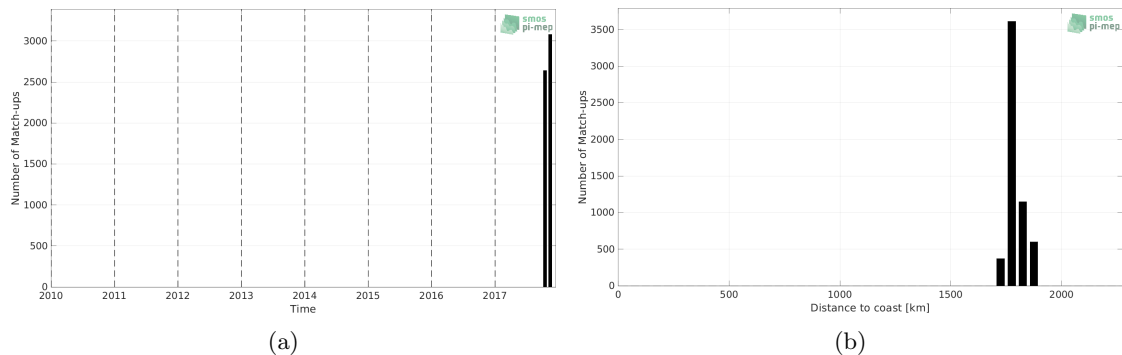
Figure 1: Number of match-ups between Sailldrone and SMOS SSS L3 v335 - 10 Days - 25 km (CATDS-CPDC) SSS as a function of time (a) and as function of the distance to coast (b) over the SPURS 2 Pi-MEP region and for the full satellite product period.
