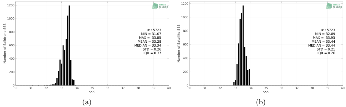
Figure 2: Histograms of SSS from Saïdrone (a) and SMOS SSS L3 v335 - 10 Days - 25 km (CATDS-CPDC) (b) considering all match-up pairs per bins of 0.1 over the SPURS 2 Pi-MEP region and for the full satellite product period.
