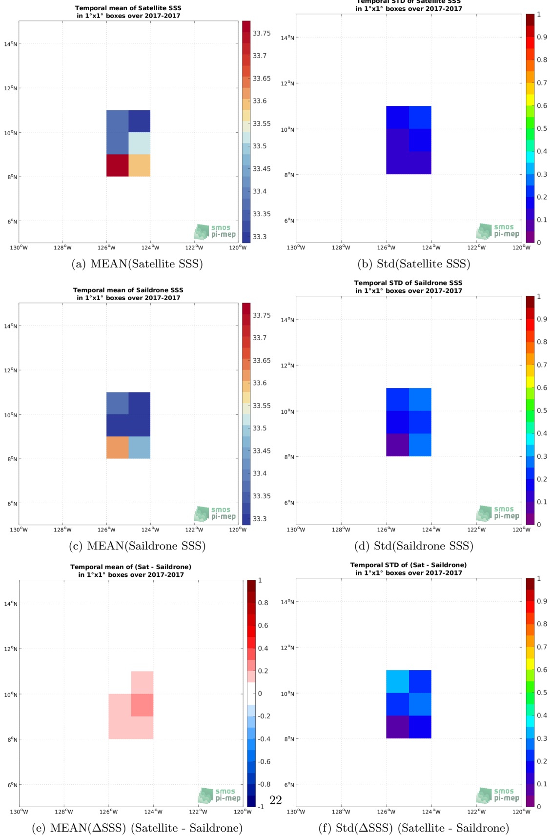
Figure 5: Temporal mean (left) and Std (right) of SSS from SMOS SSS L3 v335 - 10 Days - 25 km (CATDS-CPDC) (top), Saildrone (middle), and of \Delta SSS (Satellite - Saildrone). Only match-up pairs are used to generate these maps.
