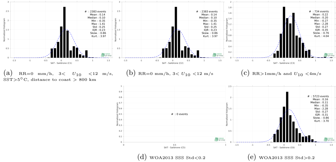
Figure 12: Normalized histogram of \Delta SSS (SMOS SSS L3 v335 - 10 Days - 25 km (CATDS-CPDC) - Sairdrone) for 5 different subdatasets corresponding to: RR=0 mm/h, 3 < U_{10} < 12 m/s, SST > 5°C, distance to coast > 800 km (a), RR=0 mm/h, 3 < U_{10} < 12 m/s (b), RR > 1mm/h and U_{10} < 4 m/s (c), WOA2013 SSS Std < 0.2 (d), WOA2013 SSS Std > 0.2 (e).
