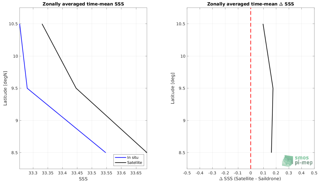
Figure 7: Left panel: Zonal mean SSS from SMOS SSS L3 v335 - 10 Days - 25 km (CATDS-CPDC) satellite product (black) and from Saildrone (blue). Right panel: Zonal mean of \Delta SSS (Satellite - Saildrone) for all the collected Pi-MEP match-up pairs estimated over the full satellite product period.
