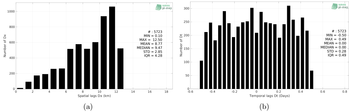
Figure 4: Histograms of the spatial (a) and temporal (b) lags between the location/time of the Saildrone measurement and the date of the corresponding SMOS SSS L3 v335 - 10 Days - 25 km (CATDS-CPDC) SSS pixel.
