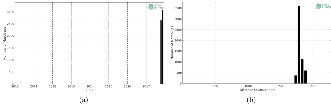
Figure 1: Number of match-ups between Saifdrone and SMOS SSS L3 v335 - 10 Days - 25 km (CATDS-CPDC) SSS as a function of time (a) and as function of the distance to coast (b) over the SPURS 2 Pi-MEP region and for the full satellite product period.
