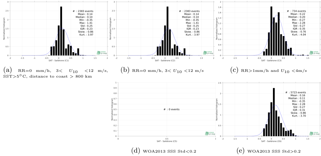
Figure 12: Normalized histogram of \Delta SSS (SMOS SSS L3 v335 - 10 Days - 25 km (CATDS-CPDC) - Saildrone) for 5 different subdatasets corresponding to: RR=0 mm/h, 3 < U_{10} < 12 m/s, SST > 5°C, distance to coast > 800 km (a), RR=0 mm/h, 3 < U_{10} < 12 m/s (b), RR > 1mm/h and U_{10} < 4 m/s (c), WOA2013 SSS Std < 0.2 (d), WOA2013 SSS Std > 0.2 (e).
