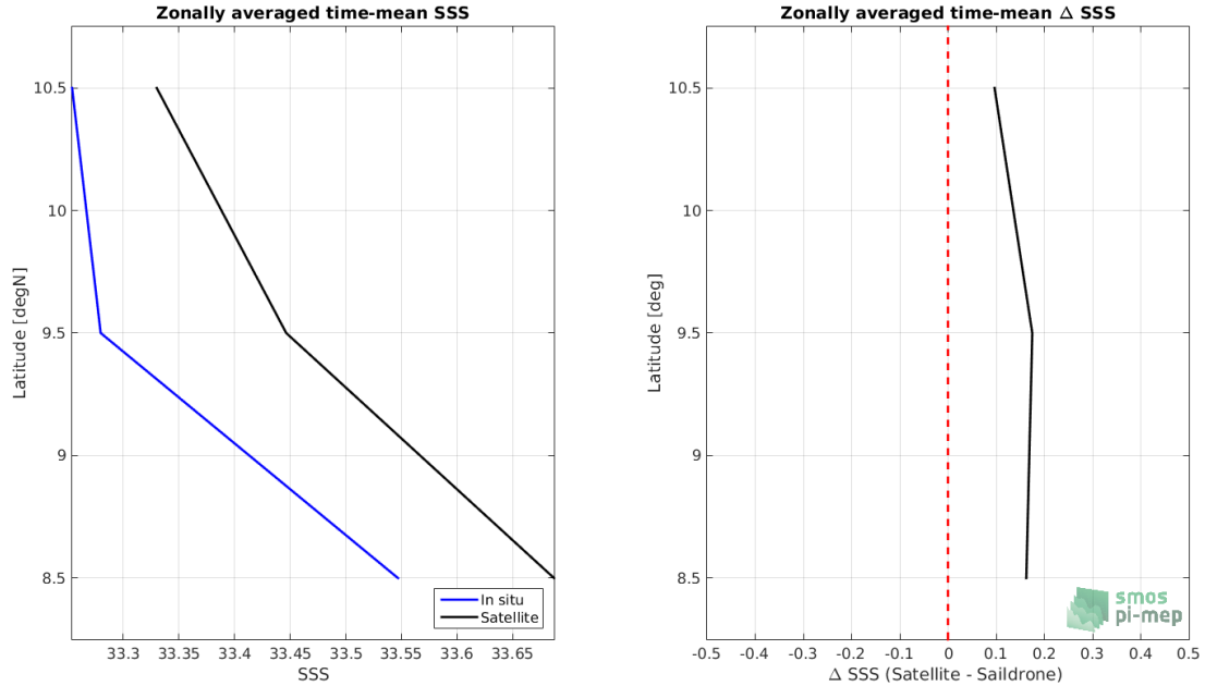
Figure 7: Left panel: Zonal mean SSS from SMOS SSS L3 v335 - 10 Days - 25 km (CATDS-CPDC) satellite product (black) and from Sairdrone (blue). Right panel: Zonal mean of \Delta SSS (Satellite - Sairdrone) for all the collected Pi-MEP match-up pairs estimated over the full satellite product period.
