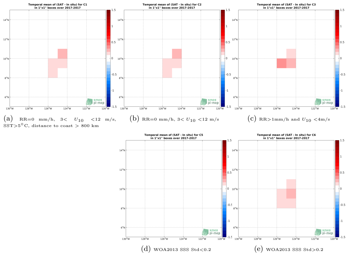
Figure 11: Temporal mean gridded over spatial boxes of size 1^\circ \times 1^\circ of \Delta SSS (SMOS SSS L3 v335 - 10 Days - 25 km (CATDS-CPDC) - Saildrone) for 5 different subdatasets corresponding to:RR=0 mm/h, 3 < U_{10} < 12 m/s, SST >5^\circ C, distance to coast > 800 km (a), RR=0 mm/h, 3 < U_{10} < 12 m/s (b), RR >1 mm/h and U_{10} < 4 m/s (c), WOA2013 SSS Std <0.2 (d), WOA2013 SSS Std >0.2 (e).
