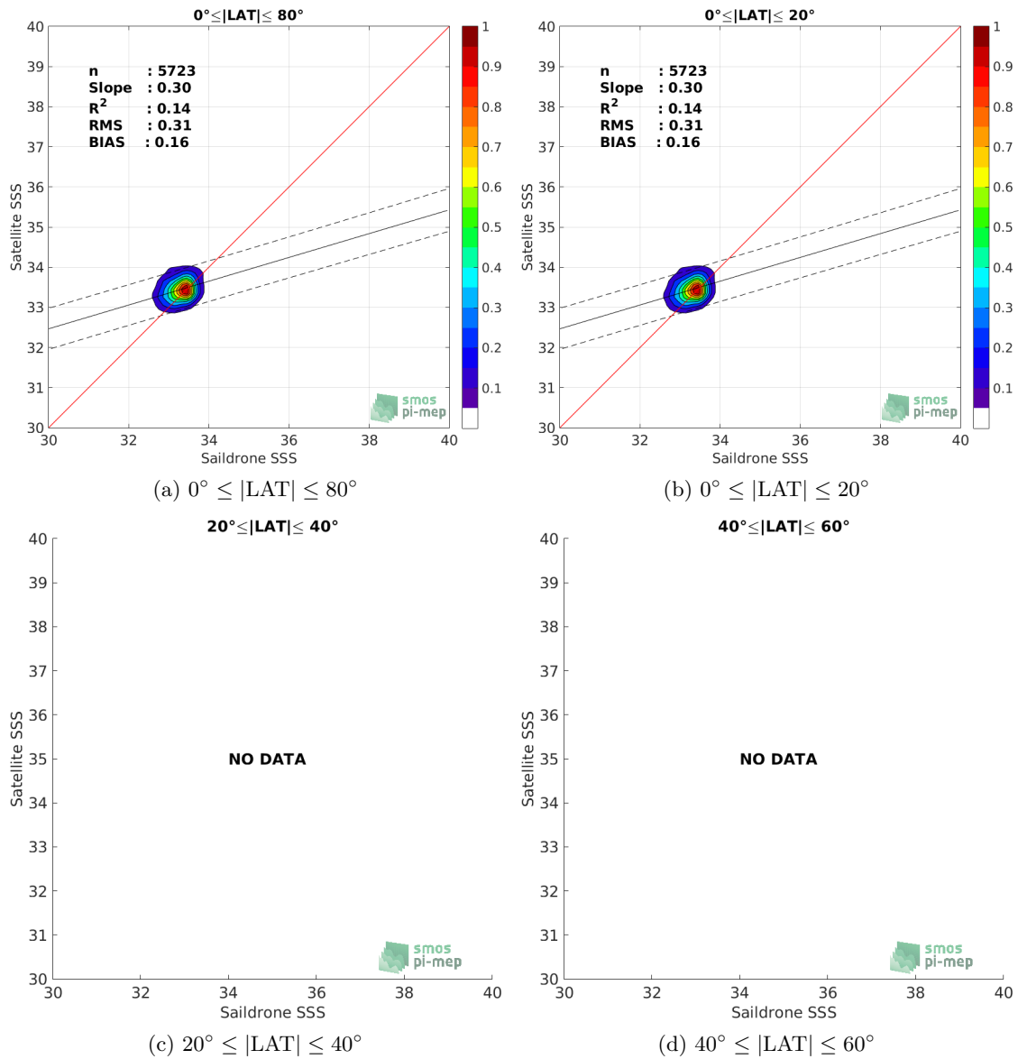
Figure 8: Contour maps of the concentration of SMOS SSS L3 v335 - 10 Days - 25 km (CATDS-CPDC) SSS (y-axis) versus SAILDRONE SSS (x-axis) at match-up pairs for different latitude bands. For each plot, the red line shows x=y . The black thin and dashed lines indicate a linear fit through the data cloud and the \pm 95\% confidence levels, respectively. The number match-up pairs n , the slope and R^2 coefficient of the linear fit, the root mean square (RMS) and the mean bias between satellite and in situ data are indicated for each latitude band in each plots.
