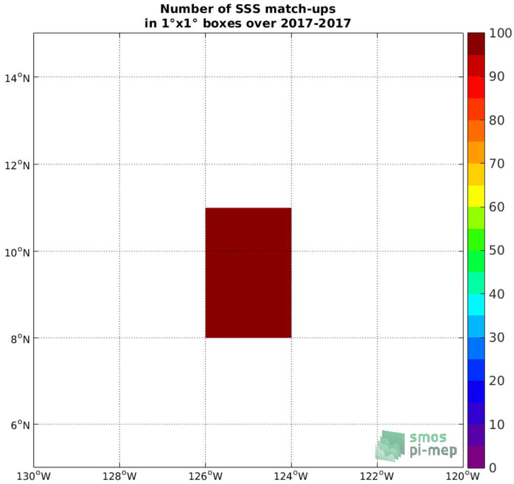
Figure 3: Number of SSS match-ups between Saildrone SSS and the SMOS SSS L3 v335 - 10 Days - 25 km (CATDS-CPDC) SSS product for the SPURS 2 Pi-MEP region over 1°×1° boxes and for the full satellite product period.
