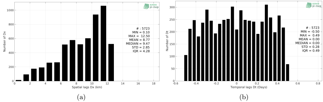
Figure 4: Histograms of the spatial (a) and temporal (b) lags between the location/time of the Sairdrone measurement and the date of the corresponding SMOS SSS L3 v335 - 10 Days - 25 km (CATDS-CPDC) SSS pixel.
