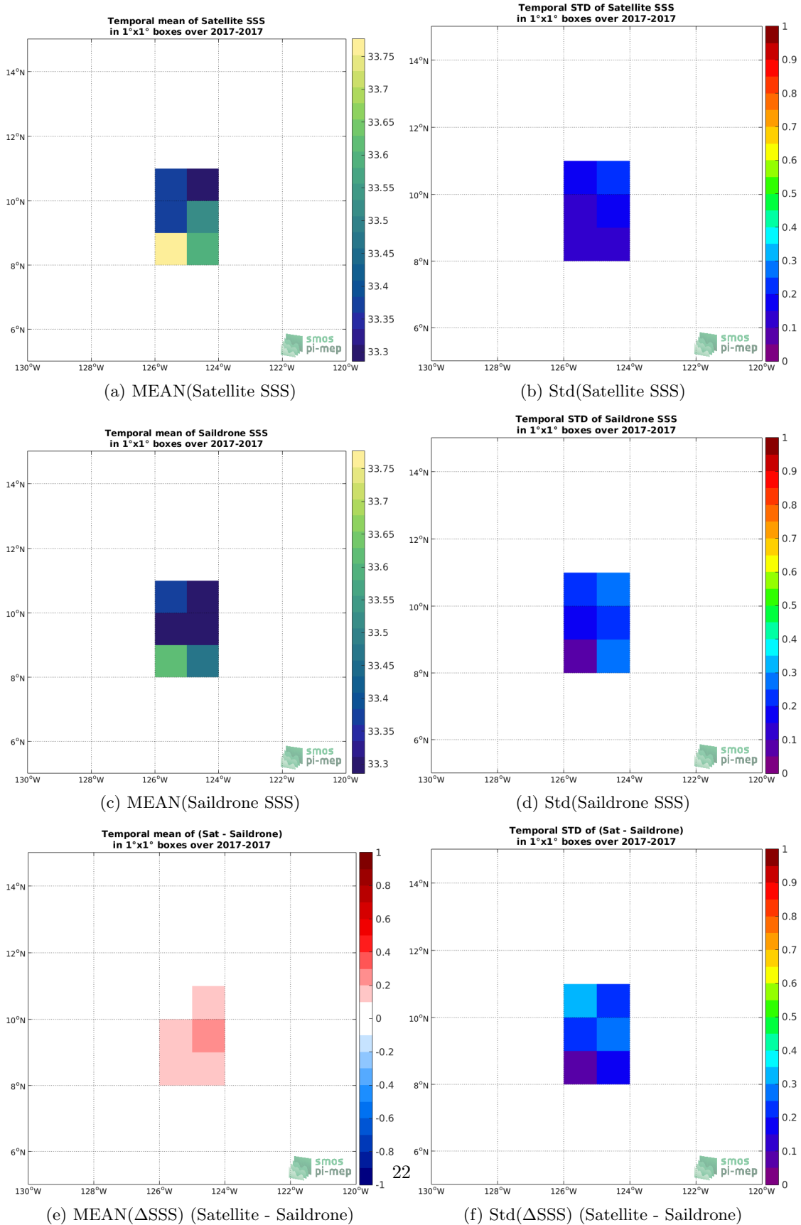
Figure 5: Temporal mean (left) and Std (right) of SSS from SMOS SSS L3 v335 - 10 Days - 25 km (CATDS-CPDC) (top), Saildrone (middle), and of \Delta SSS (Satellite - Saildrone). Only match-up pairs are used to generate these maps.
