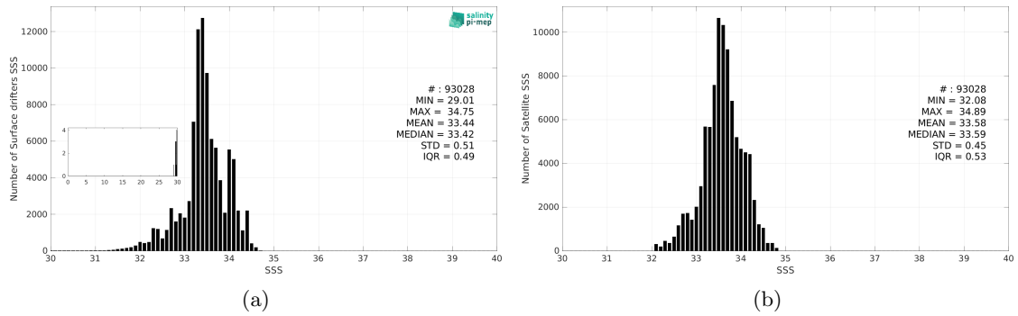
Figure 3: Histograms of SSS from Surface drifters (a) and SMOS SSS L3 v335 - 10 Days - 25 km (CATDS-CPDC) (b) considering all match-up pairs per bins of 0.1 over the SPURS 2 Pi-MEP region and for the full satellite product period.
