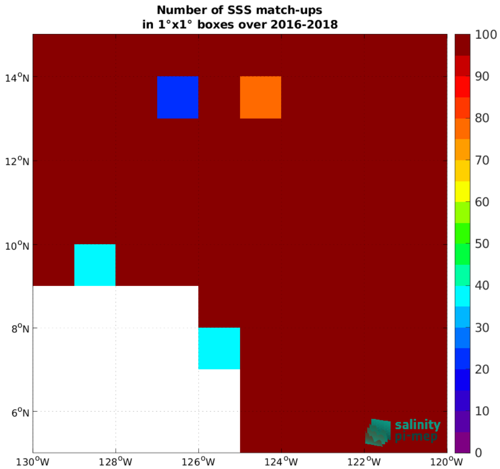
Figure 4: Number of SSS match-ups between Surface drifters SSS and the SMOS SSS L3 v335 - 10 Days - 25 km (CATDS-CPDC) SSS product for the SPURS 2 Pi-MEP region over 1°x1° boxes and for the full satellite product period.
