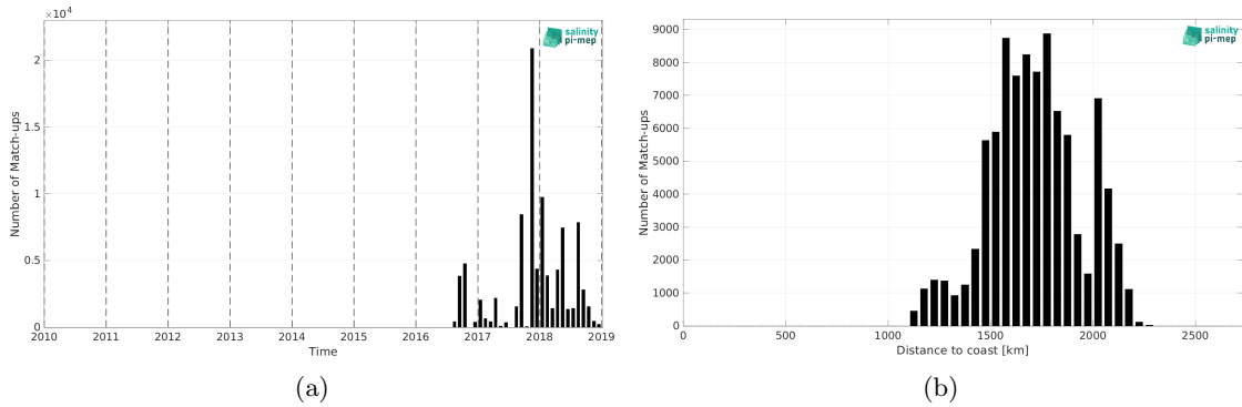
Figure 2: Number of match-ups between Surface drifters and SMOS SSS L3 v335 - 10 Days - 25 km (CATDS-CPDC) SSS as a function of time (a) and as function of the distance to coast (b) over the SPURS 2 Pi-MEP region and for the full satellite product period.
