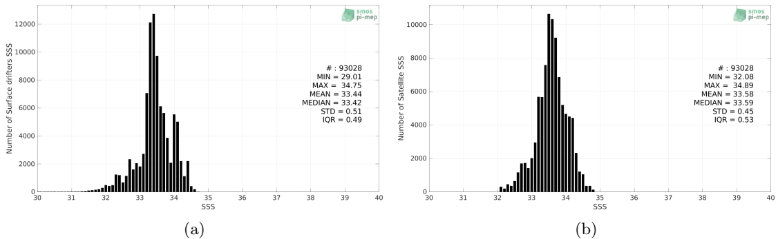
Figure 2: Histograms of SSS from Surface drifters (a) and SMOS SSS L3 v335 - 10 Days - 25 km (CATDS-CPDC) (b) considering all match-up pairs per bins of 0.1 over the SPURS 2 Pi-MEP region and for the full satellite product period.
