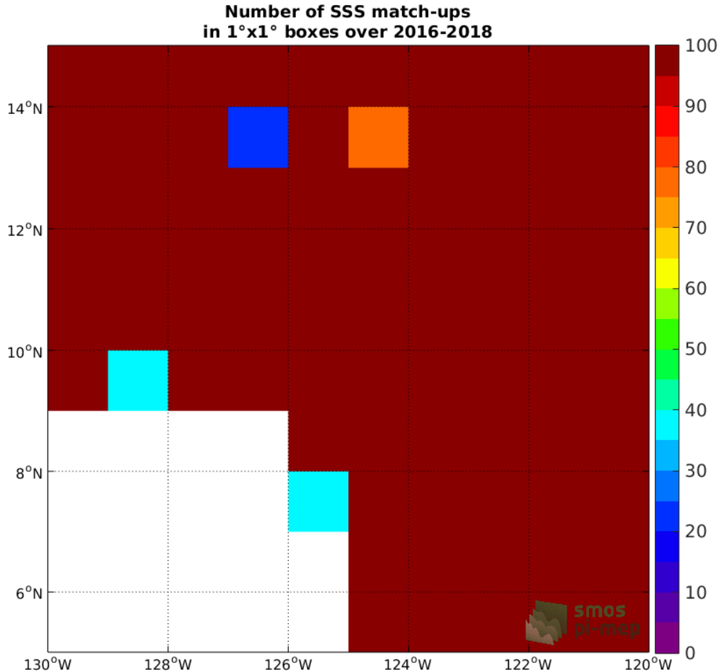
Figure 3: Number of SSS match-ups between Surface drifters SSS and the SMOS SSS L3 v335 - 10 Days - 25 km (CATDS-CPDC) SSS product for the SPURS 2 Pi-MEP region over 1^\circ \times 1^\circ boxes and for the full satellite product period.
