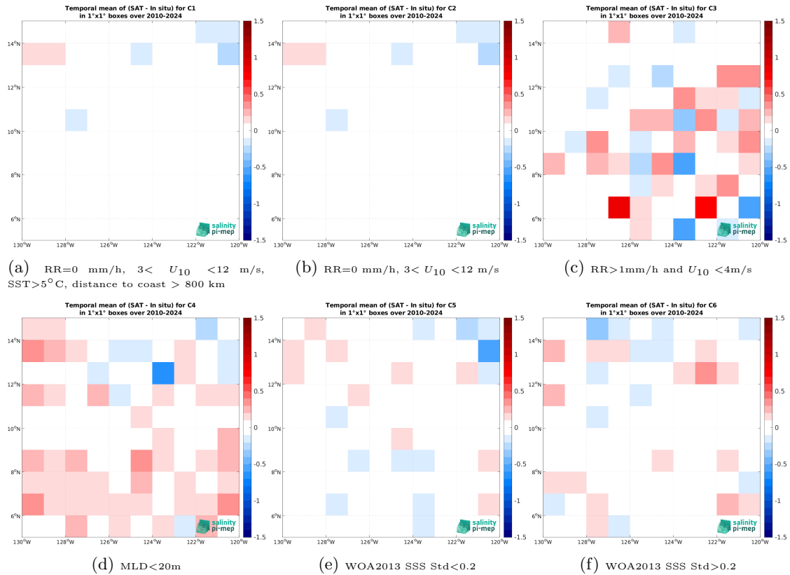
Figure 14: Temporal mean gridded over spatial boxes of size 1^\circ \times 1^\circ of \Delta SSS (SMOS SSS L3 v335 - 10 Days - 25 km (CATDS-CPDC) - Argo) for 6 different subdatasets corresponding to: RR=0 mm/h, 3 < U_{10} < 12 m/s, SST > 5^\circ\text{C} , distance to coast > 800 km (a), RR=0 mm/h, 3 < U_{10} < 12 m/s (b), RR > 1 mm/h and U_{10} < 4 m/s (c), MLD < 20 m (d), WOA2013 SSS Std < 0.2 (e), WOA2013 SSS Std > 0.2 (f).
