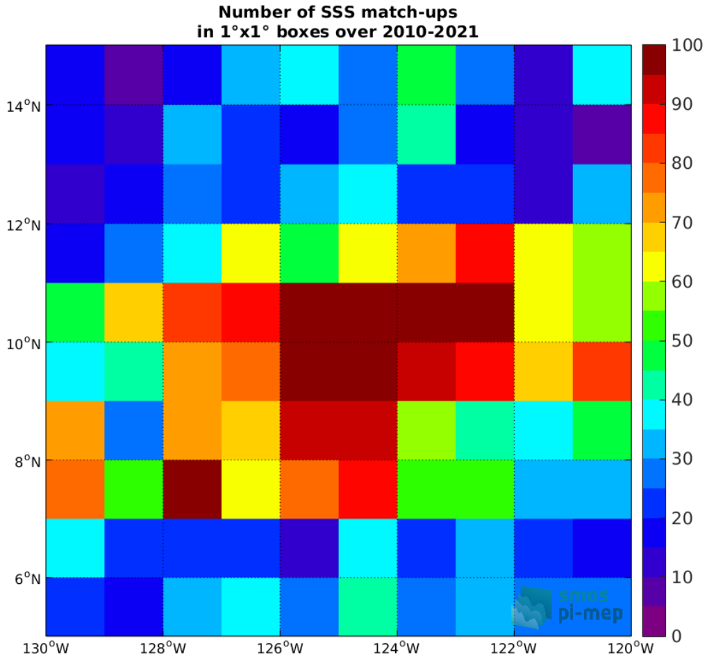
Figure 4: Number of SSS match-ups between Argo SSS and the SMOS SSS L3 v335 - 10 Days - 25 km (CATDS-CPDC) SSS product for the SPURS 2 Pi-MEP region over 1°×1° boxes and for the full satellite product period.
