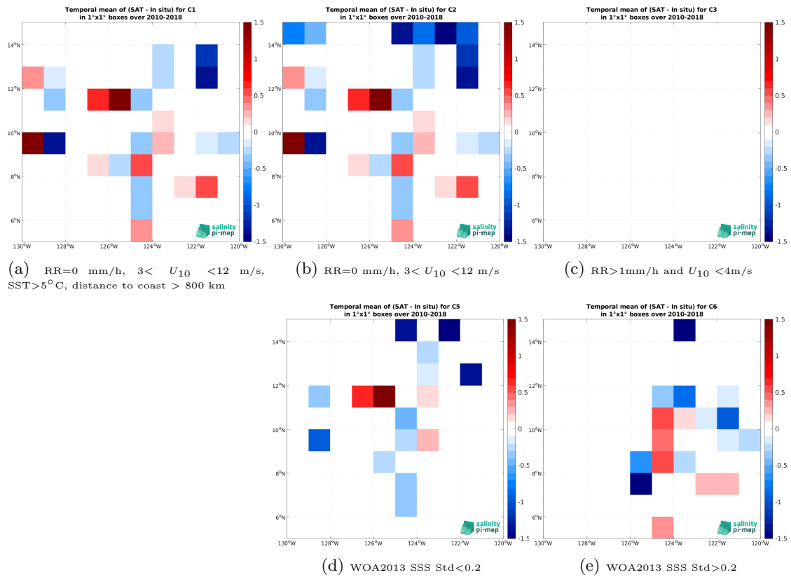
Figure 14: Temporal mean gridded over spatial boxes of size 1^\circ \times 1^\circ of \Delta SSS (SMOS SSS L2Q v333 - 0.25 Deg (CATDS-CPDC) - TSG (SAMOS)) for 5 different subdatasets corresponding to: RR=0 mm/h, 3 < U_{10} < 12 m/s, SST > 5°C, distance to coast > 800 km (a), RR=0 mm/h, 3 < U_{10} < 12 m/s (b), RR > 1mm/h and U_{10} < 4 m/s (c), WOA2013 SSS Std < 0.2 (d), WOA2013 SSS Std > 0.2 (e).
