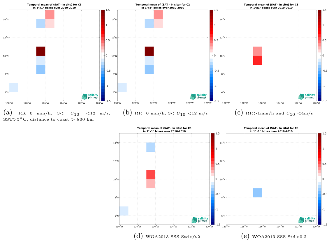
Figure 14: Temporal mean salinity gridded over spatial boxes of size 1^\circ \times 1^\circ of \Delta\text{SSS} (SMOS SSS L2Q v333 - 0.25 Deg (CATDS-CPDC) - TSG (GOSUD-Sailing-ship)) for 5 different subdatasets corresponding to:RR=0 mm/h, 3 < U_{10} < 12 m/s, SST>5°C, distance to coast > 800 km (a), RR=0 mm/h, 3 < U_{10} < 12 m/s (b), RR>1mm/h and U_{10} < 4 m/s (c), WOA2013 SSS Std<0.2 (d), WOA2013 SSS Std>0.2 (e).
