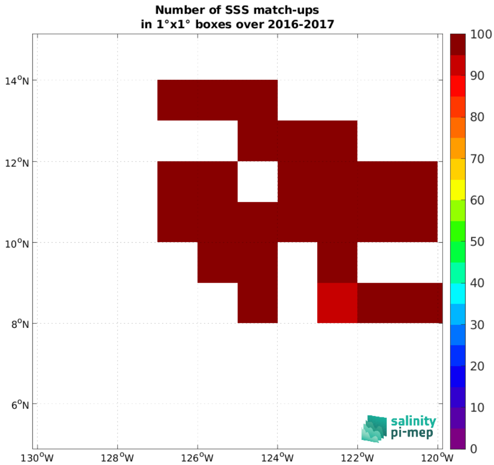
Figure 5: Number of SSS match-ups between Waveglider (SPURS 2) SSS and the SMOS SSS L3 v332 - 9 Days (CATDS-CPDC) SSS product for the SPURS 2 Pi-MEP region over 1°x1° boxes and for the full satellite product period.
