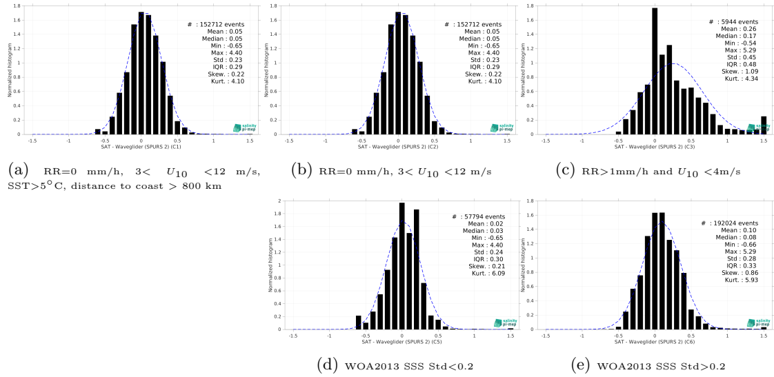
Figure 15: Normalized histogram of \Delta\text{SSS} (SMOS SSS L3 v332 - 9 Days (CATDS-CPDC) - Waveglider (SPURS 2)) for 5 different subdatasets corresponding to: RR=0 mm/h, 3 < U_{10} < 12 m/s, SST >5^{\circ}\text{C} , distance to coast > 800 km (a), RR=0 mm/h, 3 < U_{10} < 12 m/s (b), RR >1 mm/h and U_{10} < 4 m/s (c), WOA2013 SSS Std <0.2 (d), WOA2013 SSS Std >0.2 (e).
