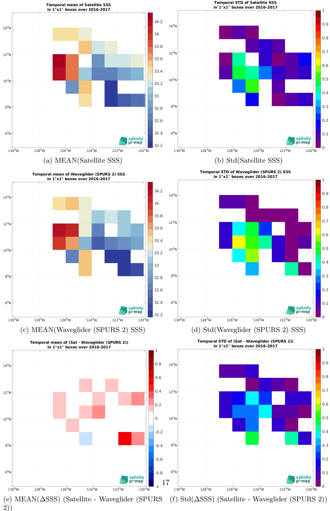
Figure 7: Temporal mean (left) and Std (right) of SSS from SMOS SSS L3 v332 - 9 Days (CATDS-CPDC) (top), Waveglider (SPURS 2) (middle), and of \Delta SSS (Satellite - Waveglider (SPURS 2)). Only match-up pairs are used to generate these maps.
