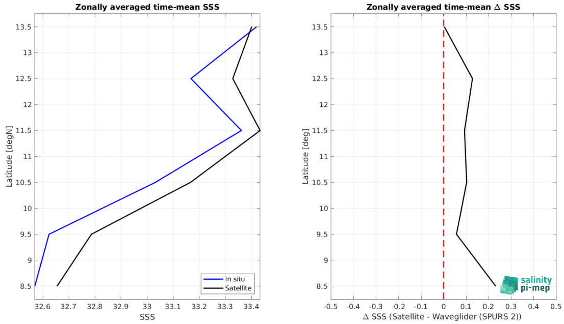
Figure 9: Left panel: Zonal mean SSS from SMOS SSS L3 v332 - 9 Days (CATDS-CPDC) satellite product (black) and from Waveglider (SPURS 2) (blue). Right panel: Zonal mean of \Delta SSS (Satellite - Waveglider (SPURS 2)) for all the collected Pi-MEP match-up pairs estimated over the full satellite product period.
