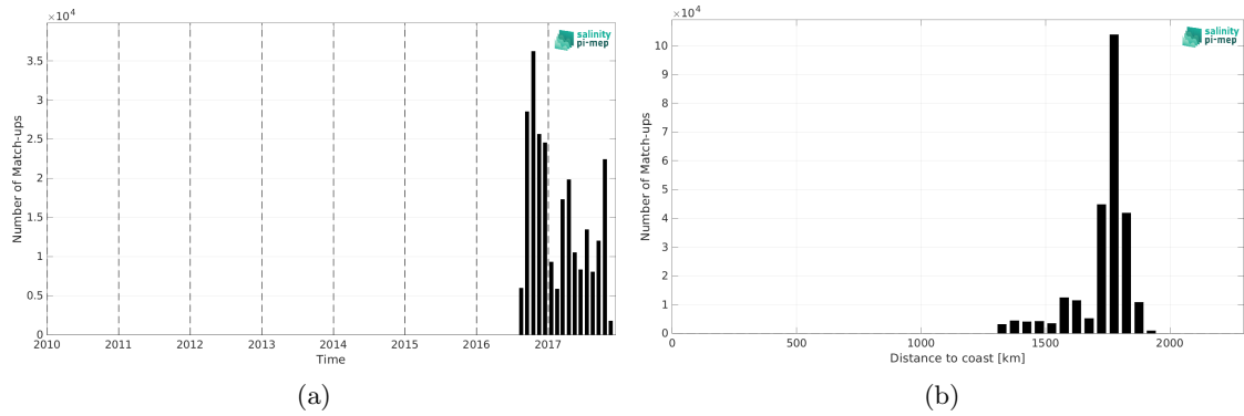
Figure 2: Number of match-ups between Waveglider (SPURS 2) and SMOS SSS L3 v332 - 9 Days (CATDS-CPDC) SSS as a function of time (a) and as function of the distance to coast (b) over the SPURS 2 Pi-MEP region and for the full satellite product period.
