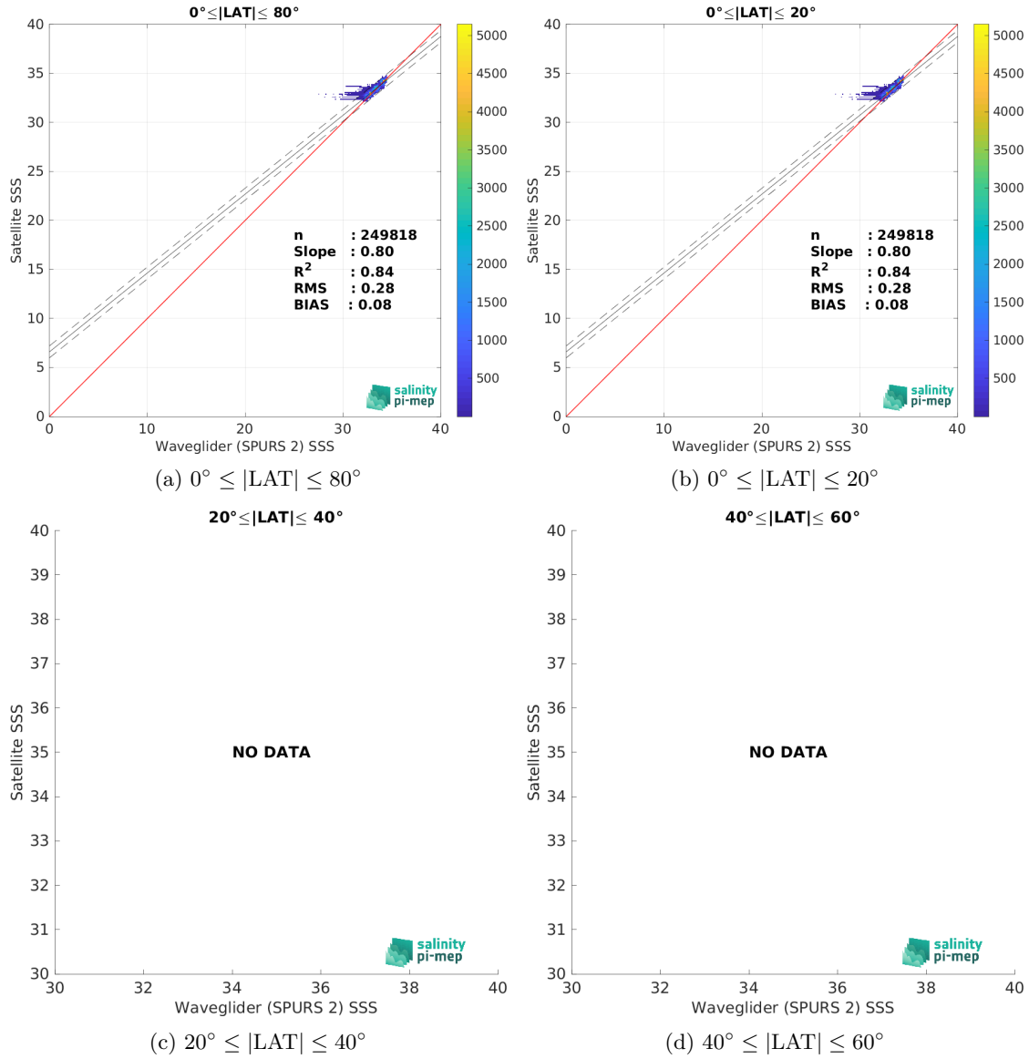
Figure 10: Contour maps of the concentration of SMOS SSS L3 v332 - 9 Days (CATDS-CPDC) SSS (y-axis) versus Waveglider (SPURS 2) SSS (x-axis) at match-up pairs for different latitude bands. For each plot, the red line shows x=y . The black thin and dashed lines indicate a linear fit through the data cloud and the \pm 95\% confidence levels, respectively. The number match-up pairs n , the slope and R^2 coefficient of the linear fit, the root mean square (RMS) and the mean bias between satellite and in situ data are indicated for each latitude band in each plots.
