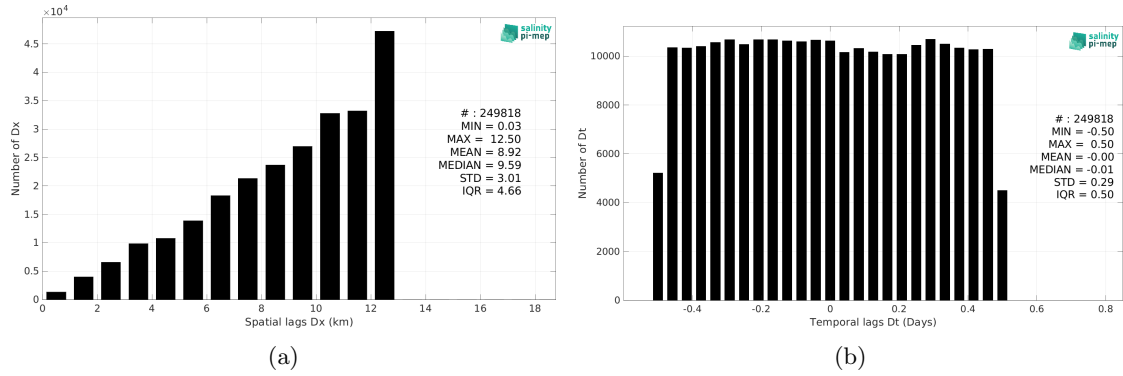
Figure 6: Histograms of the spatial (a) and temporal (b) lags between the location/time of the Waveglider (SPURS 2) measurement and the date of the corresponding SMOS SSS L3 v332 - 9 Days (CATDS-CPDC) SSS pixel.
