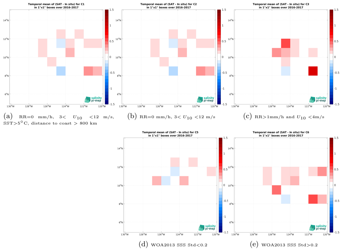
Figure 14: Temporal mean gridded over spatial boxes of size 1^\circ \times 1^\circ of \Delta\text{SSS} (SMOS SSS L3 v332 - 9 Days (CATDS-CPDC) - Waveglider (SPURS 2)) for 5 different subdatasets corresponding to:RR=0 mm/h, 3 < U_{10} < 12 m/s, SST>5°C, distance to coast > 800 km (a), RR=0 mm/h, 3 < U_{10} < 12 m/s (b), RR>1mm/h and U_{10} < 4 m/s (c), WOA2013 SSS Std<0.2 (d), WOA2013 SSS Std>0.2 (e).
