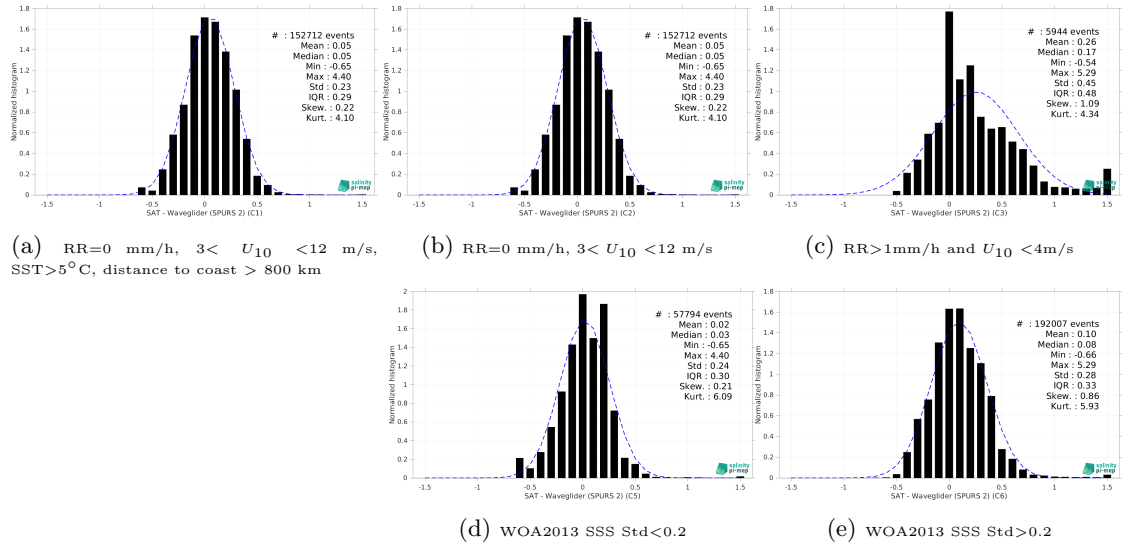
Figure 15: Normalized histogram of \Delta SSS (SMOS SSS L3 v332 - 9 Days (CATDS-CPDC) - Waveglider (SPURS 2)) for 5 different subdatasets corresponding to: RR=0 mm/h, 3 < U_{10} < 12 m/s, SST > 5°C, distance to coast > 800 km (a), RR=0 mm/h, 3 < U_{10} < 12 m/s (b), RR > 1mm/h and U_{10} < 4 m/s (c), WOA2013 SSS Std < 0.2 (d), WOA2013 SSS Std > 0.2 (e).
