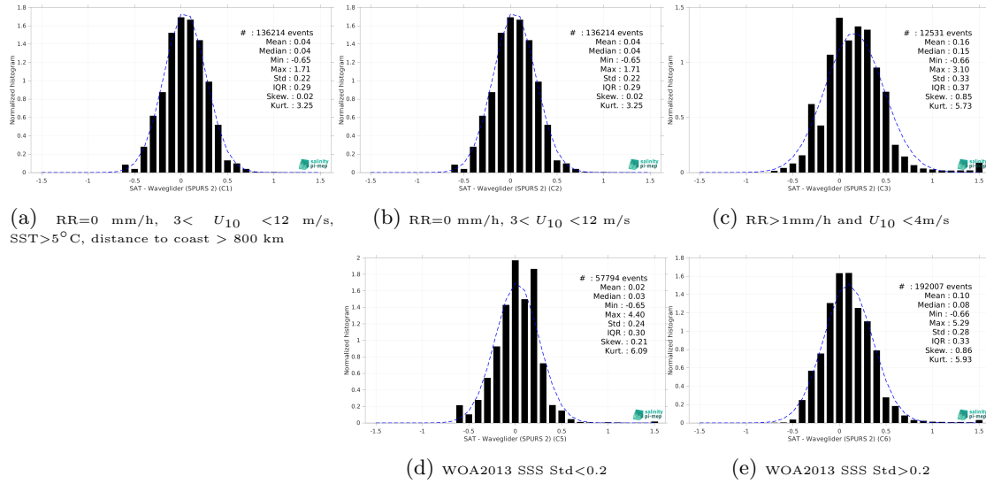
Figure 13: Normalized histogram of \Delta SSS (SMOS SSS L3 v332 - 9 Days (CATDS-CPDC) - Waveglider (SPURS 2)) for 5 different subdatasets corresponding to: RR=0 mm/h, 3 < U_{10} < 12 m/s, SST > 5°C, distance to coast > 800 km (a), RR=0 mm/h, 3 < U_{10} < 12 m/s (b), RR > 1mm/h and U_{10} < 4 m/s (c), WOA2013 SSS Std < 0.2 (d), WOA2013 SSS Std > 0.2 (e).
