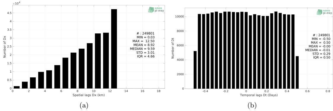
Figure 5: Histograms of the spatial (a) and temporal (b) lags between the location/time of the Waveglider (SPURS 2) measurement and the date of the corresponding SMOS SSS L3 v332 - 9 Days (CATDS-CPDC) SSS pixel.
