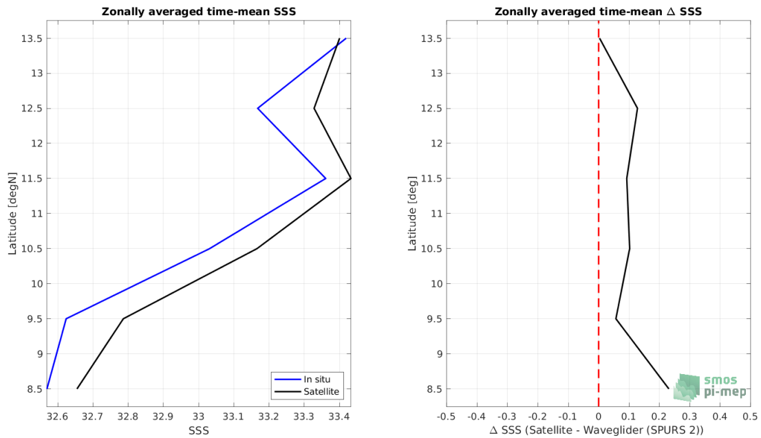
Figure 8: Left panel: Zonal mean SSS from SMOS SSS L3 v332 - 9 Days (CATDS-CPDC) satellite product (black) and from Waveglider (SPURS 2) (blue). Right panel: Zonal mean of \Delta SSS (Satellite - Waveglider (SPURS 2)) for all the collected Pi-MEP match-up pairs estimated over the full satellite product period.
