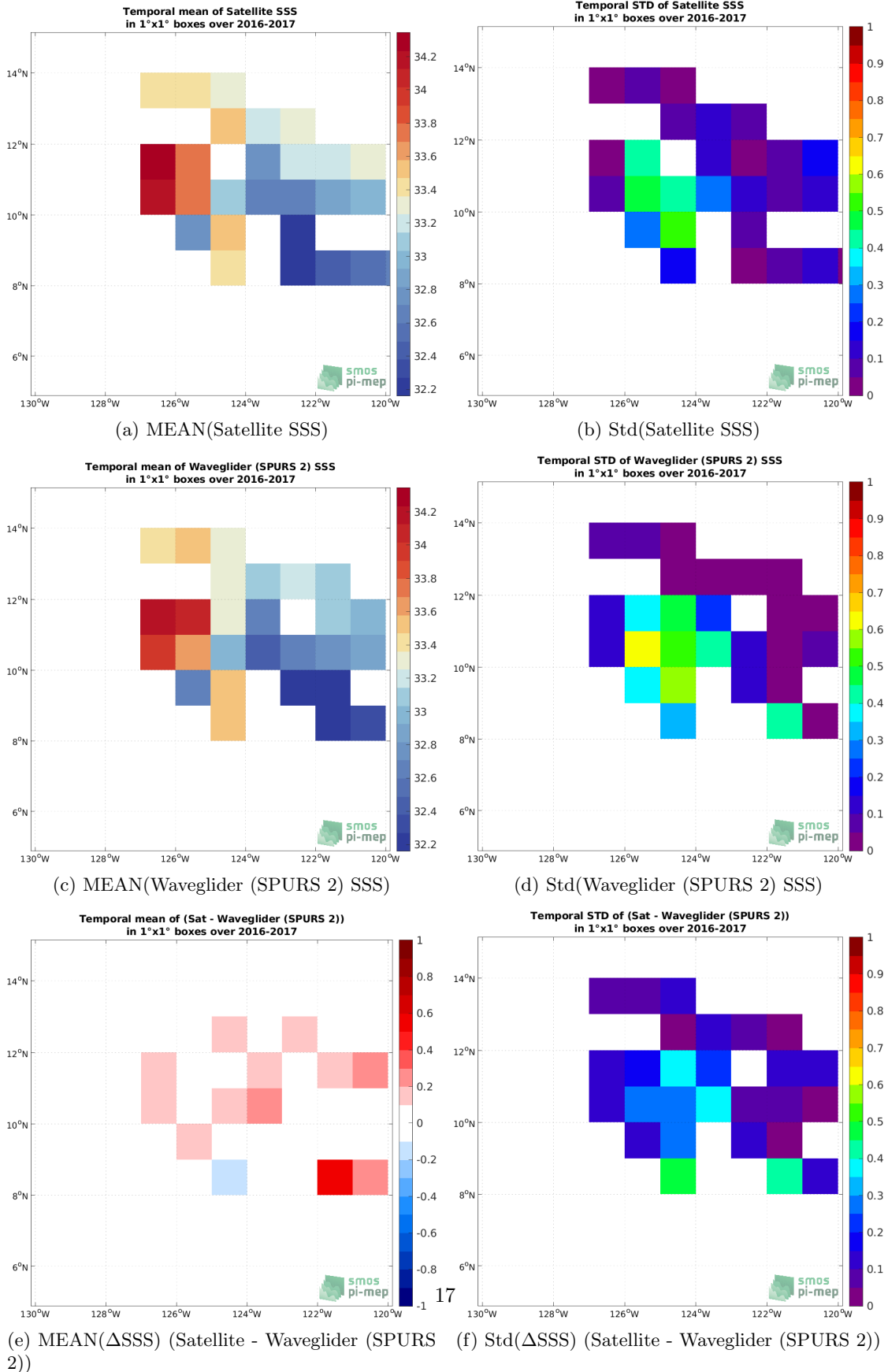
Figure 6: Temporal mean (left) and Std (right) of SSS from SMOS SSS L3 v332 - 9 Days (CATDS-CPDC) (top), Waveglider (SPURS 2) (middle), and of \Delta SSS (Satellite - Waveglider (SPURS 2)). Only match-up pairs are used to generate these maps.
