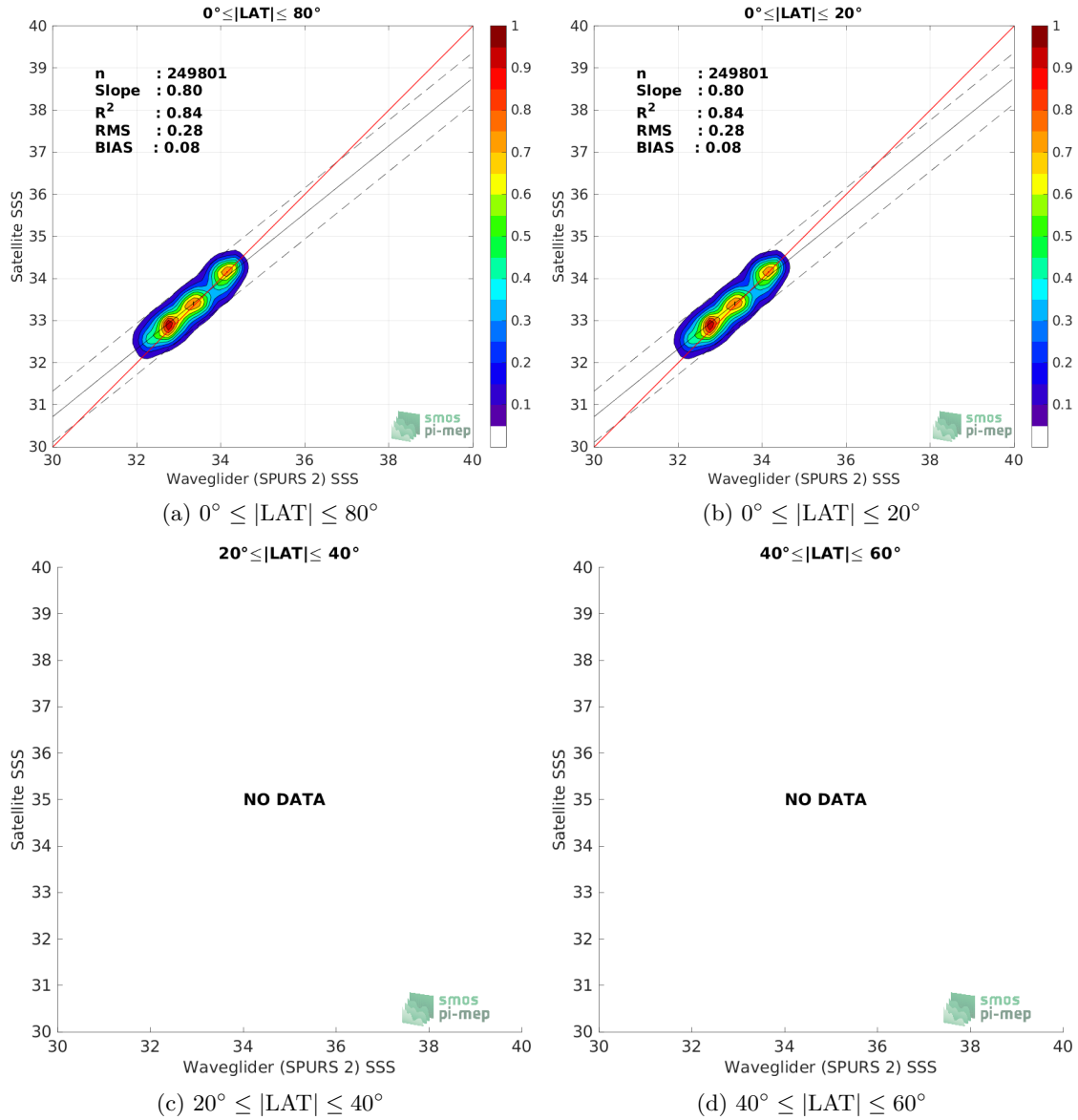
Figure 9: Contour maps of the concentration of SMOS SSS L3 v332 - 9 Days (CATDS-CPDC) SSS (y-axis) versus Waveglider (SPURS 2) SSS (x-axis) at match-up pairs for different latitude bands. For each plot, the red line shows x=y . The black thin and dashed lines indicate a linear fit through the data cloud and the \pm 95\% confidence levels, respectively. The number match-up pairs n , the slope and R^2 coefficient of the linear fit, the root mean square (RMS) and the mean bias between satellite and in situ data are indicated for each latitude band in each plots.
