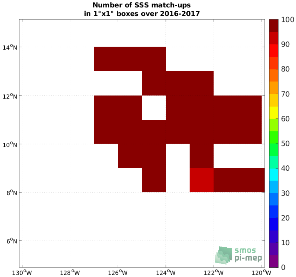
Figure 4: Number of SSS match-ups between Waveglider (SPURS 2) SSS and the SMOS SSS L3 v332 - 9 Days (CATDS-CPDC) SSS product for the SPURS 2 Pi-MEP region over 1^\circ \times 1^\circ boxes and for the full satellite product period.
