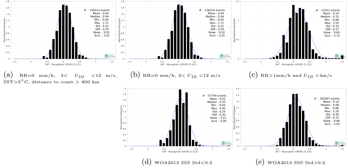
Figure 13: Normalized histogram of \Delta SSS (SMOS SSS L3 v332 - 9 Days (CATDS-CPDC) - Waveglider (SPURS 2)) for 5 different subdatasets corresponding to: RR=0 mm/h, 3 < U_{10} < 12 m/s, SST > 5°C, distance to coast > 800 km (a), RR=0 mm/h, 3 < U_{10} < 12 m/s (b), RR > 1mm/h and U_{10} < 4 m/s (c), WOA2013 SSS Std < 0.2 (d), WOA2013 SSS Std > 0.2 (e).
