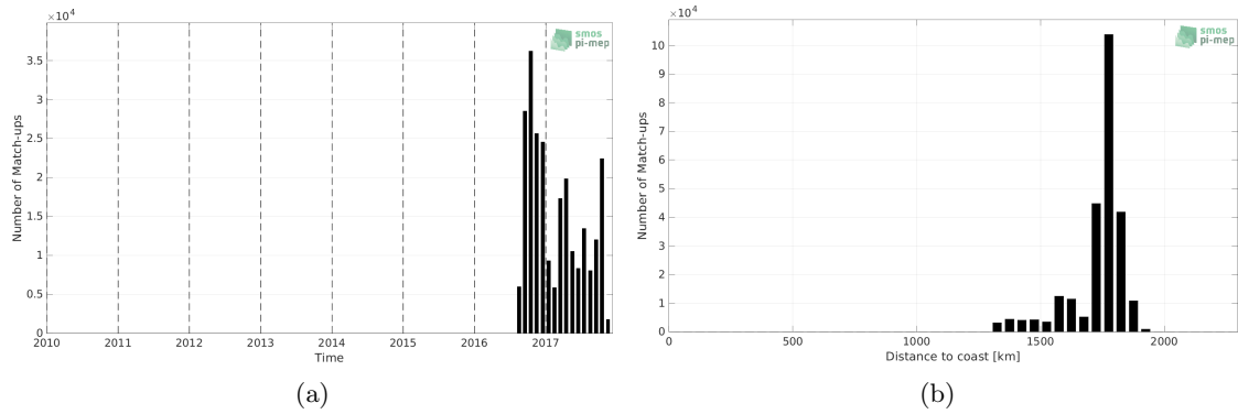
Figure 1: Number of match-ups between Waveglider (SPURS 2) and SMOS SSS L3 v332 - 9 Days (CATDS-CPDC) SSS as a function of time (a) and as function of the distance to coast (b) over the SPURS 2 Pi-MEP region and for the full satellite product period.
