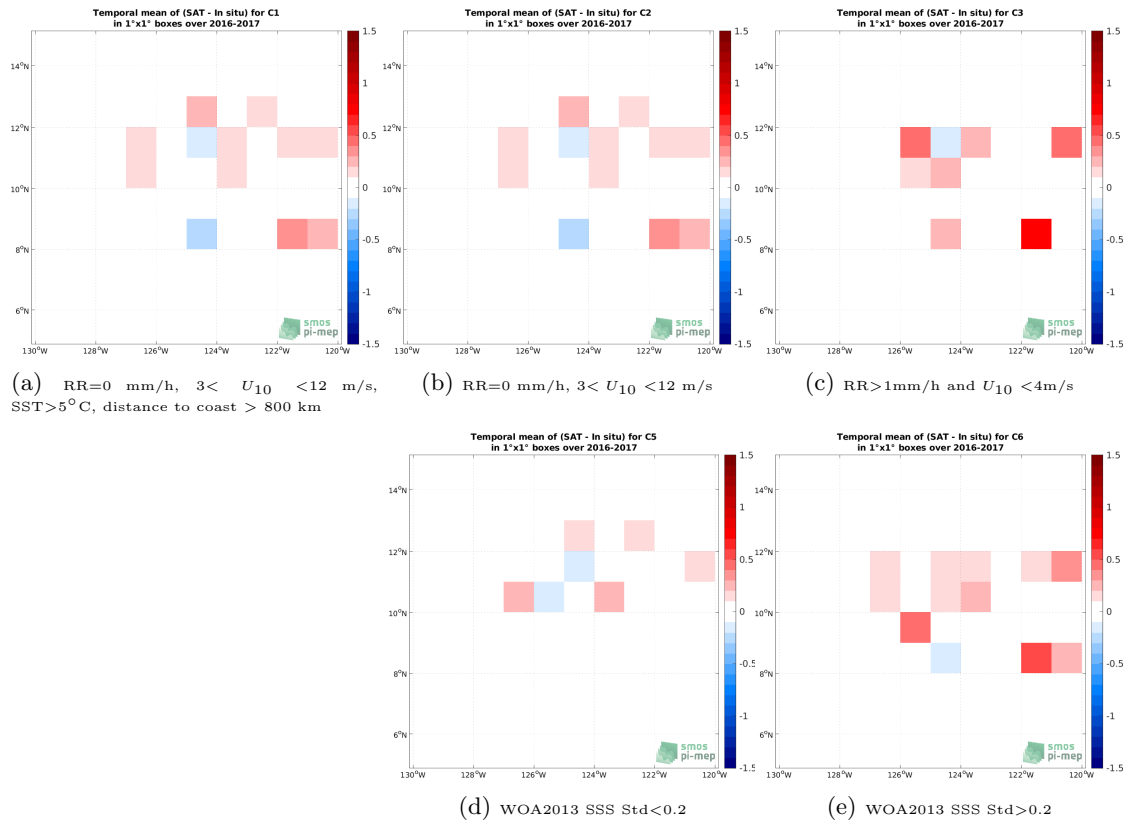
Figure 12: Temporal mean gridded over spatial boxes of size 1^\circ \times 1^\circ of \Delta SSS (SMOS SSS L3 v332 - 9 Days (CATDS-CPDC) - Waveglider (SPURS 2)) for 5 different subdatasets corresponding to:RR=0 mm/h, 3 < U_{10} < 12 m/s, SST >5^\circ C, distance to coast > 800 km (a), RR=0 mm/h, 3 < U_{10} < 12 m/s (b), RR >1 mm/h and U_{10} < 4 m/s (c), WOA2013 SSS Std <0.2 (d), WOA2013 SSS Std >0.2 (e).
