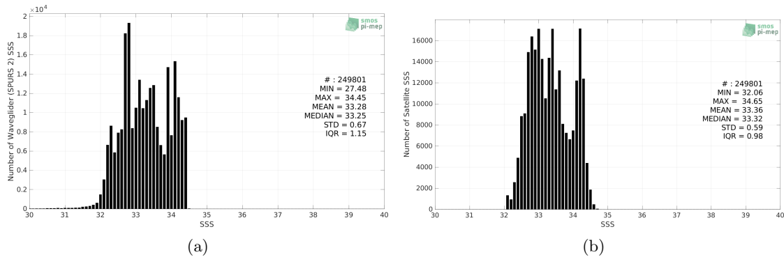
Figure 2: Histograms of SSS from Waveglider (SPURS 2) (a) and SMOS SSS L3 v332 - 9 Days (CATDS-CPDC) (b) considering all match-up pairs per bins of 0.1 over the SPURS 2 Pi-MEP region and for the full satellite product period.
