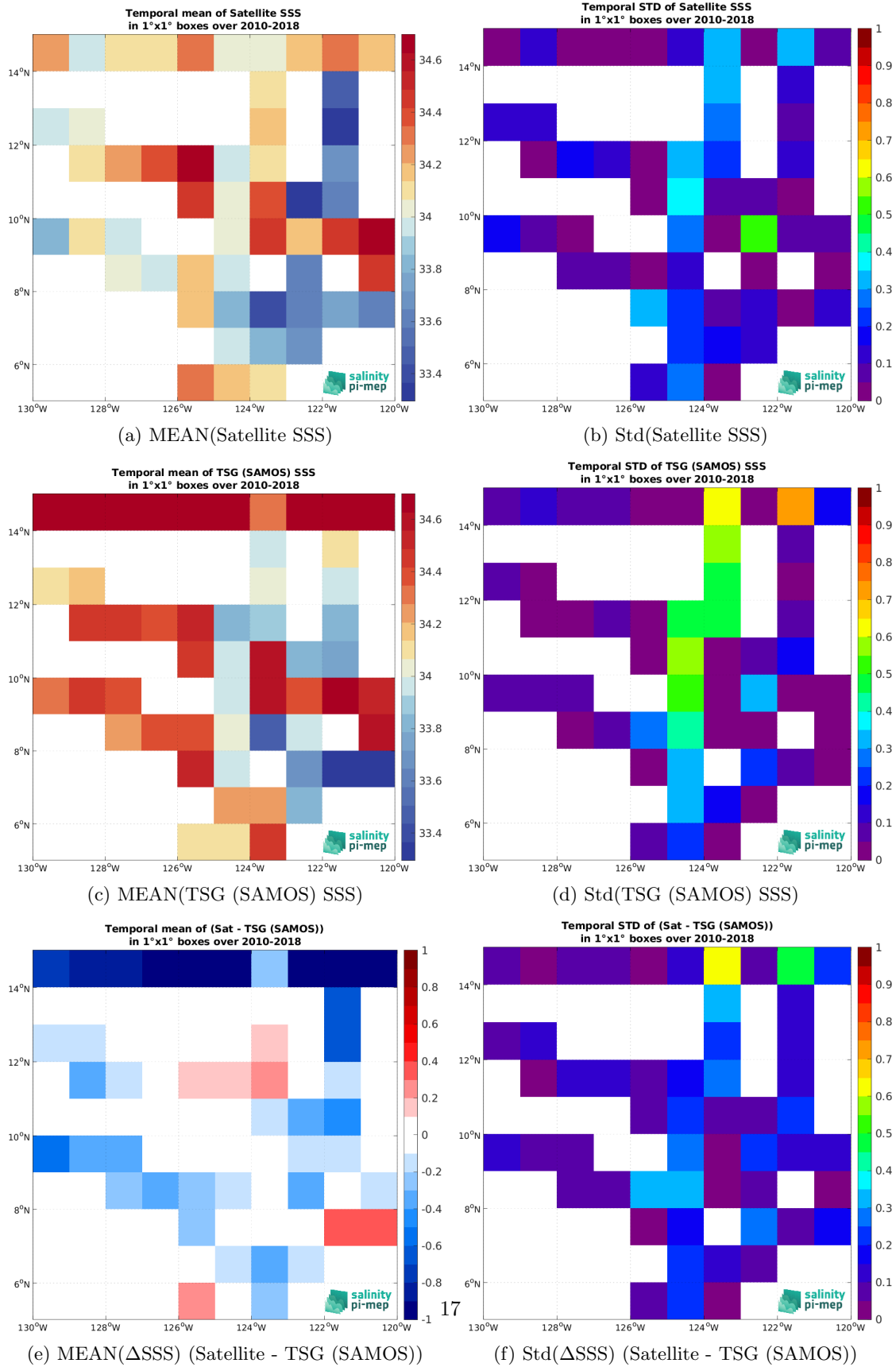
Figure 6: Temporal mean (left) and Std (right) of SSS from SMOS SSS L3 v332 - 9 Days (CATDS-CPDC) (top), TSG (SAMOS) (middle), and of \Delta SSS (Satellite - TSG (SAMOS)). Only match-up pairs are used to generate these maps.
