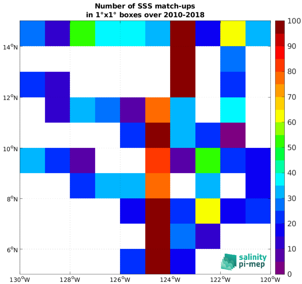
Figure 4: Number of SSS match-ups between TSG (SAMOS) SSS and the SMOS SSS L3 v332 - 9 Days (CATDS-CPDC) SSS product for the SPURS 2 Pi-MEP region over 1^\circ \times 1^\circ boxes and for the full satellite product period.
