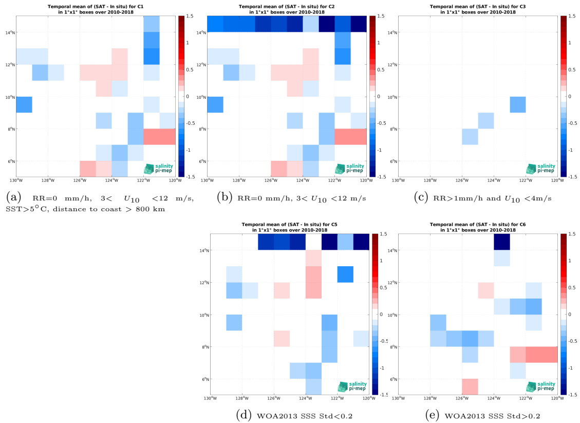
Figure 12: Temporal mean gridded over spatial boxes of size 1^\circ \times 1^\circ of \Delta\text{SSS} (SMOS SSS L3 v332 - 9 Days (CATDS-CPDC) - TSG (SAMOS)) for 5 different subdatasets corresponding to:RR=0 mm/h, 3 < U_{10} < 12 m/s, SST >5^\circ\text{C} , distance to coast > 800 km (a), RR=0 mm/h, 3 < U_{10} < 12 m/s (b), RR >1 mm/h and U_{10} < 4 m/s (c), WOA2013 SSS Std <0.2 (d), WOA2013 SSS Std >0.2 (e).
