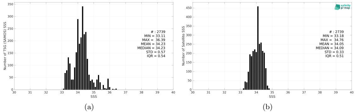
Figure 2: Histograms of SSS from TSG (SAMOS) (a) and SMOS SSS L3 v332 - 9 Days (CATDS-CPDC) (b) considering all match-up pairs per bins of 0.1 over the SPURS 2 Pi-MEP region and for the full satellite product period.
