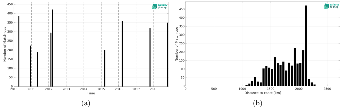
Figure 1: Number of match-ups between TSG (SAMOS) and SMOS SSS L3 v332 - 9 Days (CATDS-CPDC) SSS as a function of time (a) and as function of the distance to coast (b) over the SPURS 2 Pi-MEP region and for the full satellite product period.
