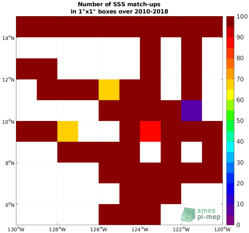
Figure 4: Number of SSS match-ups between TSG (SAMOS) SSS and the SMOS SSS L3 v332 - 9 Days (CATDS-CPDC) SSS product for the SPURS 2 Pi-MEP region over 1°x1° boxes and for the full satellite product period.
