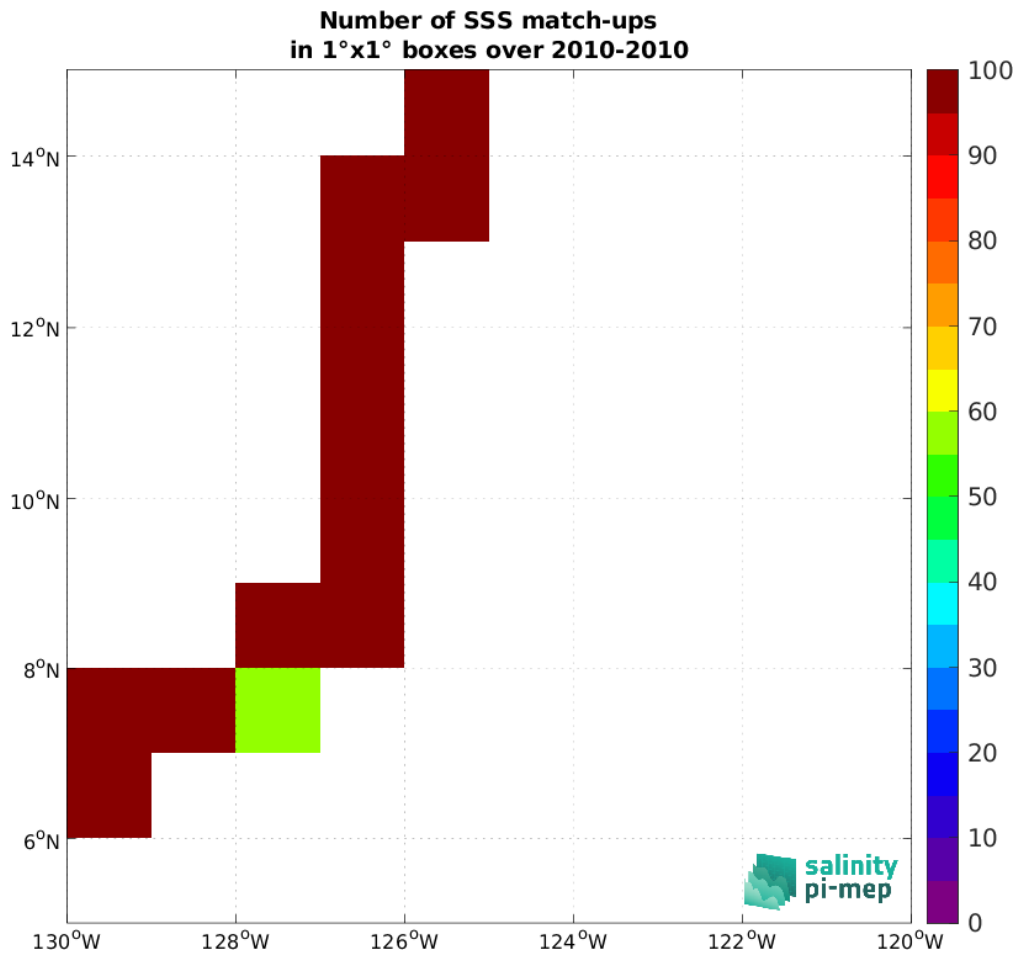
Figure 5: Number of SSS match-ups between TSG (GOSUD-Sailing-ship) SSS and the SMOS SSS L3 v332 - 9 Days (CATDS-CPDC) SSS product for the SPURS 2 Pi-MEP region over 1°x1° boxes and for the full satellite product period.
