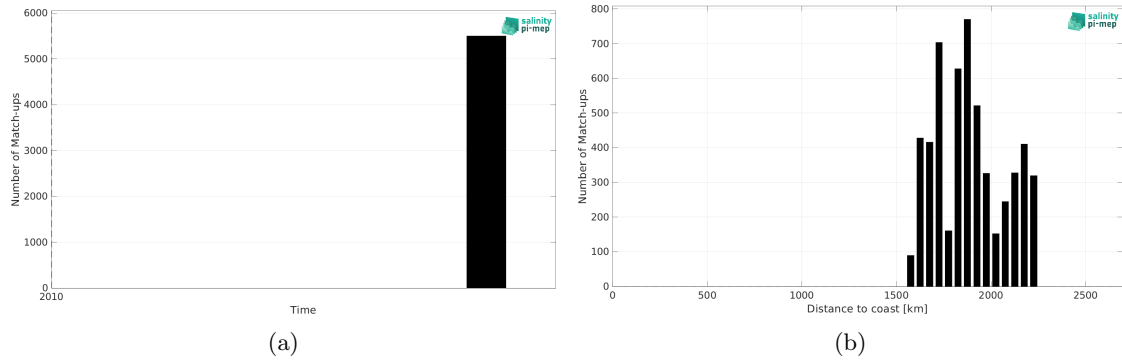
Figure 2: Number of match-ups between TSG (GOSUD-Sailing-ship) and SMOS SSS L3 v332 - 9 Days (CATDS-CPDC) SSS as a function of time (a) and as function of the distance to coast (b) over the SPURS 2 Pi-MEP region and for the full satellite product period.
