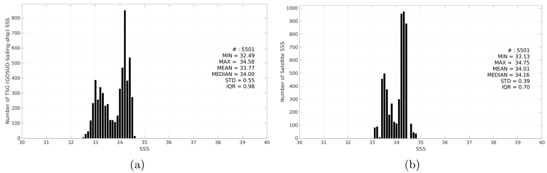
Figure 3: Histograms of SSS from TSG (GOSUD-Sailing-ship) (a) and SMOS SSS L3 v332 - 9 Days (CATDS-CPDC) (b) considering all match-up pairs per bins of 0.1 over the SPURS 2 Pi-MEP region and for the full satellite product period.
