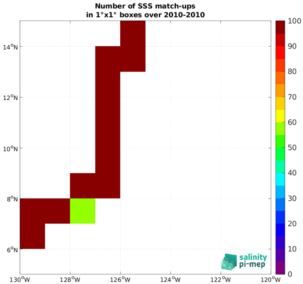
Figure 4: Number of SSS match-ups between TSG (GOSUD-Sailing-ship) SSS and the SMOS SSS L3 v332 - 9 Days (CATDS-CPDC) SSS product for the SPURS 2 Pi-MEP region over 1^{\circ} \times 1^{\circ} boxes and for the full satellite product period.
