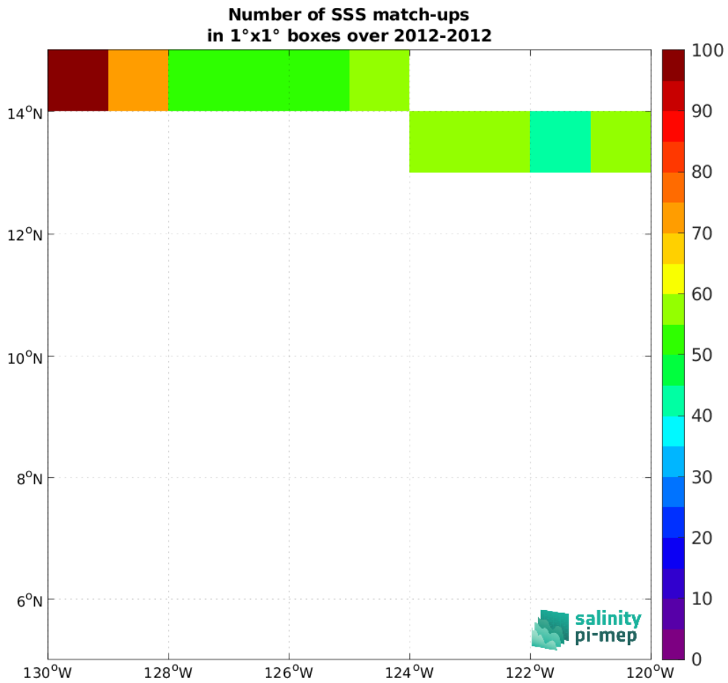
Figure 5: Number of SSS match-ups between TSG (GOSUD-Research-vessel) SSS and the SMOS SSS L3 v332 - 9 Days (CATDS-CPDC) SSS product for the SPURS 2 Pi-MEP region over 1°x1° boxes and for the full satellite product period.
