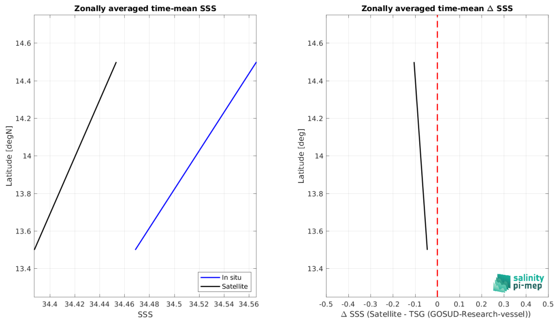
Figure 9: Left panel: Zonal mean SSS from SMOS SSS L3 v332 - 9 Days (CATDS-CPDC) satellite product (black) and from TSG (GOSUD-Research-vessel) (blue). Right panel: Zonal mean of \Delta SSS (Satellite - TSG (GOSUD-Research-vessel)) for all the collected Pi-MEP match-up pairs estimated over the full satellite product period.
