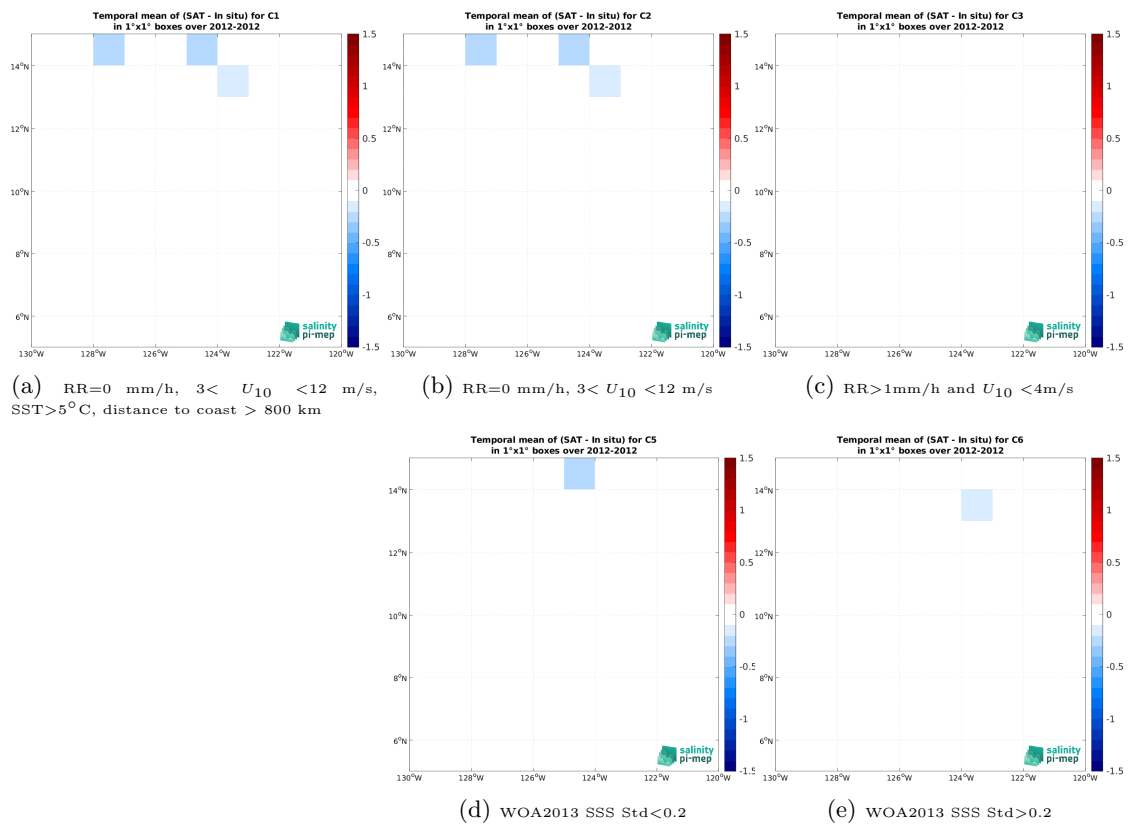
Figure 14: Temporal mean gridded over spatial boxes of size 1^\circ \times 1^\circ of \Delta\text{SSS} (SMOS SSS L3 v332 - 9 Days (CATDS-CPDC) - TSG (GOSUD-Research-vessel)) for 5 different subdatasets corresponding to:RR=0 mm/h, 3 < U_{10} < 12 m/s, SST>5°C, distance to coast > 800 km (a), RR=0 mm/h, 3 < U_{10} < 12 m/s (b), RR>1mm/h and U_{10} < 4 m/s (c), WOA2013 SSS Std<0.2 (d), WOA2013 SSS Std>0.2 (e).
