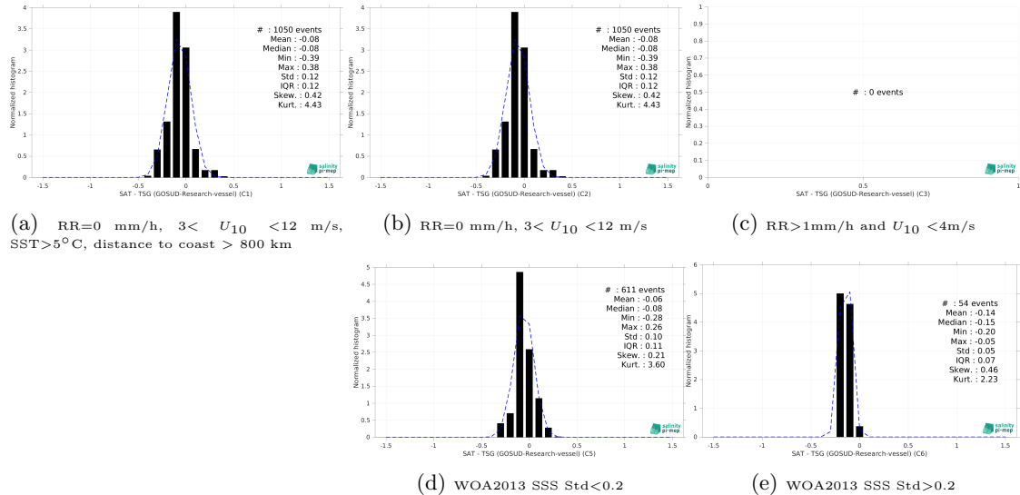
Figure 15: Normalized histogram of \Delta SSS (SMOS SSS L3 v332 - 9 Days (CATDS-CPDC) - TSG (GOSUD-Research-vessel)) for 5 different subdatasets corresponding to: RR=0 mm/h, 3 < U_{10} < 12 m/s, SST>5°C, distance to coast > 800 km (a), RR=0 mm/h, 3 < U_{10} < 12 m/s (b), RR>1mm/h and U_{10} < 4 m/s (c), WOA2013 SSS Std<0.2 (d), WOA2013 SSS Std>0.2 (e).
