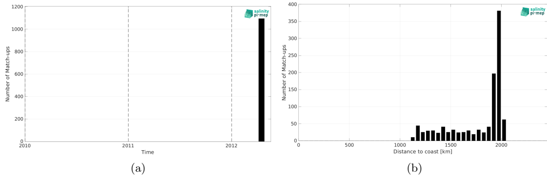
Figure 2: Number of match-ups between TSG (GOSUD-Research-vessel) and SMOS SSS L3 v332 - 9 Days (CATDS-CPDC) SSS as a function of time (a) and as function of the distance to coast (b) over the SPURS 2 Pi-MEP region and for the full satellite product period.
