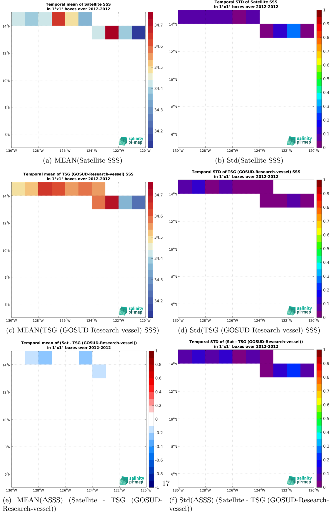
Figure 7: Temporal mean (left) and Std (right) of SSS from SMOS SSS L3 v332 - 9 Days (CATDS-CPDC) (top), TSG (GOSUD-Research-vessel) (middle), and of \Delta SSS (Satellite - TSG (GOSUD-Research-vessel)). Only match-up pairs are used to generate these maps.
