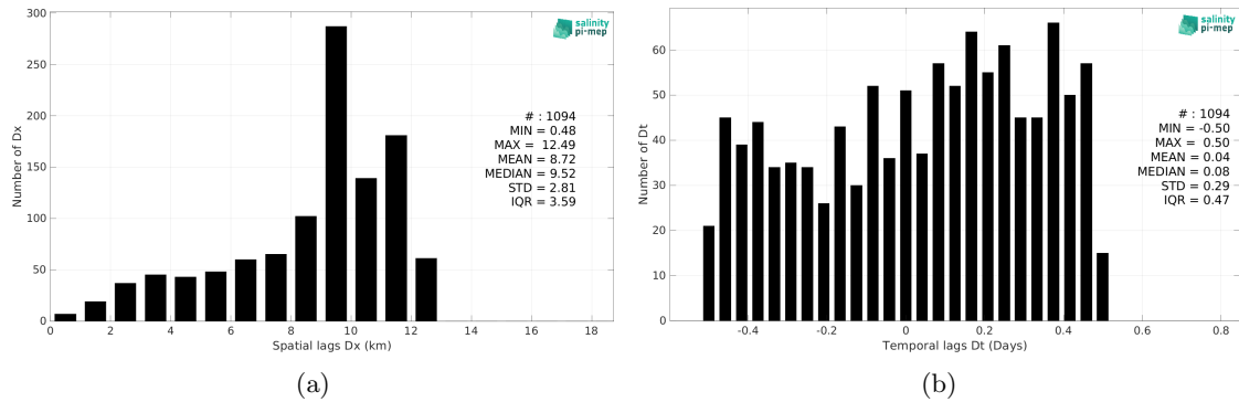
Figure 6: Histograms of the spatial (a) and temporal (b) lags between the location/time of the TSG (GOSUD-Research-vessel) measurement and the date of the corresponding SMOS SSS L3 v332 - 9 Days (CATDS-CPDC) SSS pixel.
