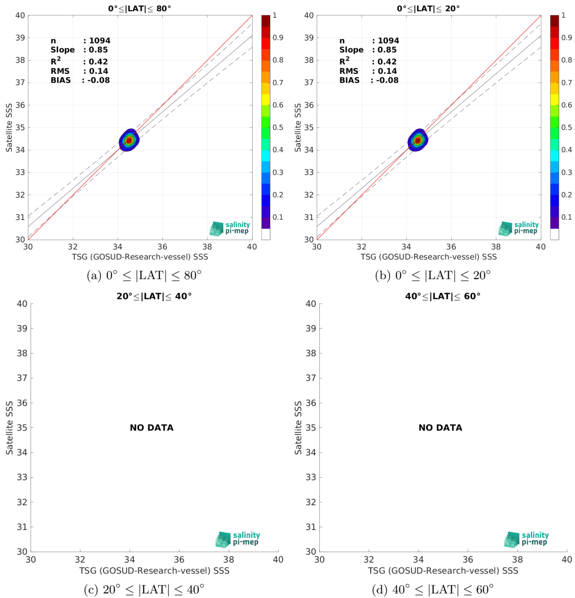
Figure 10: Contour maps of the concentration of SMOS SSS L3 v332 - 9 Days (CATDS-CPDC) SSS (y-axis) versus TSG (GOSUD-Research-vessel) SSS (x-axis) at match-up pairs for different latitude bands. For each plot, the red line shows x=y . The black thin and dashed lines indicate a linear fit through the data cloud and the \pm 95\% confidence levels, respectively. The number match-up pairs n , the slope and R^2 coefficient of the linear fit, the root mean square (RMS) and the mean bias between satellite and in situ data are indicated for each latitude band in each plots.
