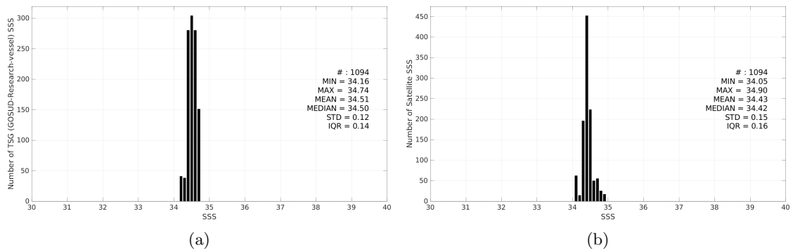
Figure 3: Histograms of SSS from TSG (GOSUD-Research-vessel) (a) and SMOS SSS L3 v332 - 9 Days (CATDS-CPDC) (b) considering all match-up pairs per bins of 0.1 over the SPURS 2 Pi-MEP region and for the full satellite product period.
