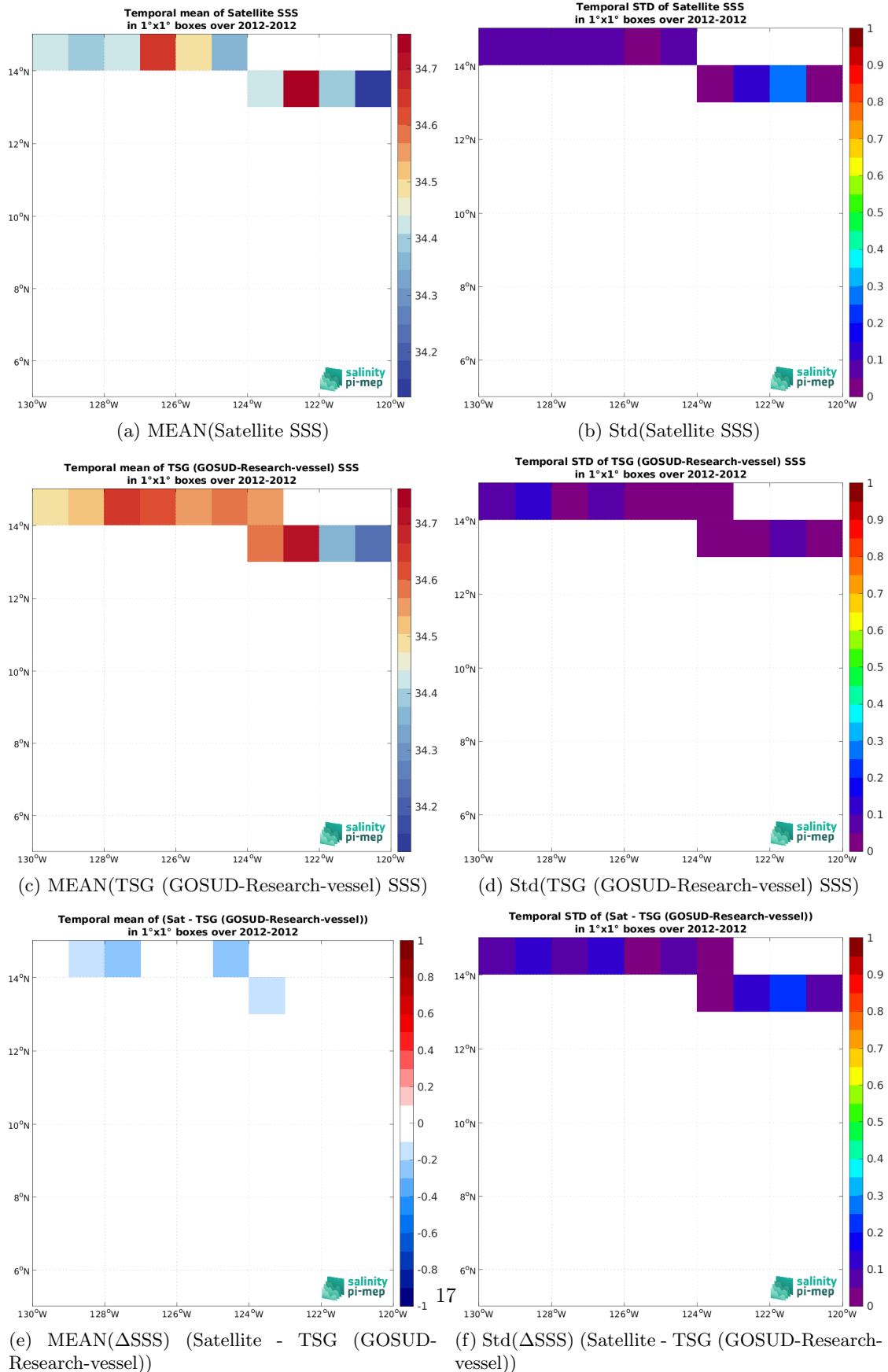
Figure 6: Temporal mean (left) and Std (right) of SSS from SMOS SSS L3 v332 - 9 Days (CATDS-CPDC) (top), TSG (GOSUD-Research-vessel) (middle), and of \Delta SSS (Satellite - TSG (GOSUD-Research-vessel)). Only match-up pairs are used to generate these maps.
