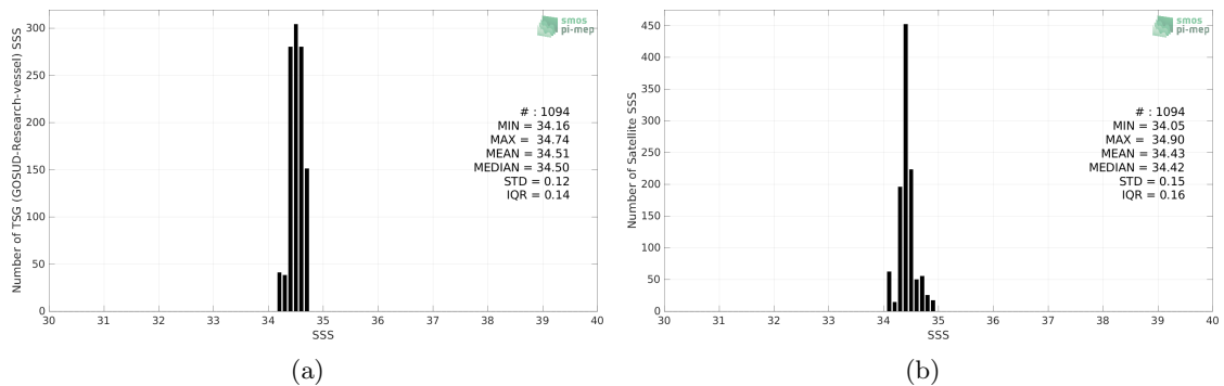
Figure 2: Histograms of SSS from TSG (GOSUD-Research-vessel) (a) and SMOS SSS L3 v332 - 9 Days (CATDS-CPDC) (b) considering all match-up pairs per bins of 0.1 over the SPURS 2 Pi-MEP region and for the full satellite product period.
