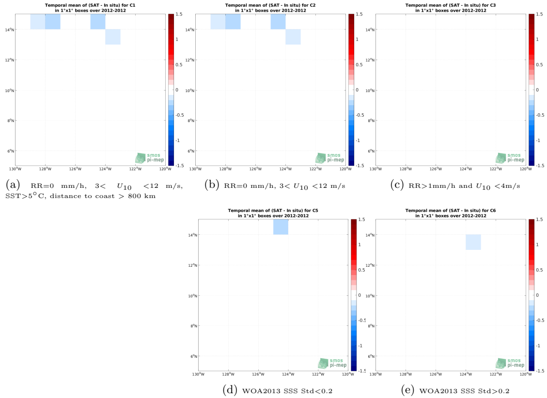
Figure 12: Temporal mean gridded over spatial boxes of size 1^{\circ} \times 1^{\circ} of \Delta\text{SSS} (SMOS SSS L3 v332 - 9 Days (CATDS-CPDC) - TSG (GOSUD-Research-vessel)) for 5 different subdatasets corresponding to: RR=0 mm/h, 3 < U_{10} < 12 m/s, SST > 5^{\circ}\text{C} , distance to coast > 800 km (a), RR=0 mm/h, 3 < U_{10} < 12 m/s (b), RR > 1\text{mm/h} and U_{10} < 4\text{m/s} (c), WOA2013 SSS Std < 0.2 (d), WOA2013 SSS Std > 0.2 (e).
