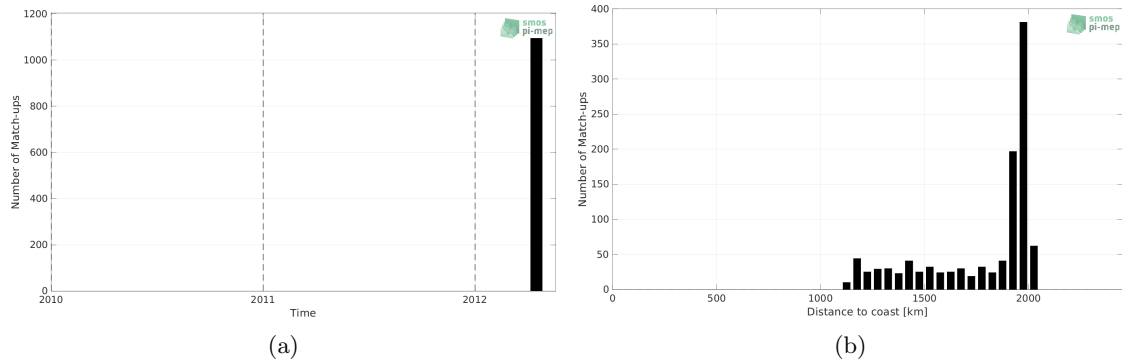
Figure 1: Number of match-ups between TSG (GOSUD-Research-vessel) and SMOS SSS L3 v332 - 9 Days (CATDS-CPDC) SSS as a function of time (a) and as function of the distance to coast (b) over the SPURS 2 Pi-MEP region and for the full satellite product period.
