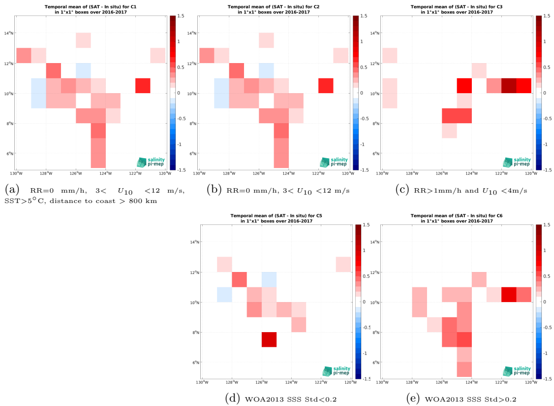
Figure 14: Temporal mean gridded over spatial boxes of size 1^\circ \times 1^\circ of \Delta\text{SSS} (SMOS SSS L3 v332 - 9 Days (CATDS-CPDC) - Salinity Snake (SPURS 2)) for 5 different subdatasets corresponding to: RR=0 mm/h, 3 < U_{10} < 12 m/s, SST > 5°C, distance to coast > 800 km (a), RR=0 mm/h, 3 < U_{10} < 12 m/s (b), RR > 1mm/h and U_{10} < 4 m/s (c), WOA2013 SSS Std < 0.2 (d), WOA2013 SSS Std > 0.2 (e).
