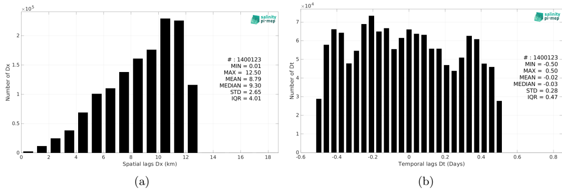
Figure 6: Histograms of the spatial (a) and temporal (b) lags between the location/time of the Salinity Snake (SPURS 2) measurement and the date of the corresponding SMOS SSS L3 v332 - 9 Days (CATDS-CPDC) SSS pixel.
