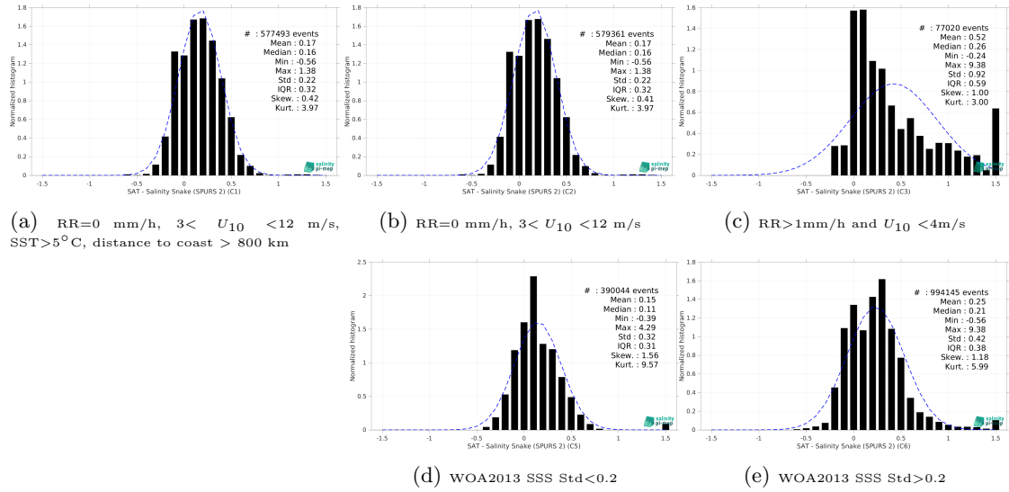
Figure 15: Normalized histogram of \Delta SSS (SMOS SSS L3 v332 - 9 Days (CATDS-CPDC) - Salinity Snake (SPURS 2)) for 5 different subdatasets corresponding to: RR=0 mm/h, 3 < U_{10} < 12 m/s, SST>5°C, distance to coast > 800 km (a), RR=0 mm/h, 3 < U_{10} < 12 m/s (b), RR>1mm/h and U_{10} < 4 m/s (c), WOA2013 SSS Std<0.2 (d), WOA2013 SSS Std>0.2 (e).
