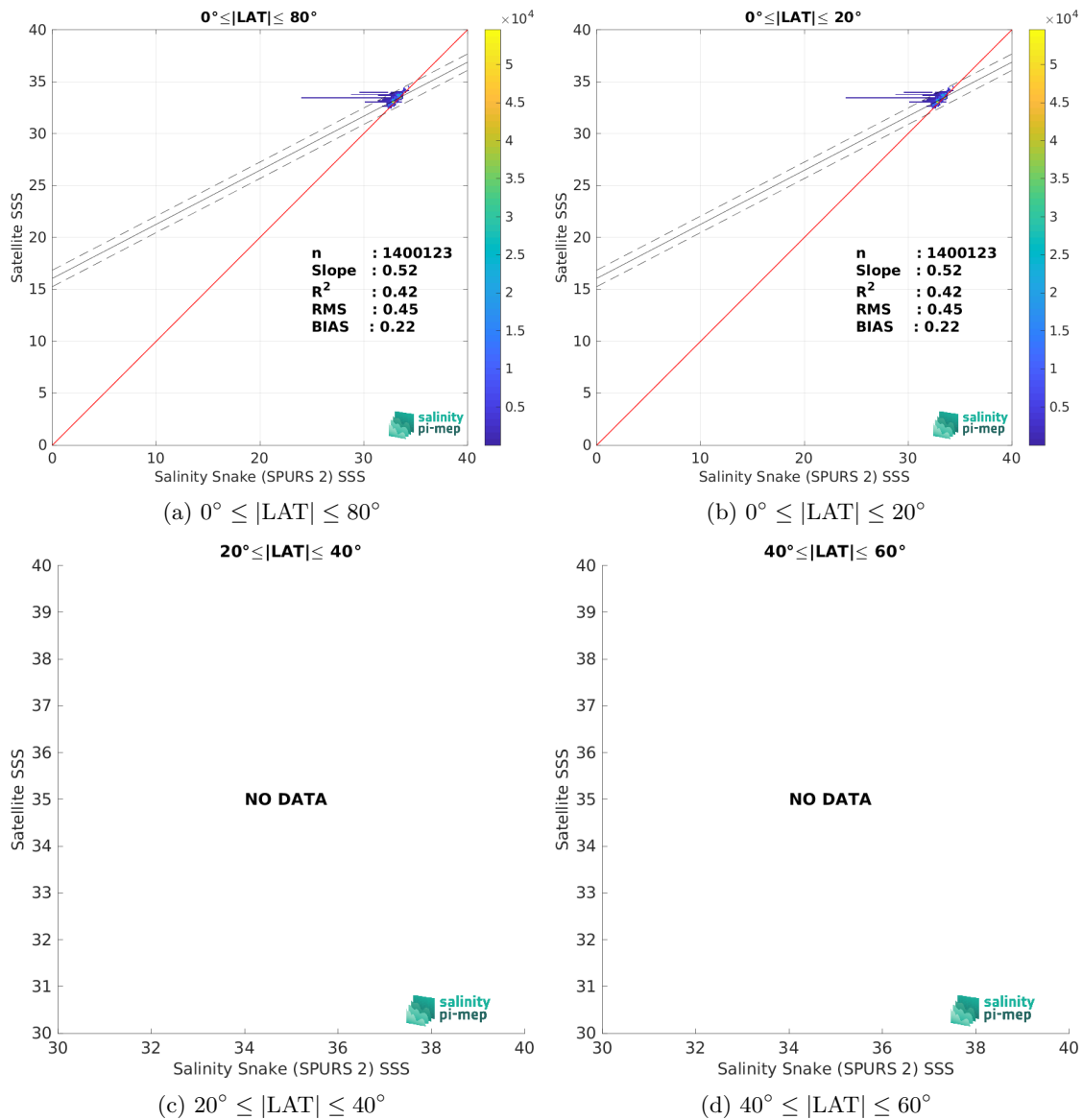
Figure 10: Contour maps of the concentration of SMOS SSS L3 v332 - 9 Days (CATDS-CPDC) SSS (y-axis) versus Salinity Snake (SPURS 2) SSS (x-axis) at match-up pairs for different latitude bands. For each plot, the red line shows x=y . The black thin and dashed lines indicate a linear fit through the data cloud and the \pm 95\% confidence levels, respectively. The number match-up pairs n , the slope and R^2 coefficient of the linear fit, the root mean square (RMS) and the mean bias between satellite and in situ data are indicated for each latitude band in each plots.
