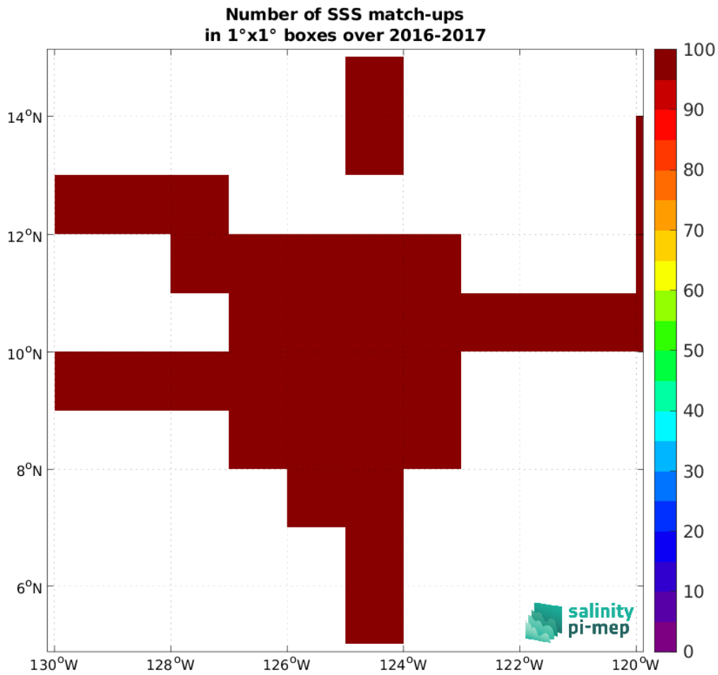
Figure 5: Number of SSS match-ups between Salinity Snake (SPURS 2) SSS and the SMOS SSS L3 v332 - 9 Days (CATDS-CPDC) SSS product for the SPURS 2 Pi-MEP region over 1°x1° boxes and for the full satellite product period.
