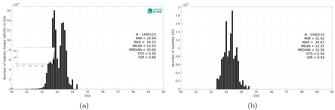
Figure 3: Histograms of SSS from Salinity Snake (SPURS 2) (a) and SMOS SSS L3 v332 - 9 Days (CATDS-CPDC) (b) considering all match-up pairs per bins of 0.1 over the SPURS 2 Pi-MEP region and for the full satellite product period.
