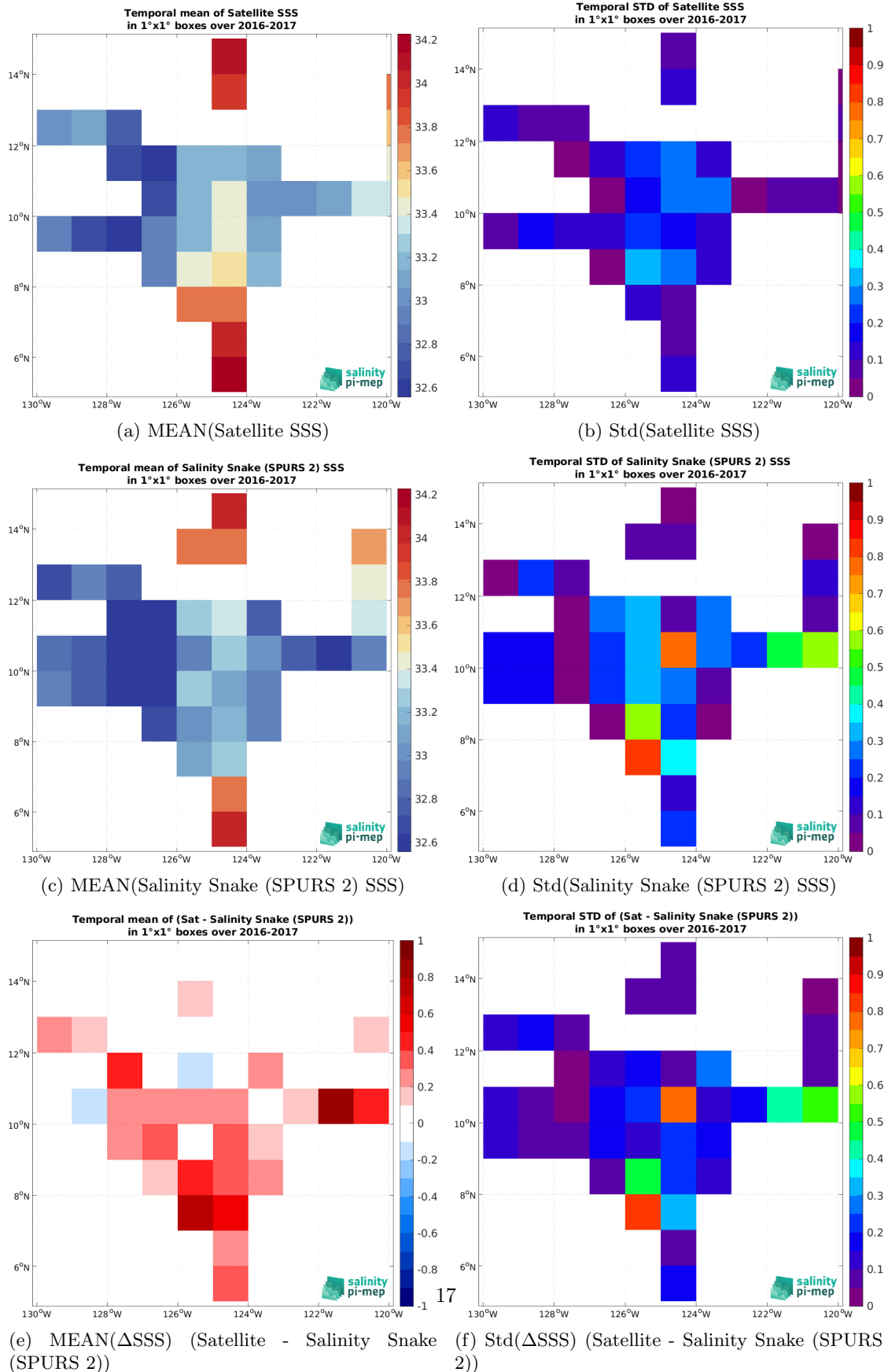
Figure 7: Temporal mean (left) and Std (right) of SSS from SMOS SSS L3 v332 - 9 Days (CATDS-CPDC) (top), Salinity Snake (SPURS 2) (middle), and of \Delta SSS (Satellite - Salinity Snake (SPURS 2)). Only match-up pairs are used to generate these maps.
