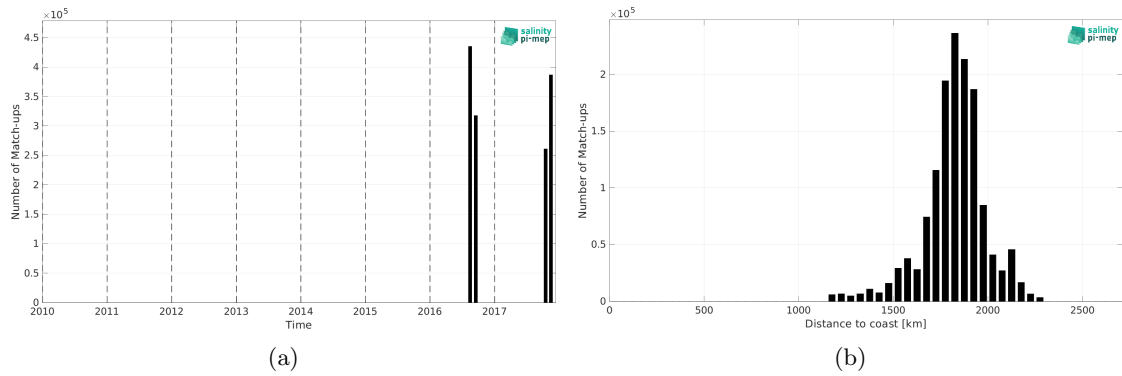
Figure 2: Number of match-ups between Salinity Snake (SPURS 2) and SMOS SSS L3 v332 - 9 Days (CATDS-CPDC) SSS as a function of time (a) and as function of the distance to coast (b) over the SPURS 2 Pi-MEP region and for the full satellite product period.
