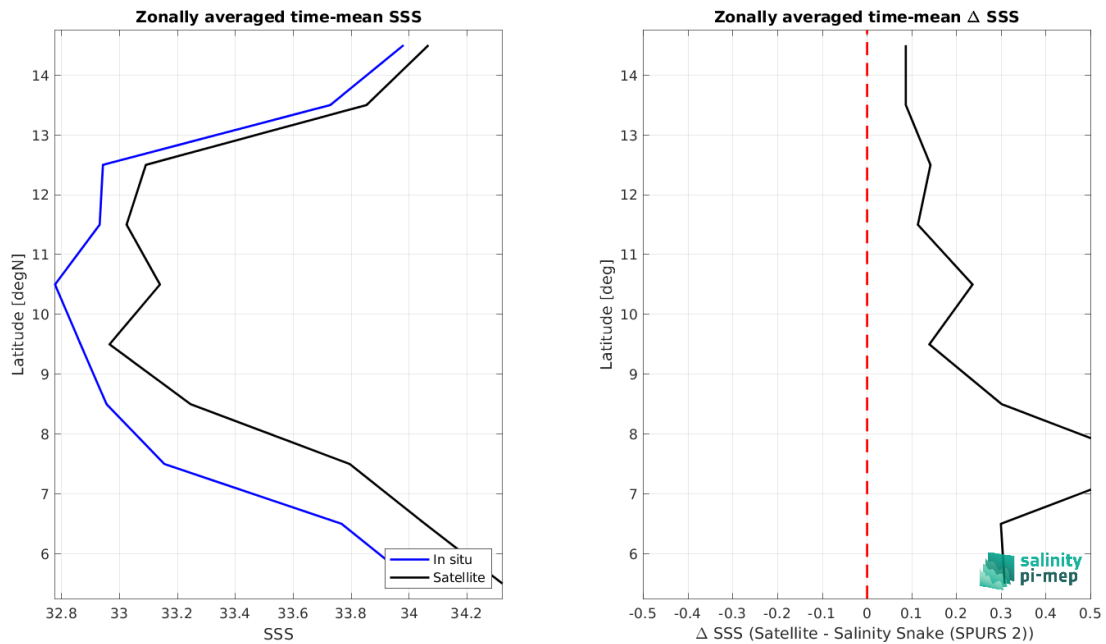
Figure 9: Left panel: Zonal mean SSS from SMOS SSS L3 v332 - 9 Days (CATDS-CPDC) satellite product (black) and from Salinity Snake (SPURS 2) (blue). Right panel: Zonal mean of \Delta SSS (Satellite - Salinity Snake (SPURS 2)) for all the collected Pi-MEP match-up pairs estimated over the full satellite product period.
